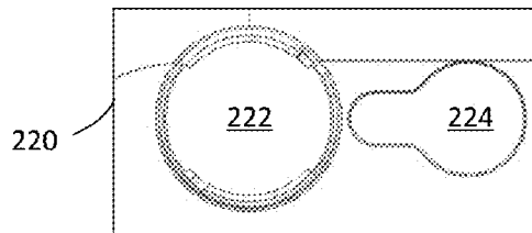
Top view of bayonet interface (phone side)
