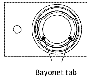
Bottom view of bayonet interface (lens)
