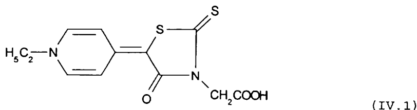
5-(1-ethyl-4(1H)-pyridyl)-4-oxo-2-thioxo-3-thiazolidine acetic acid
