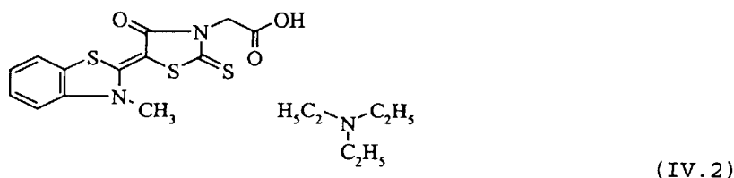
5-(3-methyl-3(3H)-benzothiazolylidene)-4-oxo-2-thioxo-3-thiazolidine acetic acid
