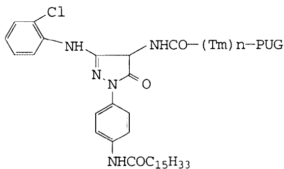
Compound No. 36A-No. 40A
