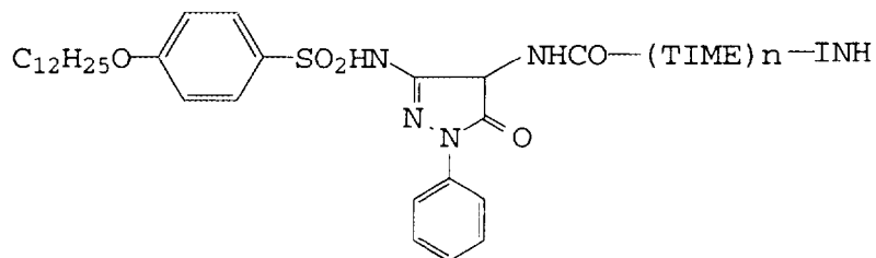
Compound No. 11B-No. 20B
