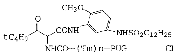
Compound No. 1A-No. 5A
