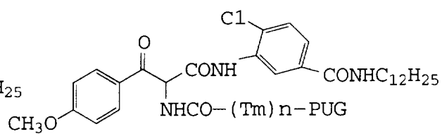
Compound No. 6A-No. 10A
