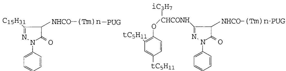
Compound No. 16A-No. 25A
