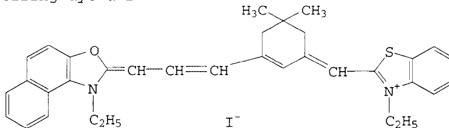
Sensitizing dye d-2
