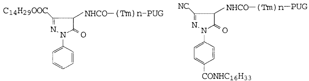
Compound No. 31A-No. 35A
