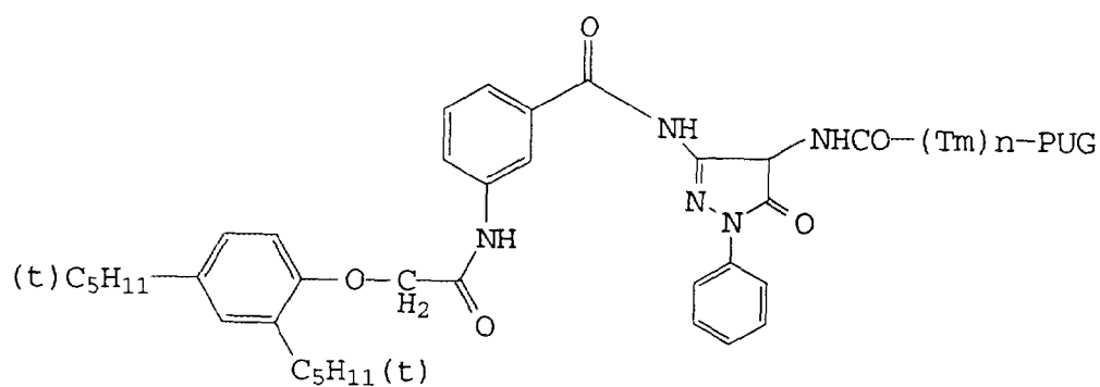
Compound No. 41A-No. 45A
