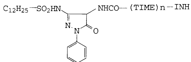
Compound No. 31B-No. 35B
