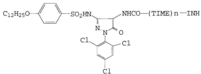
Compound No. 26B-No. 30B
