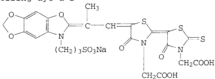
Sensitizing dye d-1
