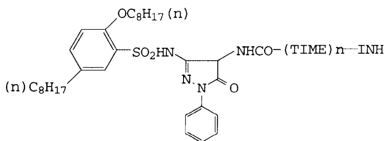
Compound No. 1B-No. 10B
