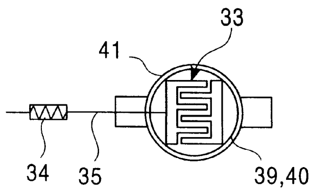
FIG. 11 PRIOR ART
