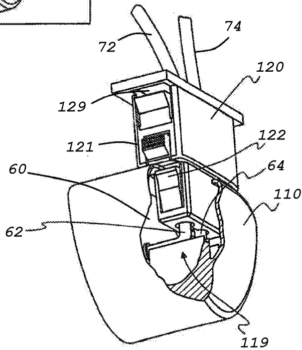
FIG. 7 (Prior Art)
