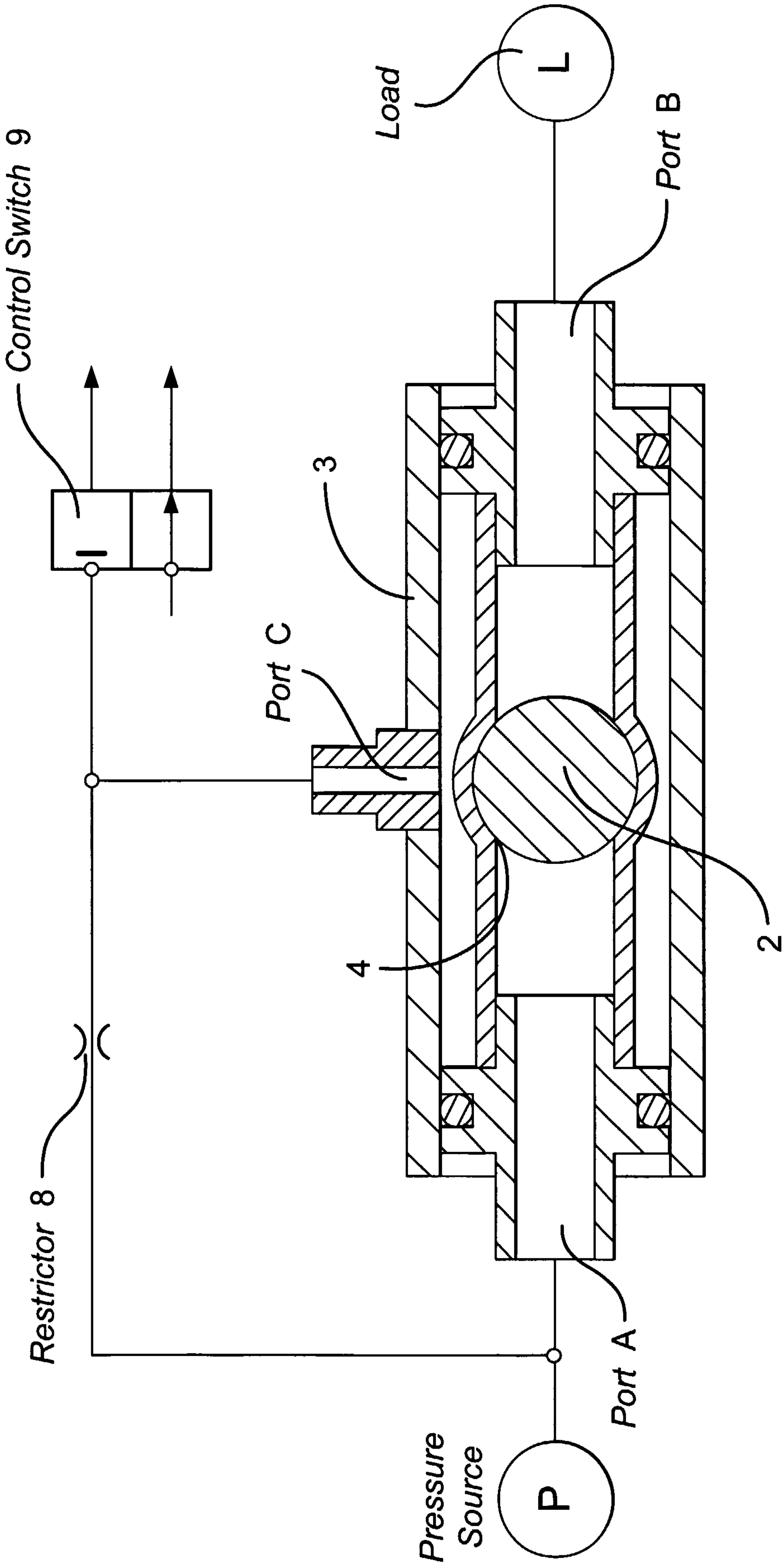
Fig.4 Valve in simplified switching mode.
