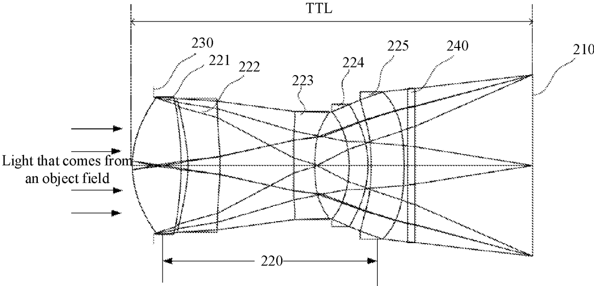
Image photographing apparatus 20
