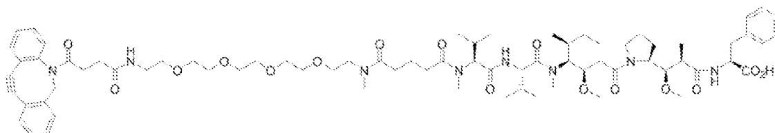
Figure 11B: DBCO-DM4
