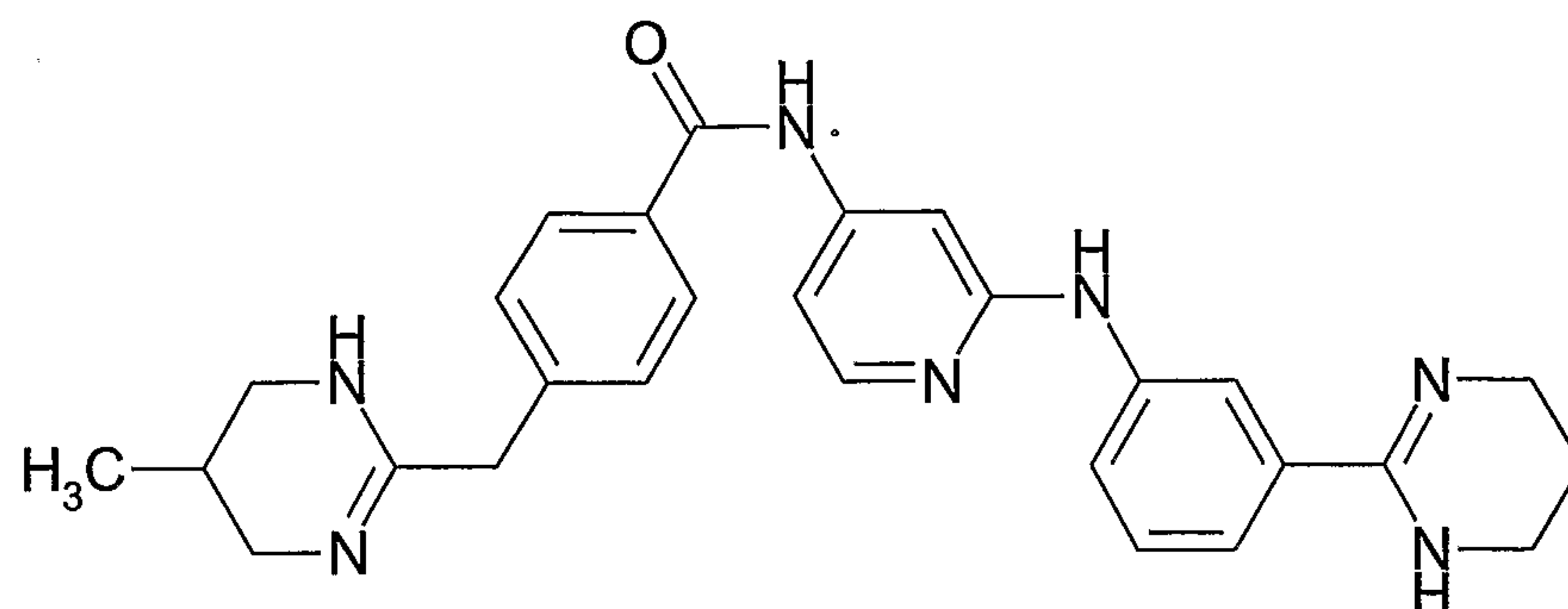
Formula II
