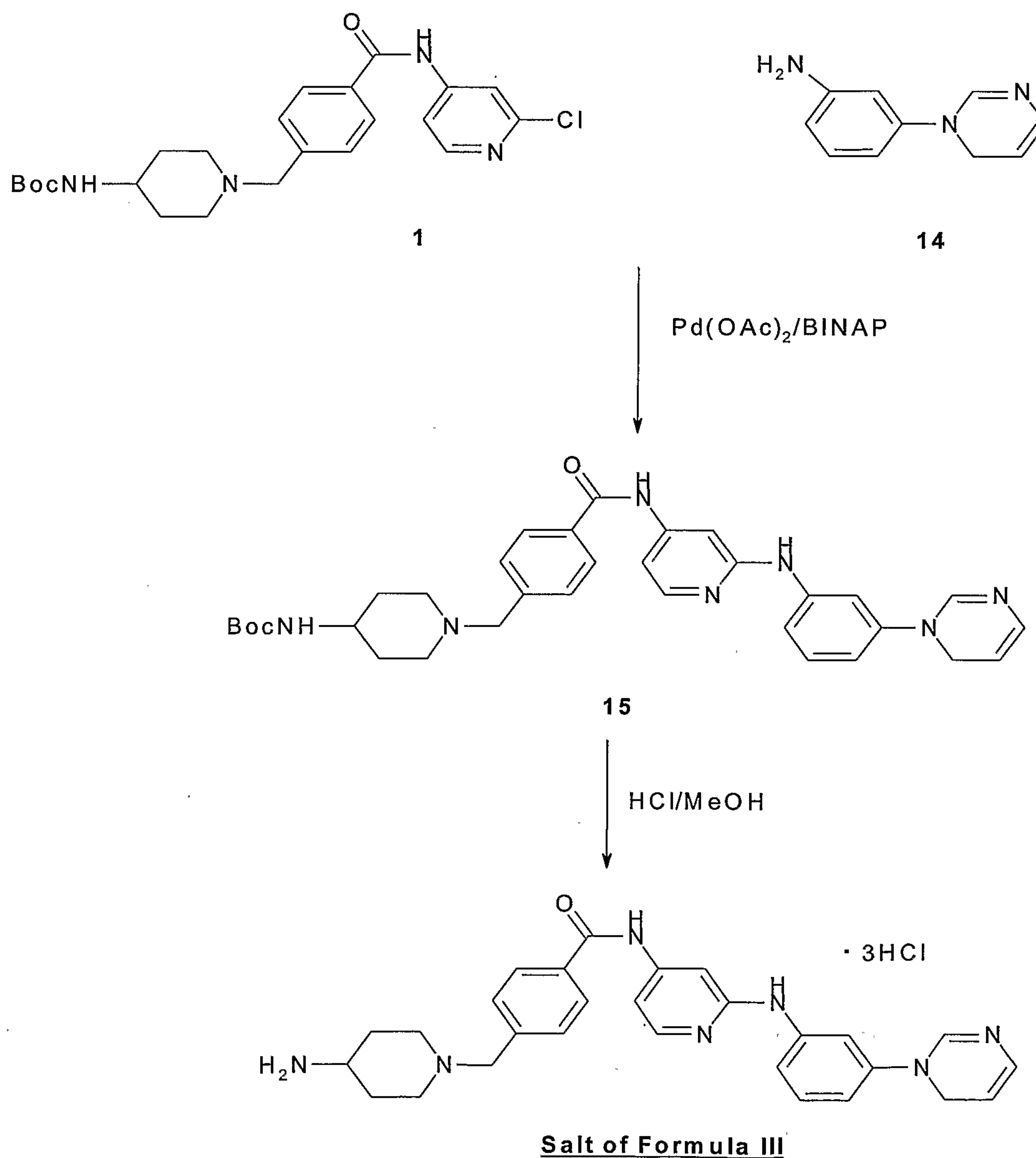
Scheme 4
