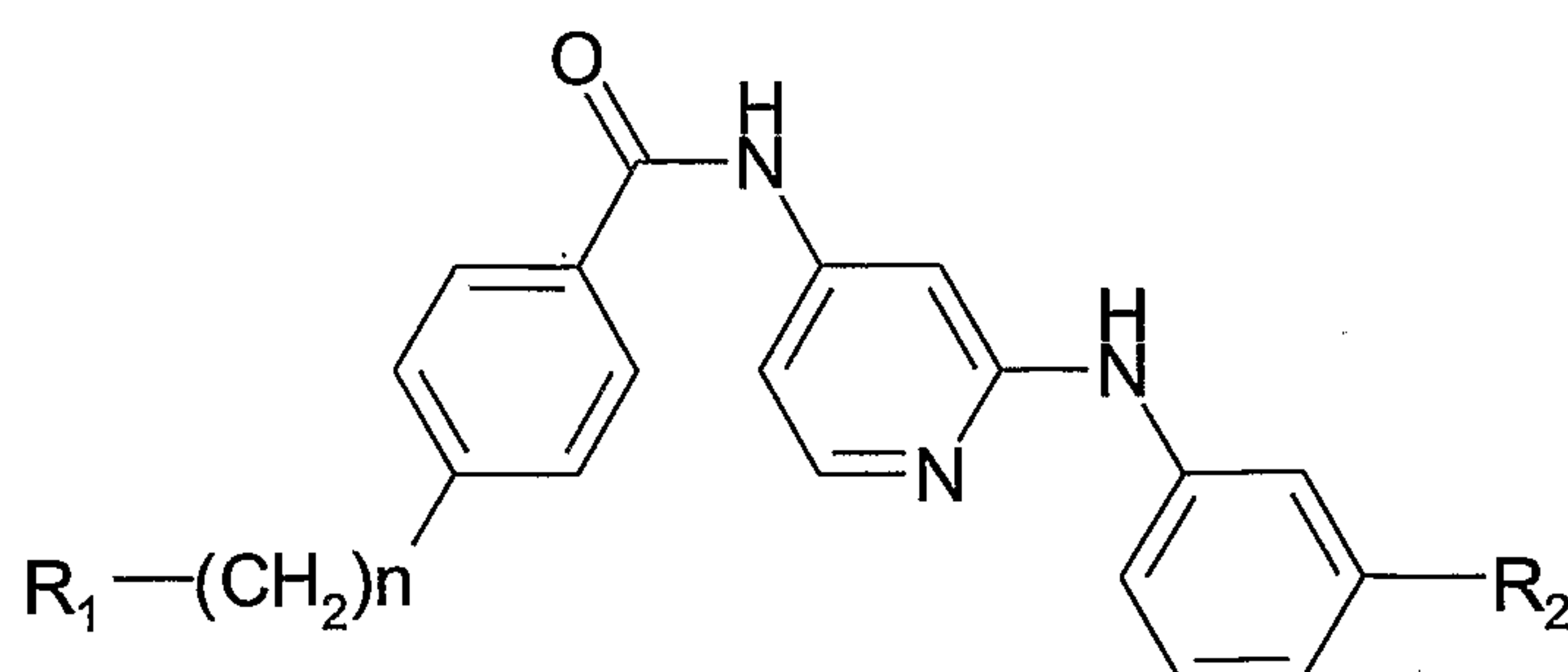
Formula I
