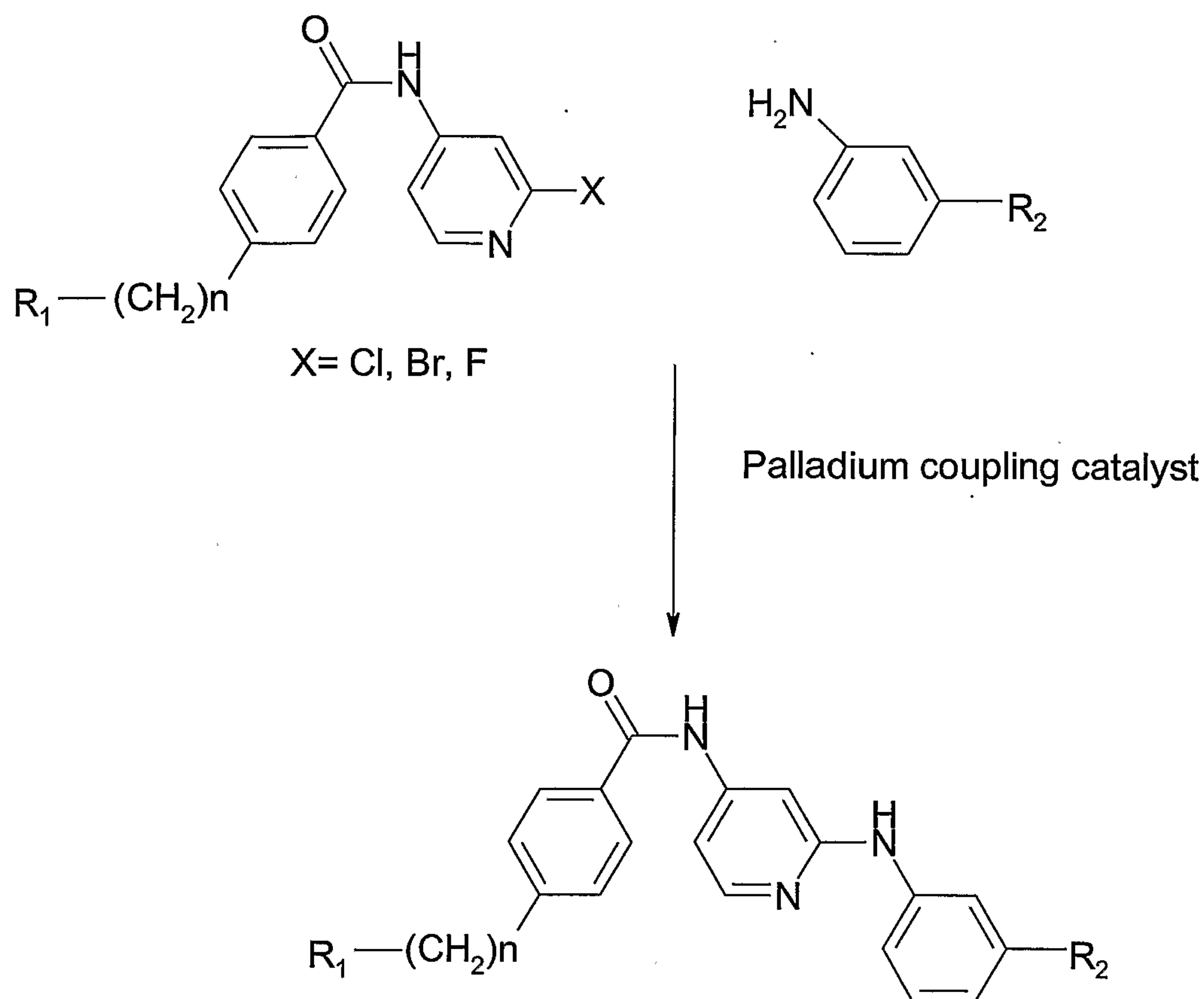
Formula I
