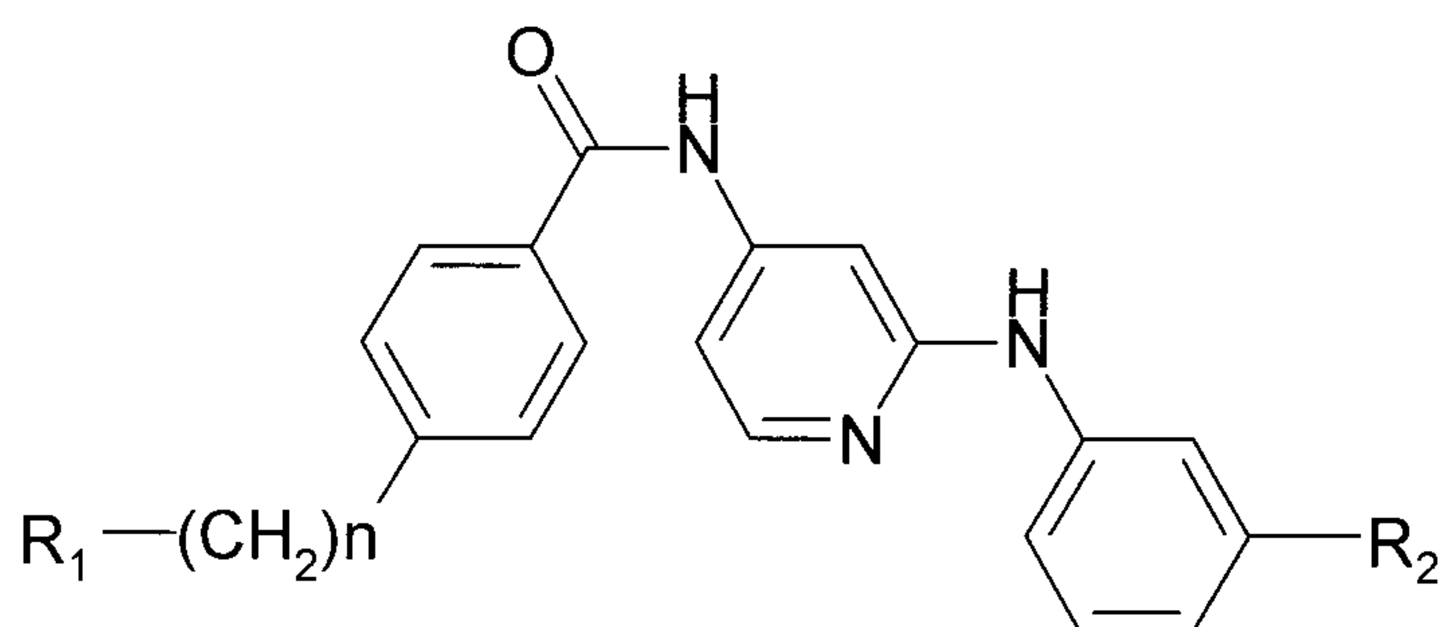
Formula I
