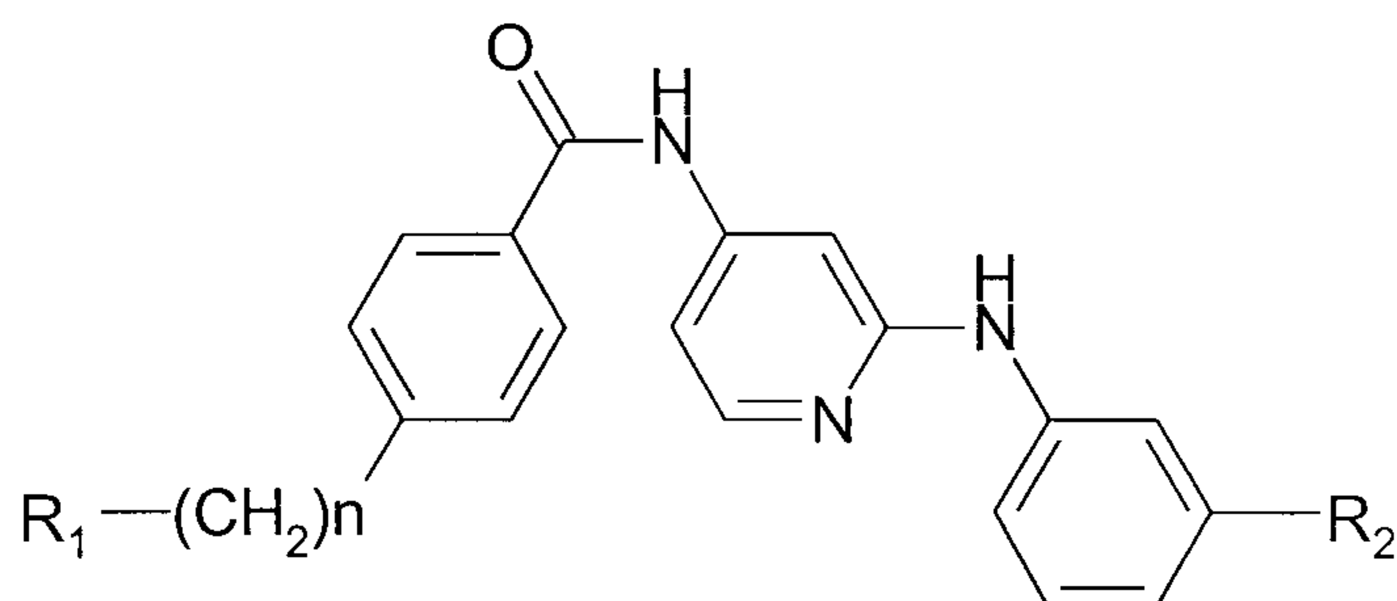
Formula I
