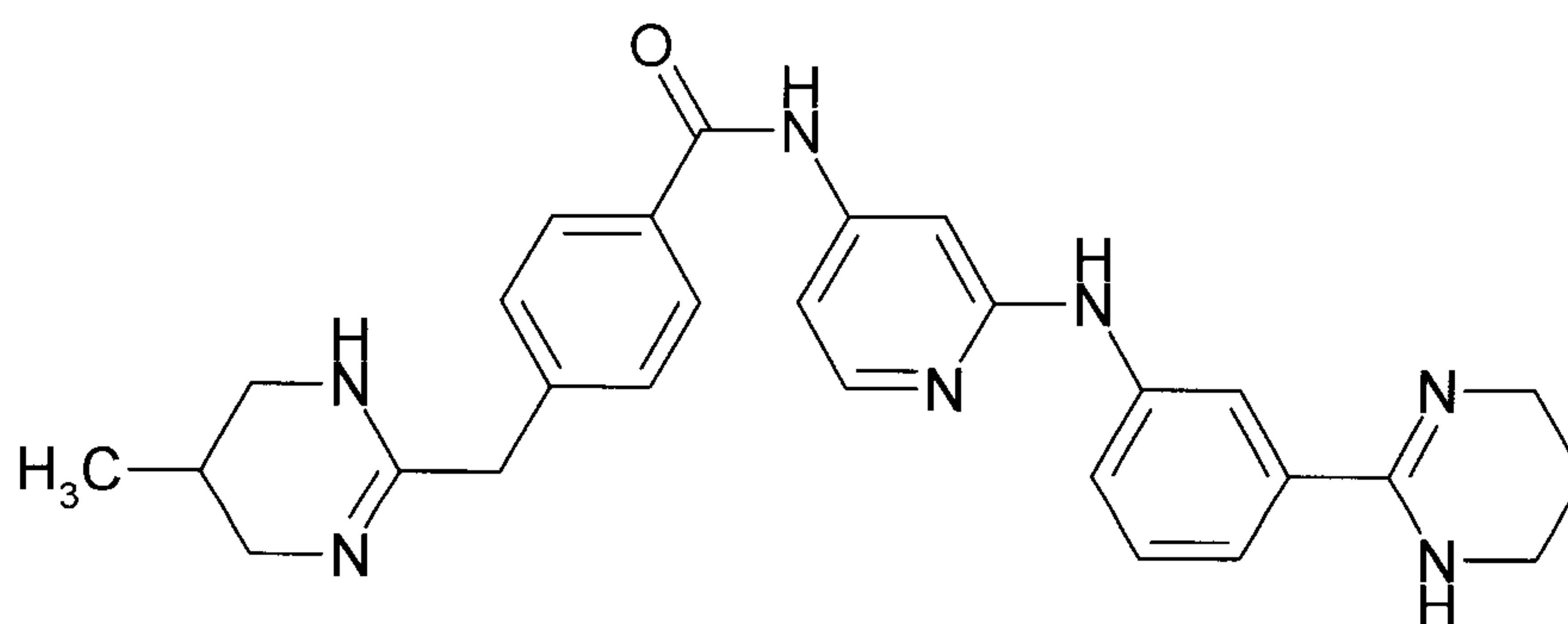
Formula II
