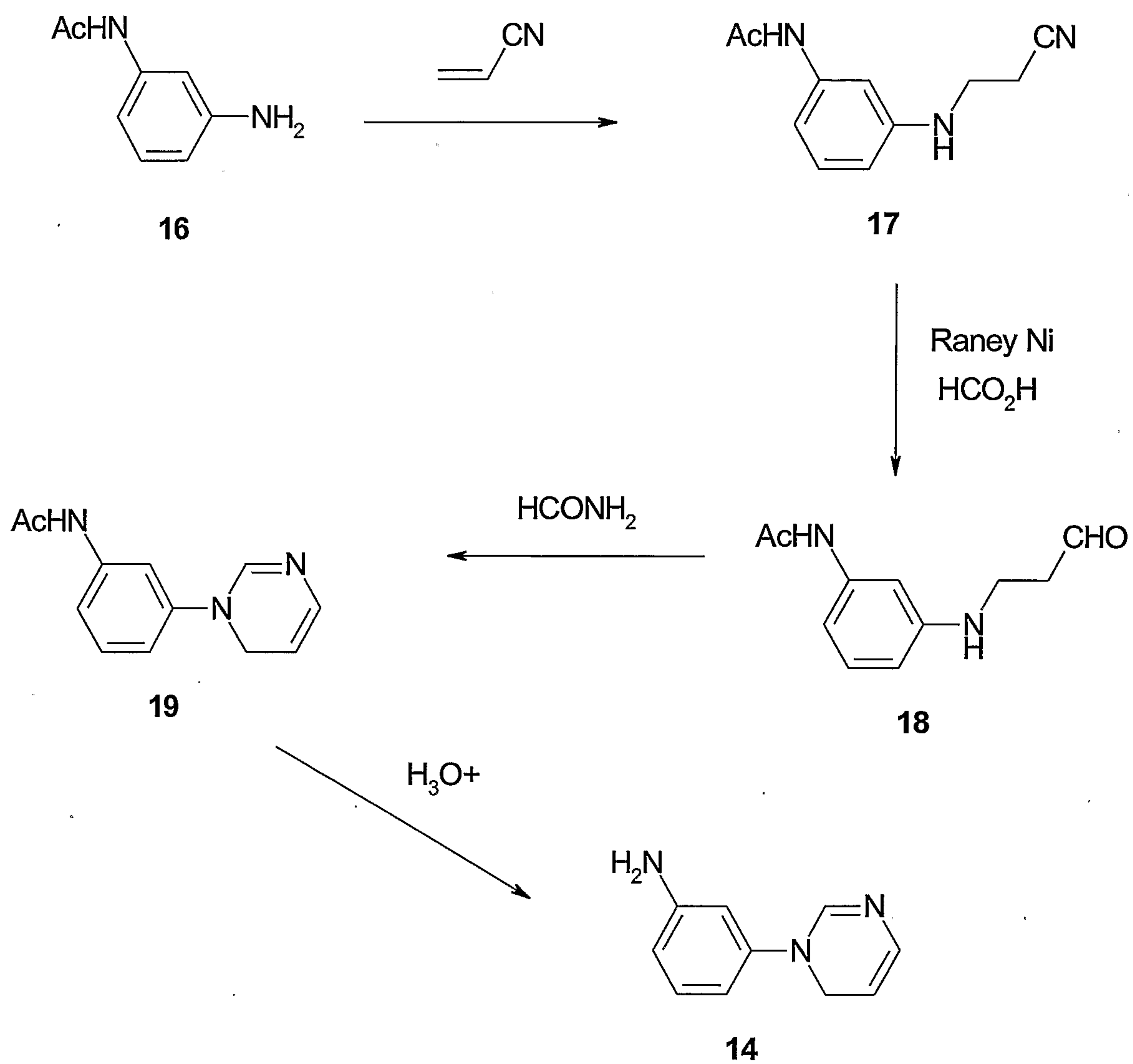
Scheme 5
