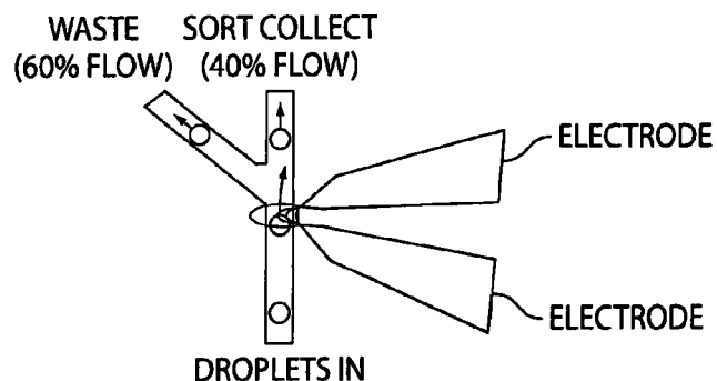
FLIPPED FLUIDIC GEOMETRY (ASYMMETRIC FLOW GEOMETRY)
