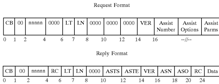
FIG. X3 - SETIPXASSTPARMS Reply and Request Command Format
