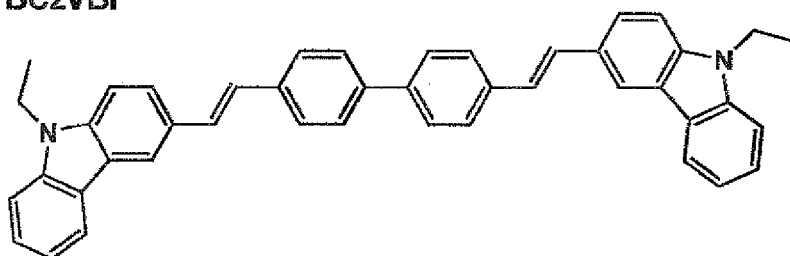
BCzVBi
