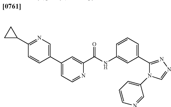
6-cyclopropyl-N-(3-(4-(pyridin-2-yl)-4H-1,2,4-triazol-3-yl)phenyl)-3,4'-bipyridine-2'-carboxamide
