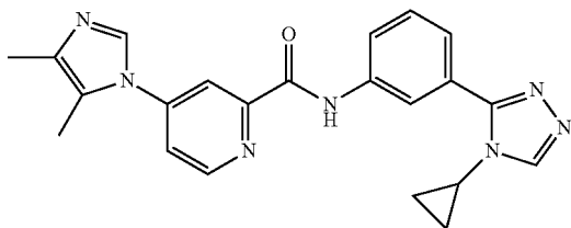
N-(3-(4-cyclopropyl-4H-1,2,4-triazol-3-yl)phenyl)- 4-(4,5-dimethyl-1H-imidazol-1-yl)picolinamide
