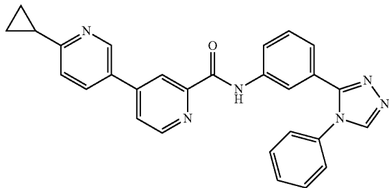
6-cyclopropyl-N-(3-(4-phenyl-4H-1,2,4-triazol-3-yl)phenyl)-3,4'-bipyridine-2'-carboxamide
