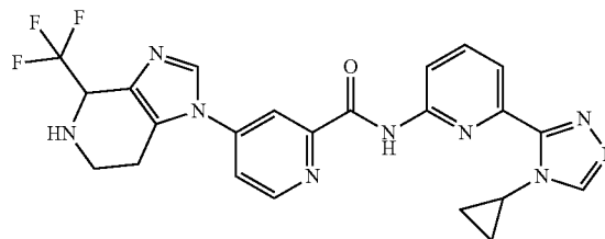
N-(6-(4-cyclopropyl-4H-1,2,4-triazol-3-yl)pyridin-2-yl)-4-(4-(trifluoromethyl)-4,5,6,7-tetrahydro-1H-imidazo[4,5-c]pyridin-1-yl)picolinamide
