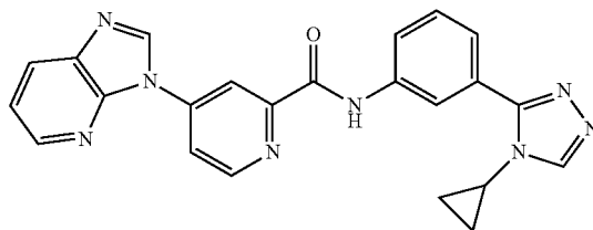
N-(3-(4-cyclopropyl-4H-1,2,4-triazol-3-yl)phenyl)- 4-(3H-imidazo[4,5-b]pyridin-3-yl)picolinamide
