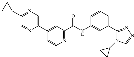
N-(3-(4-cyclopropyl-4H-1,2,4-triazol-3-yl)phenyl)-4-(5-cyclopropylpyrazin-2-yl)picolinamide
