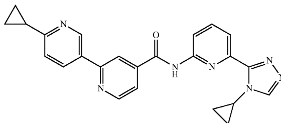
6'-cyclopropyl-N-(6-(4-cyclopropyl-4H-1,2,4-triazol-3-yl)pyridin-2-yl)-2,3'-bipyridine-4-carboxamide
