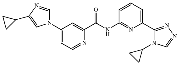
4-(4-cyclopropyl-1H-imidazol-1-yl)-N-(6-(4-cyclopropyl-4H-1,2,4-triazol-3-yl)pyridin-2-yl)picolinamide
