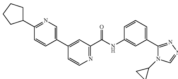
6-cyclopentyl-N-(3-(4-cyclopropyl-4H-1,2,4-triazol- 3-yl)phenyl)-3,4'-bipyridine-2'-carboxamide
