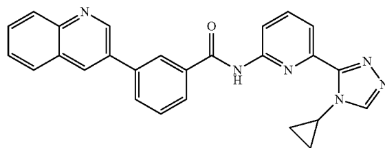
N-(6-(4-cyclopropyl-4H-1,2,4-triazol-3-yl)pyridin-2-yl)-3-(quinolin-3-yl)benzamide
