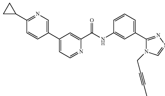
N-(3-(4-(but-2-ynyl)-4H-1,2,4-triazol-3-yl)phenyl)-6-cyclopropyl-3,4'-bipyridine-2'-carboxamide
