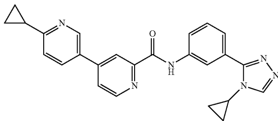
6-cyclopropyl-N-(3-(4-cyclopropyl-4H-1,2,4-triazol-3-yl)phenyl)-3,4'-bipyridine-2'-carboxamide
