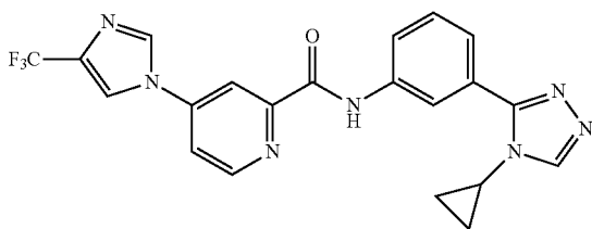
N-(3-(4-cyclopropyl-4H-1,2,4-triazol-3-yl)phenyl)- 4-(4-(trifluoromethyl)-1H-imidazol-1-yl)picolinamide
