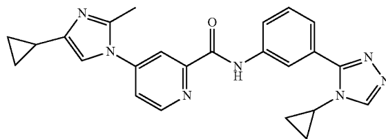
4-(4-cyclopropyl-2-methyl-1H-imidazol-1-yl)-N-(3-(4-cyclopropyl-4H-1,2,4-triazol-3-yl)phenyl)picolinamide
