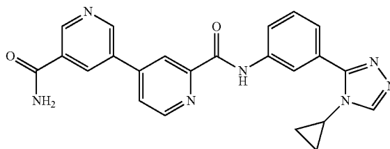
N2'-(3-(4-cyclopropyl-4H-1,2,4-triazol-3-yl)phenyl)-3,4'-bipyridine-2',5-dicarboxamide
