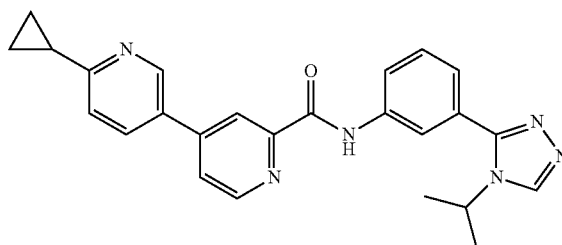
6-cyclopropyl-N-(3-(4-isopropyl-4H-1,2,4-triazol-3-yl)phenyl)-3,4'-bipyridine-2'-carboxamide
