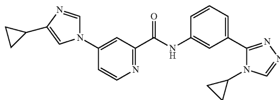
4-(4-cyclopropyl-1H-imidazol-1-yl)-N-(3-(4-cyclopropyl-4H-1,2,4-triazol-3-yl)phenyl)picolinamide
