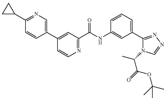
(S)-tert-butyl 2-(3-(3-(6-cyclopropyl-3,4'-bipyridine-2'-carboxamido)phenyl)-4H-1,2,4-triazol-4-yl)propanoate
