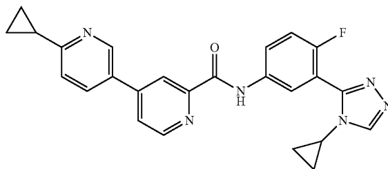
6-cyclopropyl-N-(3-(4-cyclopropyl-4H-1,2,4-triazol-3-yl)-4-fluorophenyl)-3,4'-bipyridine-2'-carboxamide
