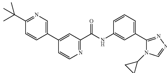
6-tert-butyl-N-(3-(4-cyclopropyl-4H-1,2,4-triazol-3-yl)phenyl)-3,4'-bipyridine-2'-carboxamide
