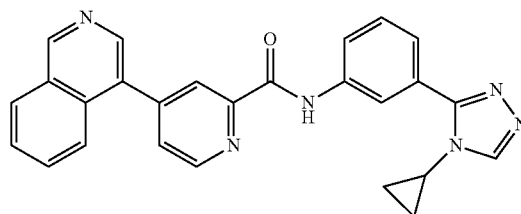
N-(3-(4-cyclopropyl-4H-1,2,4-triazol-3-yl)phenyl)-4-(isoquinolin-4-yl)picolinamide
