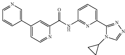
N-(6-(4-cyclopropyl-4H-1,2,4-triazol-3-yl)pyridin-2-yl)-3,4'-bipyridine-2'-carboxamide
