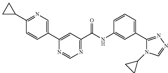
N-(3-(4-cyclopropyl-4H-1,2,4-triazol-3-yl)phenyl)-6-(6-cyclopropylpyridin-3-yl)pyrimidine-4-carboxamide
