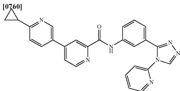
6-cyclopropyl-N-(3-(4-(pyridin-2-yl)-4H-1,2,4-triazol-3-yl)phenyl)-3,4'-bipyridine-2'-carboxamide
