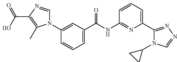
1-(3-(6-(4-cyclopropyl-4H-1,2,4-triazol-3-yl)pyridin-2-ylcarbamoyl)phenyl)-5-methyl-1H-imidazole-4-carboxylic acid
