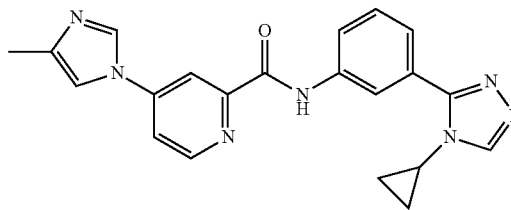
N-(3-(4-cyclopropyl-4H-1,2,4-triazol-3-yl)phenyl)-4-(4-methyl-1H-imidazol-1-yl)picolinamide
