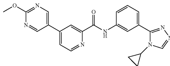
N-(3-(4-cyclopropyl-4H-1,2,4-triazol-3-yl)phenyl)- 4-(2-methoxypyrimidin-5-yl)picolinamide
