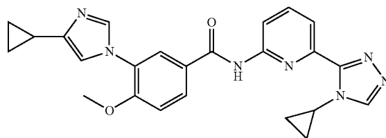
3-(4-cyclopropyl-1H-imidazol-1-yl)-N-(6-(4-cyclopropyl-4H-1,2,4-triazol-3-yl)pyridin-2-yl)-4-methoxybenzamide
