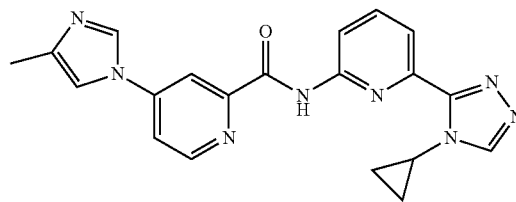
N-(6-(4-cyclopropyl-4H-1,2,4-triazol-3-yl)pyridin-2-yl)-4-(4-methyl-1H-imidazol-1-yl)picolinamide
