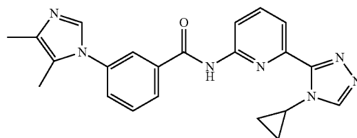
N-(6-(4-cyclopropyl-4H-1,2,4-triazol-3-yl)pyridin-2-yl)-3-(4,5-dimethyl-1H-imidazol-1-yl)benzamide
