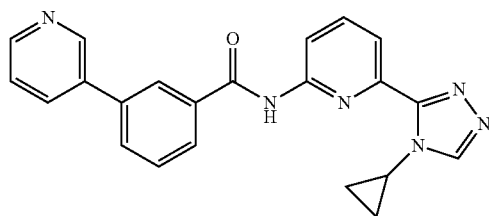
N-(6-(4-cyclopropyl-4H-1,2,4-triazol-3-yl)pyridin-2-yl)-3-(pyridin-3-yl)benzamide
