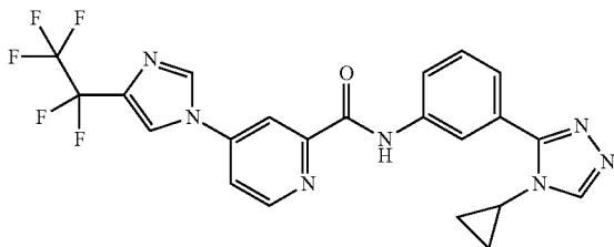
N-(3-(4-cyclopropyl-4H-1,2,4-triazol-3-yl)phenyl)-4-(4-(perfluoroethyl)-1H-imidazol-1-yl)picolinamide
