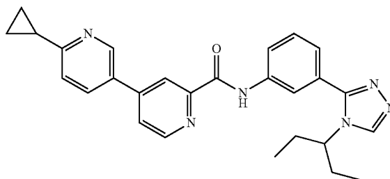
6-cyclopropyl-N-(3-(4-(pentan-3-yl)-4H-1,2,4-triazol-3-yl)phenyl)-3,4'-bipyridine-2'-carboxamide
