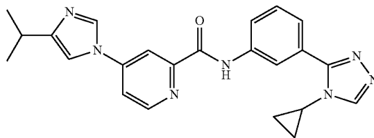
N-(3-(4-cyclopropyl-4H-1,2,4-triazol-3-yl)phenyl)-4-(4-isopropyl-1H-imidazol-1-yl)picolinamide
