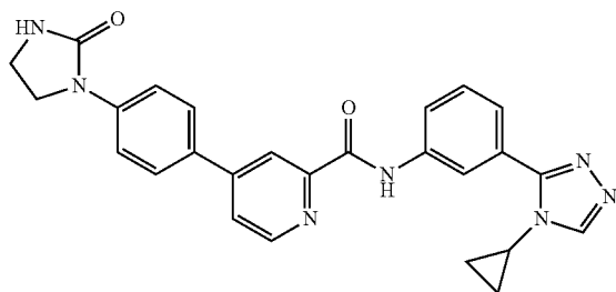
N-(3-(4-cyclopropyl-4H-1,2,4-triazol-3-yl)phenyl)-4-(4-(2-oxoimidazolidin-1-yl)phenyl)picolinamide
