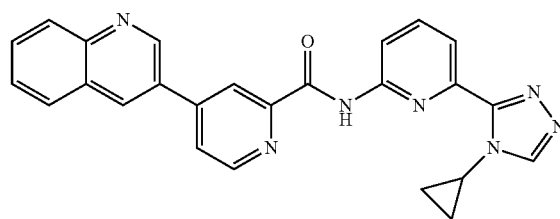
N-(6-(4-cyclopropyl-4H-1,2,4-triazol-3-yl)pyridin-2-yl)-4-(quinolin-3-yl)picolinamide
