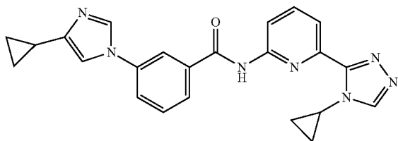
3-(4-cyclopropyl-1H-imidazol-1-yl)-N-(6-(4-cyclopropyl-4H-1,2,4-triazol-3-yl)pyridin-2-yl)benzamide
