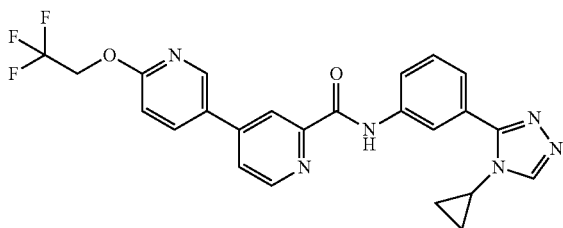
N-(3-(4-cyclopropyl-4H-1,2,4-triazol-3-yl)phenyl)-6-(2,2,2-trifluoroethoxy)-3,4'-bipyridine-2'-carboxamide
