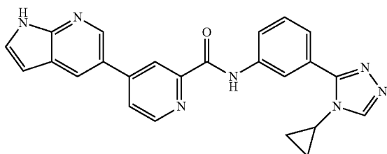
N-(3-(4-cyclopropyl-4H-1,2,4-triazol-3-yl)phenyl)-4-(1H-pyrrolo[2,3-b]pyridin-5-yl)picolinamide
