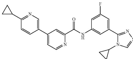
6-cyclopropyl-N-(3-(4-cyclopropyl-4H-1,2,4-triazol-3-yl)-5-fluorophenyl)-3,4'-bipyridine-2'-carboxamide
