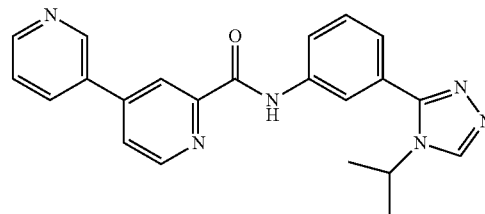
N-(3-(4-isopropyl-4H-1,2,4-triazol-3-yl)phenyl)-3,4'-bipyridine-2'-carboxamide
