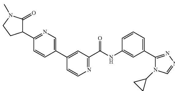
N-(3-(4-cyclopropyl-4H-1,2,4-triazol-3-yl)phenyl)- 6-(1-methyl-2-oxopyrrolidin-3-yl)-3,4'-bipyridine-2'- carboxamide
