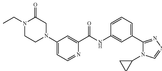
N-(3-(4-cyclopropyl-4H-1,2,4-triazol-3-yl)phenyl)-4-(4-ethyl-3-oxopiperazin-1-yl)picolinamide
