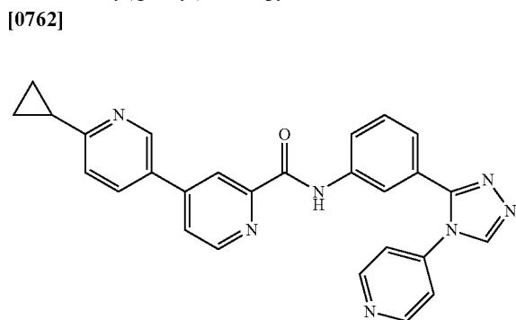
6-cyclopropyl-N-(3-(4-(pyridin-3-yl)-4H-1,2,4-triazol-3-yl)phenyl)-3,4'-bipyridine-2'-carboxamide
