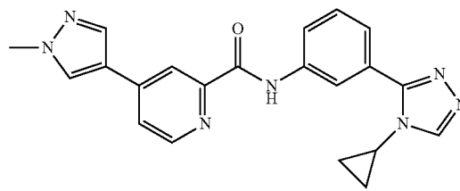
N-(3-(4-cyclopropyl-4H-1,2,4-triazol-3-yl)phenyl)-4-(1-methyl-1H-pyrazol-4-yl)picolinamide
