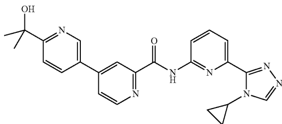
N-(6-(4-cyclopropyl-4H-1,2,4-triazol-3-yl)pyridin-2-yl)-6-(2-hydroxypropan-2-yl)-3,4'-bipyridine-2'-carboxamide
