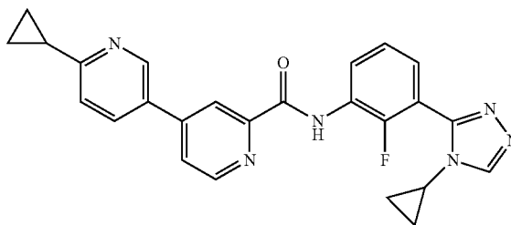
6-cyclopropyl-N-(3-(4-cyclopropyl-4H-1,2,4-triazol-3-yl)-2-fluorophenyl)-3,4'-bipyridine-2'-carboxamide
