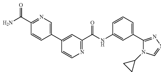
N2'-(3-(4-cyclopropyl-4H-1,2,4-triazol-3-yl)phenyl)-3,4'-bipyridine-2',6-dicarboxamide
