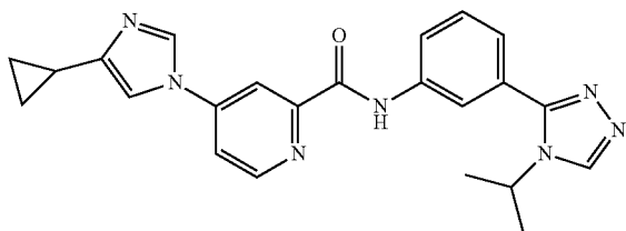
4-(4-cyclopropyl-1H-imidazol-1-yl)-N-(3-(4-isopropylphenyl)picolinamide
