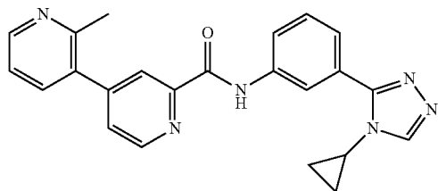
N-(3-(4-cyclopropyl-4H-1,2,4-triazol-3-yl)phenyl)-2-methyl-3,4'-bipyridine-2'-carboxamide
