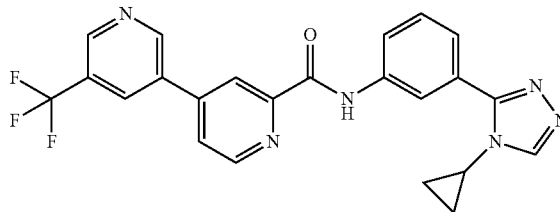
N-(3-(4-cyclopropyl-4H-1,2,4-triazol-3-yl)phenyl)-5-(trifluoromethyl)-3,4'-bipyridine-2'-carboxamide
