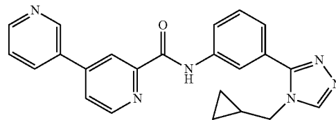
N-(3-(4-(cyclopropylmethyl)-4H-1,2,4-triazol-3-yl)phenyl)-3,4'-bipyridine-2'-carboxamide
