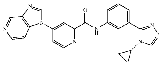
N-(3-(4-cyclopropyl-4H-1,2,4-triazol-3-yl)phenyl)- 4-(1H-imidazo[4,5-c]pyridin-1-yl)picolinamide
