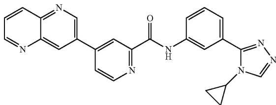
N-(3-(4-cyclopropyl-4H-1,2,4-triazol-3-yl)phenyl)-4-(1,5-naphthyridin-3-yl)picolinamide
