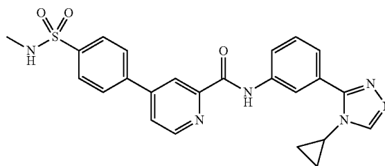
N-(3-(4-cyclopropyl-4H-1,2,4-triazol-3-yl)phenyl)-4-(N-methylsulfamoyl)-phenylpicolinamide
