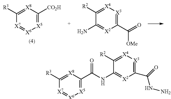
REACTION SCHEME XI Alternative Preparation of a Precursor to a Compound of Formula (I)
