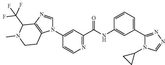
N-(3-(4-cyclopropyl-4H-1,2,4-triazol-3-yl)phenyl)- 4-(5-methyl-4-(trifluoromethyl)-4,5,6,7-tetrahydro- 1H-imidazo[4,5-c]pyridin-1-yl)picolinamide
