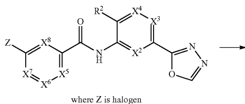
REACTION SCHEME XII Alternative Preparation of an Oxadiazole Precursor to a Compound of Formula (I)
