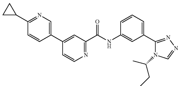
(S)-N-(3-(4-sec-butyl-4H-1,2,4-triazol-3-yl)phenyl)-6-cyclopropyl-3,4'-bipyridine-2'-carboxamide
