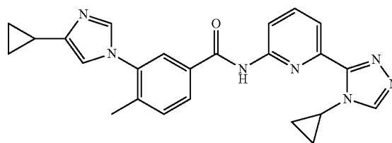
3-(4-cyclopropyl-1H-imidazol-1-yl)-N-(6-(4-cyclopropyl-4H-1,2,4-triazol-3-yl)pyridin-2-yl)-4-methylbenzamide
