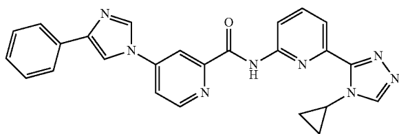
N-(6-(4-cyclopropyl-4H-1,2,4-triazol-3-yl)pyridin-2-yl)-4-(4-phenyl-1H-imidazol-1-yl)picolinamide
