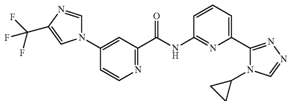
N-(6-(4-cyclopropyl-4H-1,2,4-triazol-3-yl)pyridin-2-yl)-4-(4-(trifluoromethyl)-1H-imidazol-1-yl)picolinamide
