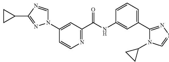
4-(3-cyclopropyl-1H-1,2,4-triazol-1-yl)-N-(3-(4-cyclopropyl-4H-1,2,4-triazol-3-yl)phenyl)picolinamide
