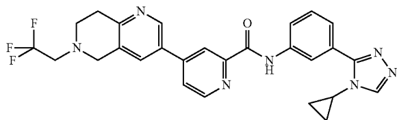
N-(3-(4-cyclopropyl-4H-1,2,4-triazol-3-yl)phenyl)-4-(6-(2,2,2-trifluoroethyl)-5,6,7,8-tetrahydro-1,6-naphthyridin-3-yl)picolinamide
