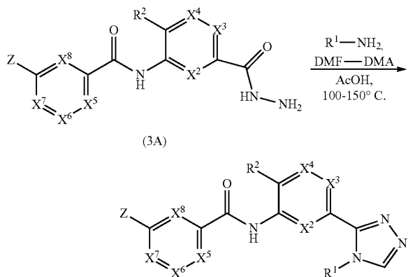
REACTION SCHEME X Alternative Preparation of a Precursor to a Compound of Formula (I)
