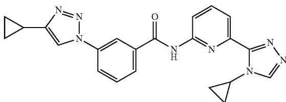
3-(4-cyclopropyl-1H-1,2,3-triazol-1-yl)-N-(6-(4- cyclopropyl-4H-1,2,4-triazol-3-yl)pyridin-2-yl)benz- amide
