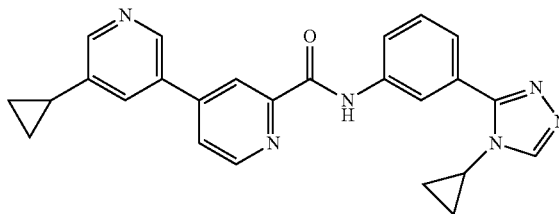
5-cyclopropyl-N-(3-(4-cyclopropyl-4H-1,2,4-triazol-3-yl)phenyl)-3,4'-bipyridine-2'-carboxamide
