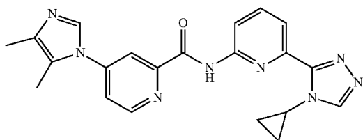
N-(6-(4-cyclopropyl-4H-1,2,4-triazol-3-yl)pyridin-2-yl)-4-(4,5-dimethyl-1H-imidazol-1-yl)picolinamide
