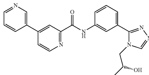
(R)—N-(3-(4-(2-hydroxypropyl)-4H-1,2,4-triazol-3-yl)phenyl)-3,4'-bipyridine-2'-carboxamide
