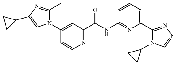
4-(4-cyclopropyl-2-methyl-1H-imidazol-1-yl)-N-(6-(4-cyclopropyl-4H-1,2,4-triazol-3-yl)pyridin-2-yl)picolinamide
