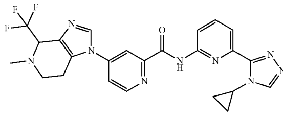
N-(6-(4-cyclopropyl-4H-1,2,4-triazol-3-yl)pyridin-2-yl)-4-(5-methyl-4-(trifluoromethyl)-4,5,6,7-tetrahydro-1H-imidazo[4,5-c]pyridin-1-yl)picolinamide
