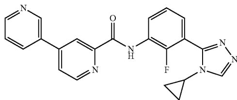
N-(3-(4-cyclopropyl-4H-1,2,4-triazol-3-yl)-2-fluorophenyl)-3,4'-bipyridine-2'-carboxamide
