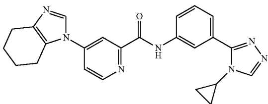
N-(3-(4-cyclopropyl-4H-1,2,4-triazol-3-yl)phenyl)- 4-(4,5,6,7-tetrahydro-1H-benzo[d]imidazol-1-yl) picolinamide
