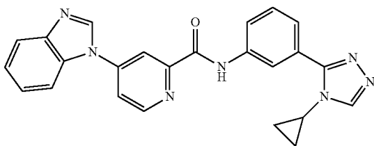
4-(1H-benzo[d]imidazol-1-yl)-N-(3-(4-cyclopropyl-4H-1,2,4-triazol-3-yl)phenyl)picolinamide
