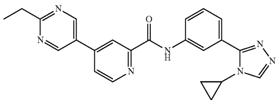
N-(3-(4-cyclopropyl-4H-1,2,4-triazol-3-yl)phenyl)-4-(2-ethylpyrimidin-5-yl)picolinamide
