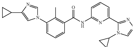
3-(4-cyclopropyl-1H-imidazol-1-yl)-N-(6-(4-cyclopropyl-4H-1,2,4-triazol-3-yl)pyridin-2-yl)-2-methylbenzamide
