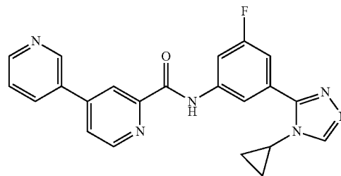
N-(3-(4-cyclopropyl-4H-1,2,4-triazol-3-yl)-5-fluorophenyl)-3,4'-bipyridine-2'-carboxamide
