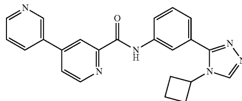
N-(3-(4-(cyclobutyl)-4H-1,2,4-triazol-3-yl)phenyl)-3,4'-bipyridine-2'-carboxamide
