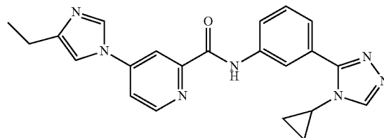
N-(3-(4-cyclopropyl-4H-1,2,4-triazol-3-yl)phenyl)- 4-(4-ethyl-1H-imidazol-1-yl)picolinamide
