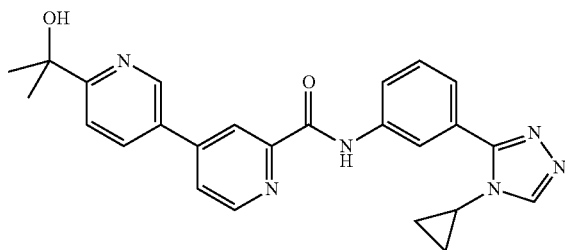
N-(3-(4-cyclopropyl-4H-1,2,4-triazol-3-yl)phenyl)-6-(2-hydroxypropan-2-yl)-3,4'-bipyridine-2'-carboxamide
