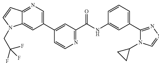
N-(3-(4-cyclopropyl-4H-1,2,4-triazol-3-yl)phenyl)-4-(1-(2,2,2-trifluoroethyl)-1H-pyrrolo[3,2-b]pyridin-6-yl)picolinamide
