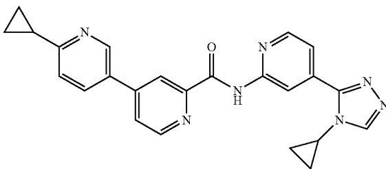
6-cyclopropyl-N-(4-(4-cyclopropyl-4H-1,2,4-triazol-3-yl)pyridin-2-yl)-3,4'-bipyridine-2'-carboxamide
