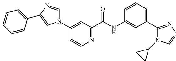
N-(3-(4-cyclopropyl-4H-1,2,4-triazol-3-yl)phenyl)-4-(4-phenyl-1H-imidazol-1-yl)picolinamide
