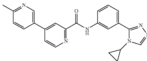
N-(3-(4-cyclopropyl-4H-1,2,4-triazol-3-yl)phenyl)-6-methyl-3,4'-bipyridine-2'-carboxamide
