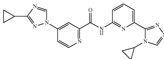
4-(3-cyclopropyl-1H-1,2,4-triazol-1-yl)-N-(6-(4-cyclopropyl-4H-1,2,4-triazol-3-yl)pyridin-2-yl)picolinamide
