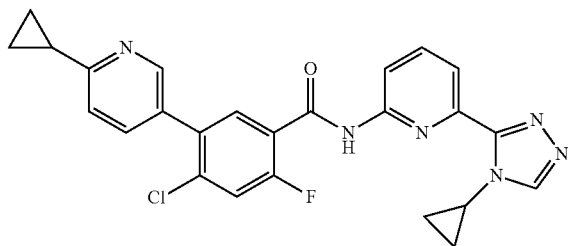
4-chloro-N-(6-(4-cyclopropyl-4H-1,2,4-triazol-3-yl)pyridin-2-yl)-5-(6-cyclopropylpyridin-3-yl)-2-fluorobenzamide
