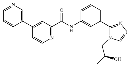
(S)—N-(3-(4-(2-hydroxypropyl)-4H-1,2,4-triazol-3-yl)phenyl)-3,4'-bipyridine-2'-carboxamide
