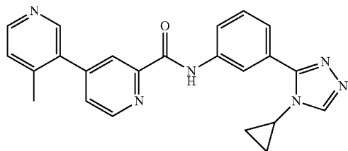
N-(3-(4-cyclopropyl-4H-1,2,4-triazol-3-yl)phenyl)-4-methyl-3,4'-bipyridine-2'-carboxamide
