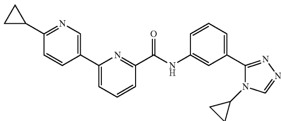
6'-cyclopropyl-N-(3-(4-cyclopropyl-4H-1,2,4-triazol-3-yl)phenyl)-2,3'-bipyridine-6-carboxamide
