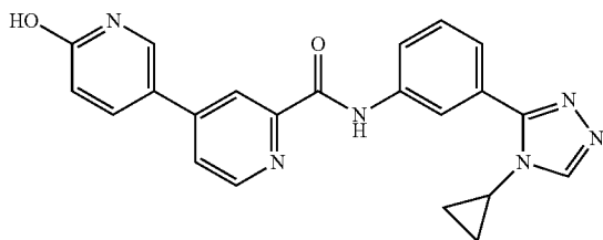
N-(3-(4-cyclopropyl-4H-1,2,4-triazol-3-yl)phenyl)- 6-hydroxy-3,4'-bipyridine-2'-carboxamide
