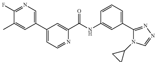
N-(3-(4-cyclopropyl-4H-1,2,4-triazol-3-yl)phenyl)-6-fluoro-5-methyl-3,4'-bipyridine-2'-carboxamide
