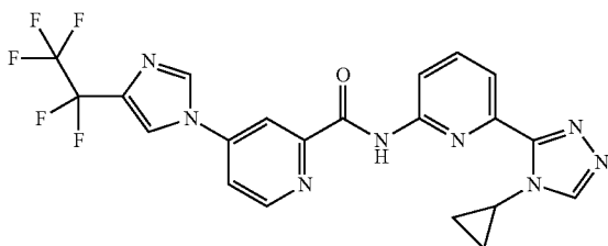
N-(6-(4-cyclopropyl-4H-1,2,4-triazol-3-yl)pyridin-2-yl)-4-(4-(perfluoroethyl)-1H-imidazol-1-yl)picolinamide
