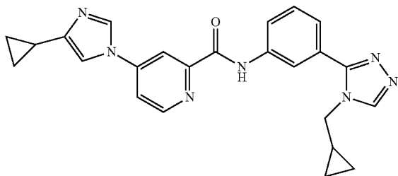
4-(4-cyclopropyl-1H-imidazol-1-yl)-N-(3-(4-(cyclopropylmethyl)-4H-1,2,4-triazol-3-yl)phenyl)picolinamide
