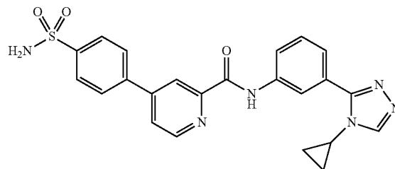
N-(3-(4-cyclopropyl-4H-1,2,4-triazol-3-yl)phenyl)-4-(4-sulfamoylphenyl)picolinamide
