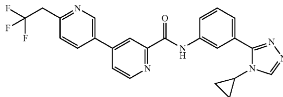
N-(3-(4-cyclopropyl-4H-1,2,4-triazol-3-yl)phenyl)-6-(2,2,2-trifluoroethyl)-3,4'-bipyridine-2'-carboxamide
