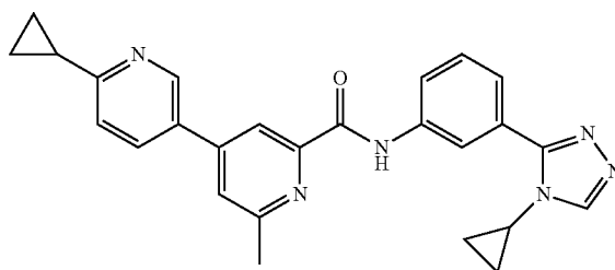
6-cyclopropyl-N-(3-(4-cyclopropyl-4H-1,2,4-triazol-3-yl)phenyl)-6'-methyl-3,4'-bipyridine-2'-carboxamide
