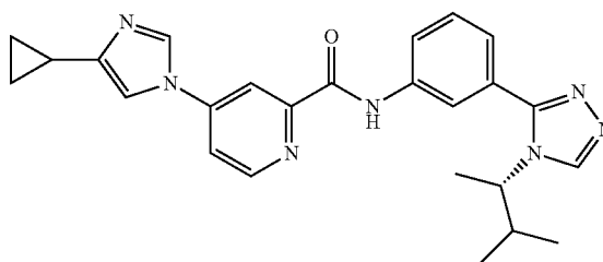
(S)-4-(4-cyclopropyl-1H-imidazol-1-yl)-N-(3-(4-(3- methylbutan-2-yl)-4H-1,2,4-triazol-3-yl)phenyl) picolinamide
