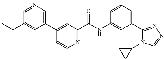
N-(3-(4-cyclopropyl-4H-1,2,4-triazol-3-yl)phenyl)-5-ethyl-3,4'-bipyridine-2'-carboxamide
