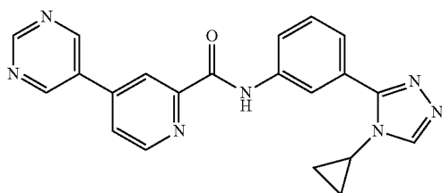
N-(3-(4-cyclopropyl-4H-1,2,4-triazol-3-yl)phenyl)- 4-(pyrimidin-5-yl)picolinamide
