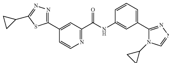
4-(5-cyclopropyl-1,3,4-thiadiazol-2-yl)-N-(3-(4-cyclopropyl-4H-1,2,4-triazol-3-yl)phenyl)picolinamide
