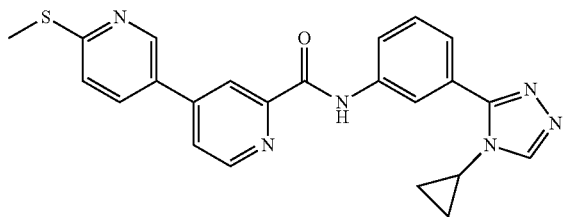
N-(3-(4-cyclopropyl-4H-1,2,4-triazol-3-yl)phenyl)-6-(methylthio)-3,4'-bipyridine-2'-carboxamide
