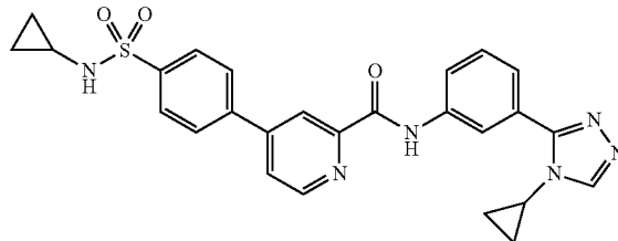
N-(3-(4-cyclopropyl-4H-1,2,4-triazol-3-yl)phenyl)-4-(N-cyclopropylsulfamoyl)-phenylpicolinamide
