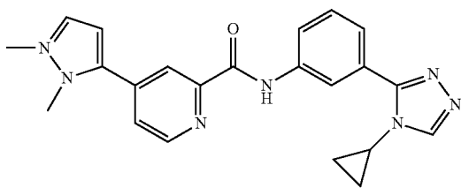
N-(3-(4-cyclopropyl-4H-1,2,4-triazol-3-yl)phenyl)-4-(1,2-dimethyl-1H-imidazol-5-yl)picolinamide
