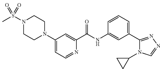
N-(3-(4-cyclopropyl-4H-1,2,4-triazol-3-yl)phenyl)-4-(4-(methylsulfonyl)piperazin-1-yl)picolinamide
