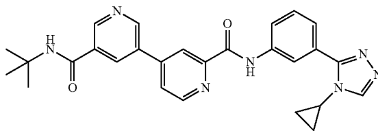
N5-tert-butyl-N2'-(3-(4-cyclopropyl-4H-1,2,4-triazol-3-yl)phenyl)-3,4'-bipyridine-2',5-dicarboxamide
