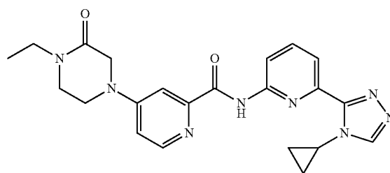
N-(6-(4-cyclopropyl-4H-1,2,4-triazol-3-yl)pyridin-2-yl)-4-(4-ethyl-3-oxopiperazin-1-yl)picolinamide
