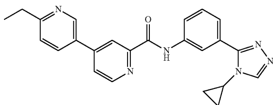
N-(3-(4-cyclopropyl-4H-1,2,4-triazol-3-yl)phenyl)- 6-ethyl-3,4'-bipyridine-2'-carboxamide
