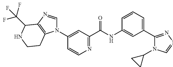
N-(3-(4-cyclopropyl-4H-1,2,4-triazol-3-yl)phenyl)-4-(4-(trifluoromethyl)-4,5,6,7-tetrahydro-1H-imidazo[4,5-c]pyridin-1-yl)picolinamide
