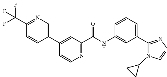
N-(3-(4-cyclopropyl-4H-1,2,4-triazol-3-yl)phenyl)-6-(trifluoromethyl)-3,4'-bipyridine-2'-carboxamide
