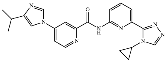
N-(6-(4-cyclopropyl-4H-1,2,4-triazol-3-yl)pyridin-2-yl)-4-(4-isopropyl-1H-imidazol-1-yl)picolinamide
