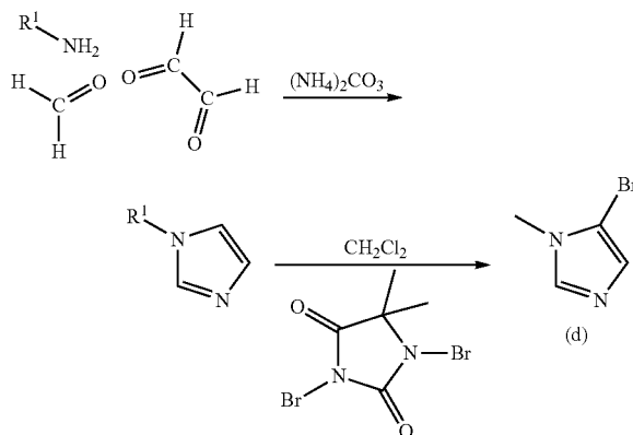
REACTION SCHEME XIII Synthesis of heterocyclic building blocks
