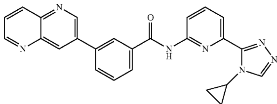
N-(6-(4-cyclopropyl-4H-1,2,4-triazol-3-yl)pyridin-2-yl)-3-(1,5-naphthyridin-3-yl)benzamide
