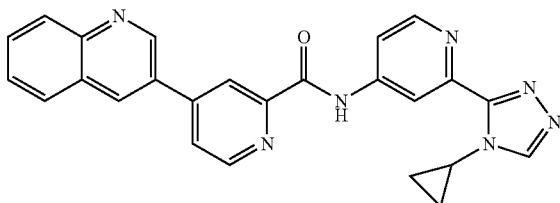
N-(2-(4-cyclopropyl-4H-1,2,4-triazol-3-yl)pyridin-4-yl)-4-(quinolin-3-yl)picolinamide
