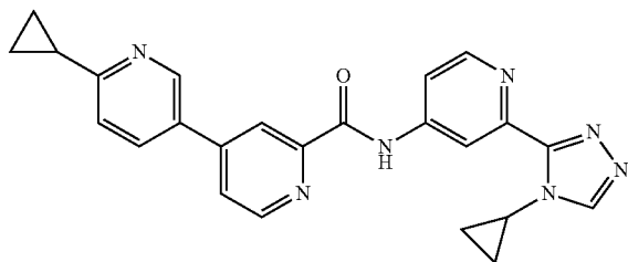
6-cyclopropyl-N-(2-(4-cyclopropyl-4H-1,2,4-triazol-3-yl)pyridin-4-yl)-3,4'-bipyridine-2'-carboxamide
