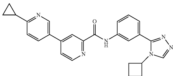
N-(3-(4-cyclobutyl-4H-1,2,4-triazol-3-yl)phenyl)-6-cyclopropyl-3,4'-bipyridine-2'-carboxamide
