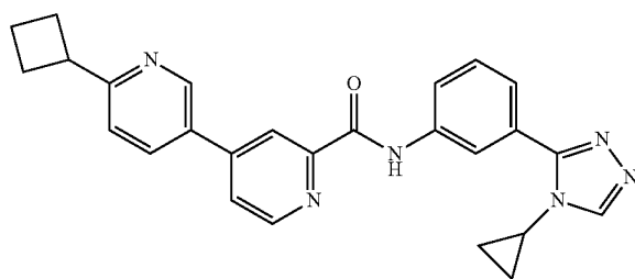
6-cyclobutyl-N-(3-(4-cyclopropyl-4H-1,2,4-triazol- 3-yl)phenyl)-3,4'-bipyridine-2'-carboxamide
