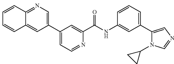
N-(3-(1-cyclopropyl-1H-imidazol-5-yl)phenyl)-4-(quinolin-3-yl)picolinamide
