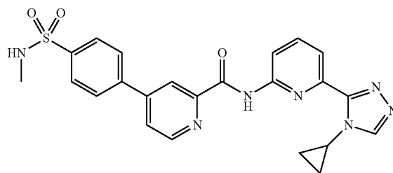
N-(6-(4-cyclopropyl-4H-1,2,4-triazol-3-yl)pyridin-2-yl)-4-(4-(N-methylsulfamoyl)phenyl)picolinamide
