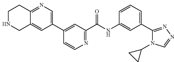
N-(3-(4-cyclopropyl-4H-1,2,4-triazol-3-yl)phenyl)-4-(5,6,7,8-tetrahydro-1,6-naphthyridin-3-yl)picolinamide
