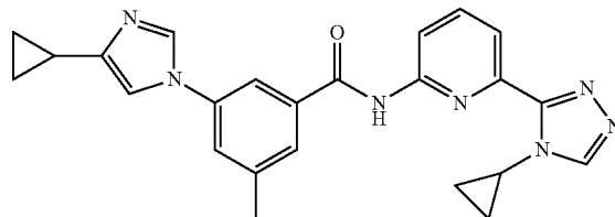
3-(4-cyclopropyl-1H-imidazol-1-yl)-N-(6-(4-cyclopropyl-4H-1,2,4-triazol-3-yl)pyridin-2-yl)-5-methylbenzamide
