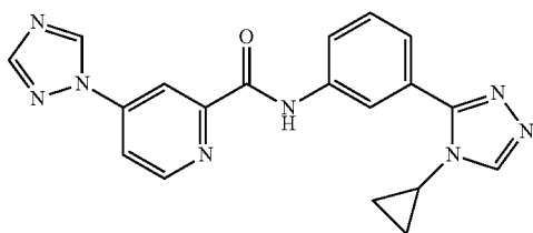
N-(3-(4-cyclopropyl-4H-1,2,4-triazol-3-yl)phenyl)-4-(1H-1,2,4-triazol-1-yl)picolinamide
