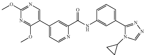
N-(3-(4-cyclopropyl-4H-1,2,4-triazol-3-yl)phenyl)-4-(2,4-dimethoxypyrimidin-5-yl)picolinamide
