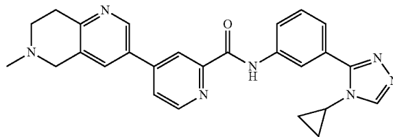
N-(3-(4-cyclopropyl-4H-1,2,4-triazol-3-yl)phenyl)-4-(6-methyl-5,6,7,8-tetrahydro-1,6-naphthyridin-3-yl)picolinamide
