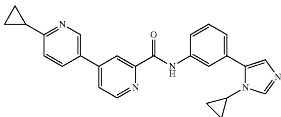
6-cyclopropyl-N-(3-(1-cyclopropyl-1H-imidazol-5-yl)phenyl)-3,4'-bipyridine-2'-carboxamide
