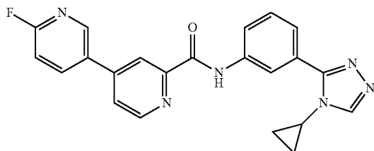
N-(3-(4-cyclopropyl-4H-1,2,4-triazol-3-yl)phenyl)-6-fluoro-3,4'-bipyridine-2'-carboxamide
