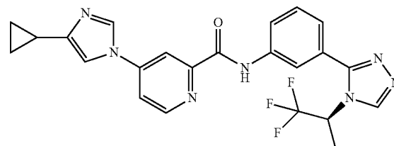
(S)-4-(4-cyclopropyl-1H-imidazol-1-yl)-N-(3-(4-(1,1,1-trifluoropropan-2-yl)-4H-1,2,4-triazol-3-yl)phenyl)picolinamide
