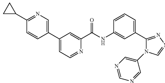
6-cyclopropyl-N-(3-(4-(pyrimidin-5-yl)-4H-1,2,4-triazol-3-yl)phenyl)-3,4'-bipyridine-2'-carboxamide
