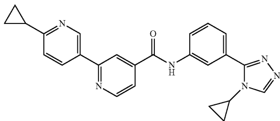
6'-cyclopropyl-N-(3-(4-cyclopropyl-4H-1,2,4-triazol-3-yl)phenyl)-2,3'-bipyridine-4-carboxamide
