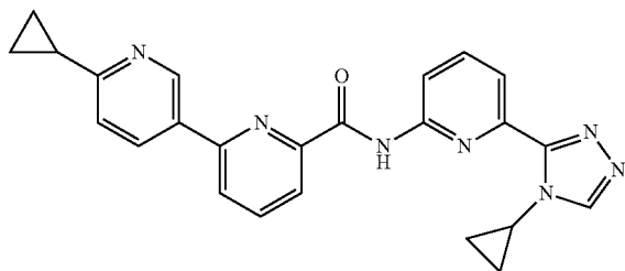
6'-cyclopropyl-N-(6-(4-cyclopropyl-4H-1,2,4-triazol-3-yl)pyridin-2-yl)-2,3'-bipyridine-6-carboxamide
