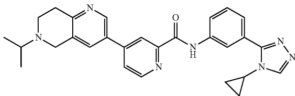
N-(3-(4-cyclopropyl-4H-1,2,4-triazol-3-yl)phenyl)-4-(6-isopropyl-5,6,7,8-tetrahydro-1,6-naphthyridin-3-yl)picolinamide
