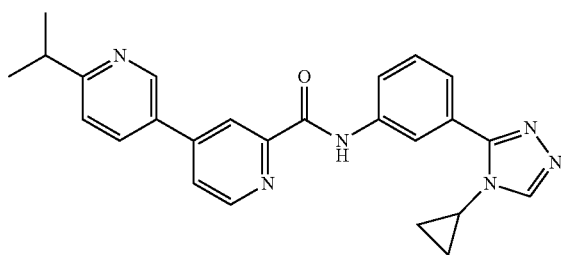
N-(3-(4-cyclopropyl-4H-1,2,4-triazol-3-yl)phenyl)- 6-isopropyl-3,4'-bipyridine-2'-carboxamide
