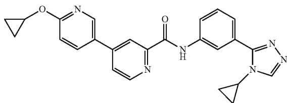
6-cyclopropoxy-N-(3-(4-cyclopropyl-4H-1,2,4-triazol-3-yl)phenyl)-3,4'-bipyridine-2'-carboxamide
