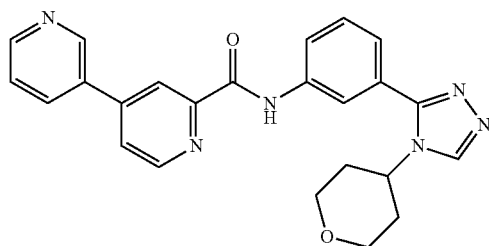
N-(3-(4-(tetrahydro-2H-pyran-4-yl)-4H-1,2,4-triazol-3-yl)phenyl)-3,4'-bipyridine-2'-carboxamide
