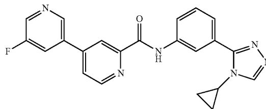
N-(3-(4-cyclopropyl-4H-1,2,4-triazol-3-yl)phenyl)-5-fluoro-3,4'-bipyridine-2'-carboxamide
