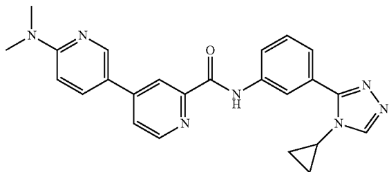
N-(3-(4-cyclopropyl-4H-1,2,4-triazol-3-yl)phenyl)-6-(dimethylamino)-3,4'-bipyridine-2'-carboxamide
