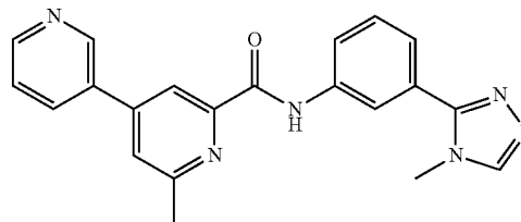
6'-methyl-N-(3-(4-methyl-4H-1,2,4-triazol-3-yl) phenyl)-3,4'-bipyridine-2'-carboxamide
