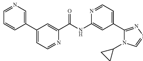
N-(4-(4-cyclopropyl-4H-1,2,4-triazol-3-yl)pyridin-2-yl)-3,4'-bipyridine-2'-carboxamide
