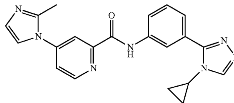
N-(3-(4-cyclopropyl-4H-1,2,4-triazol-3-yl)phenyl)-4-(2-methyl-1H-imidazol-1-yl)picolinamide
