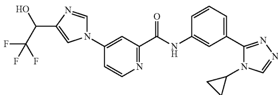
N-(3-(4-cyclopropyl-4H-1,2,4-triazol-3-yl)phenyl)-4-(4-(2,2,2-trifluoro-1-hydroxyethyl)-1H-imidazol-1-yl)picolinamide
