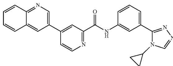
N-(3-(4-cyclopropyl-4H-1,2,4-triazol-3-yl)phenyl)-4-(quinolin-3-yl)picolinamide
