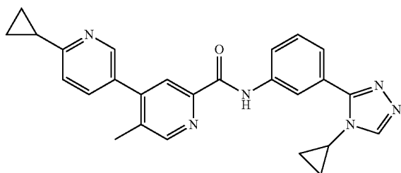
6-cyclopropyl-N-(3-(4-cyclopropyl-4H-1,2,4-triazol-3-yl)phenyl)-5'-methyl-3,4'-bipyridine-2'-carboxamide
