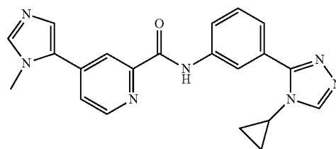
N-(3-(4-cyclopropyl-4H-1,2,4-triazol-3-yl)phenyl)- 4-(1-methyl-1H-imidazol-5-yl)picolinamide
