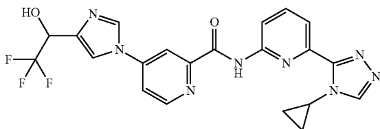
N-(6-(4-cyclopropyl-4H-1,2,4-triazol-3-yl)pyridin-2-yl)-4-(4-(2,2,2-trifluoro-1-hydroxyethyl)-1H-imidazol-1-yl)picolinamide
