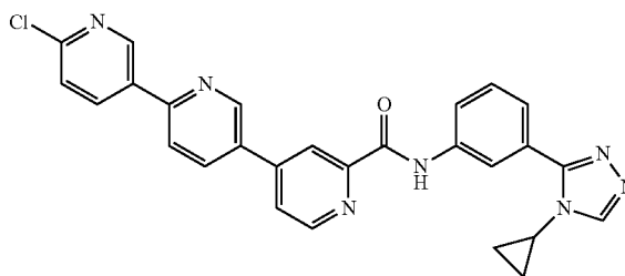
6-Chloro-[3,2';5',4'']terpyridine-2''-carboxylic acid [3-(4-cyclopropyl-4H-[1,2,4]triazol-3-yl)-phenyl]-amide
