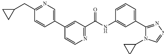
N-(3-(4-cyclopropyl-4H-1,2,4-triazol-3-yl)phenyl)-6-(cyclopropylmethyl)-3,4'-bipyridine-2'-carboxamide
