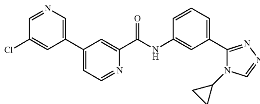
5-chloro-N-(3-(4-cyclopropyl-4H-1,2,4-triazol-3-yl)phenyl)-3,4'-bipyridine-2'-carboxamide
