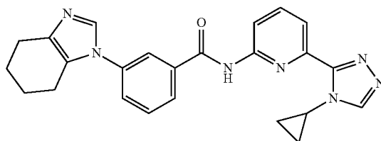
N-(6-(4-cyclopropyl-4H-1,2,4-triazol-3-yl)pyridin-2-yl)-3-(4,5,6,7-tetrahydro-1H-benzo[d]imidazol-1-yl)benzamide
