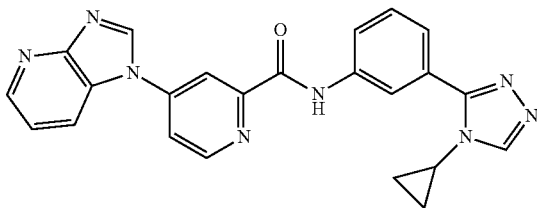
N-(3-(4-cyclopropyl-4H-1,2,4-triazol-3-yl)phenyl)- 4-(1H-imidazo[4,5-b]pyridin-1-yl)picolinamide
