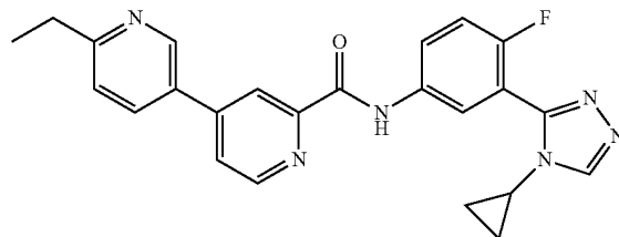
N-(3-(4-cyclopropyl-4H-1,2,4-triazol-3-yl)-4-fluorophenyl)-6-ethyl-3,4'-bipyridine-2'-carboxamide
