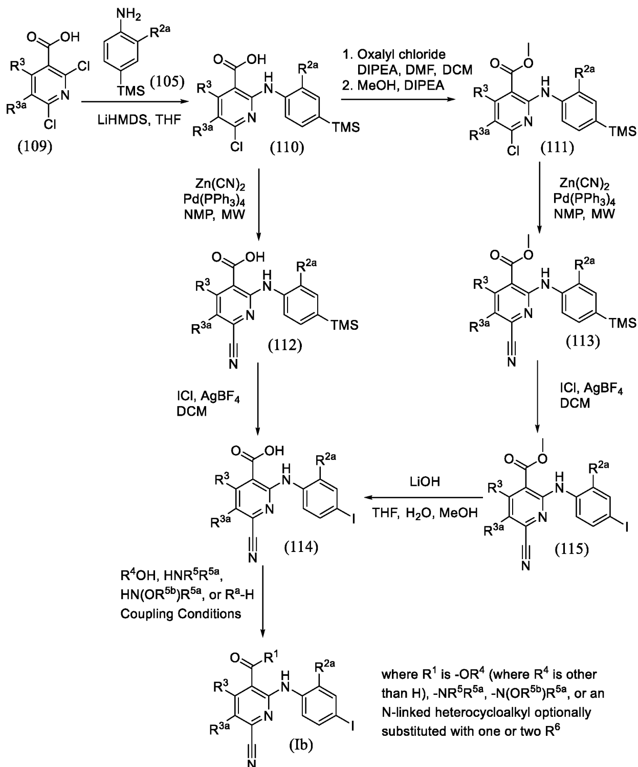
Scheme 3
