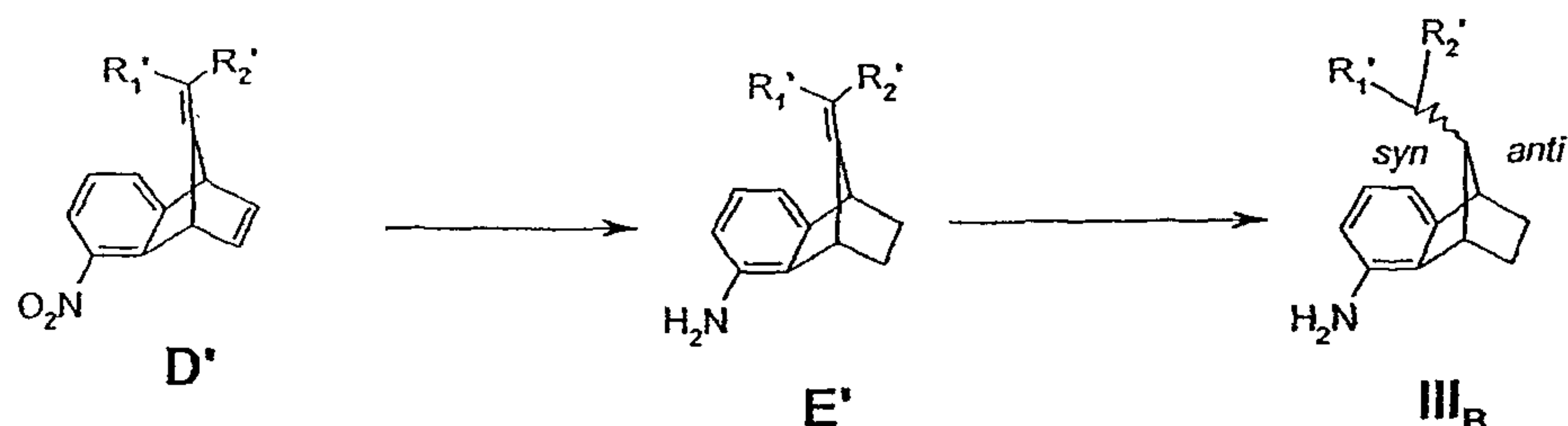
Scheme 2: Two-step hydrogenation
