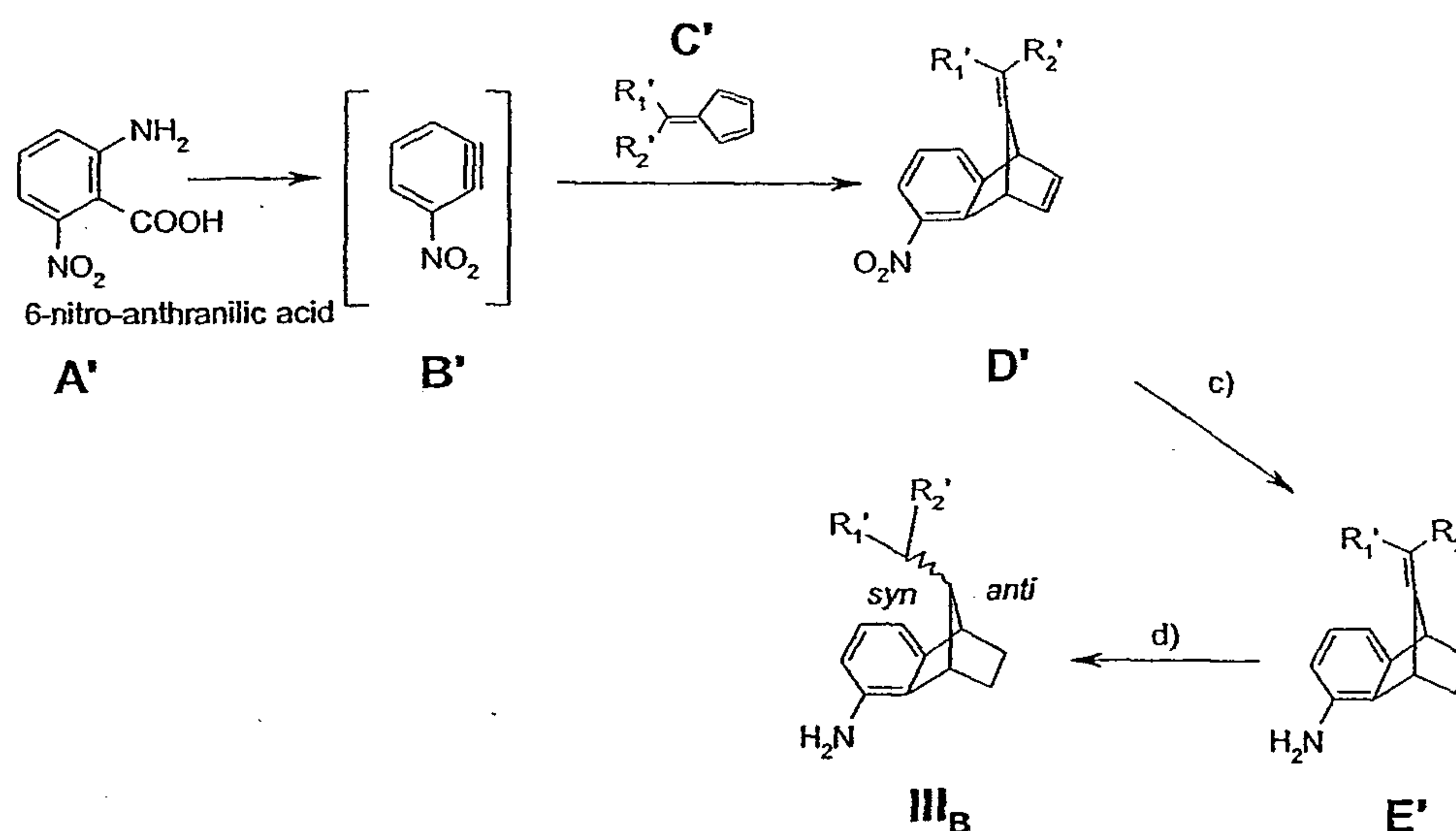
Scheme 1: Synthesis of III B using 6-nitroanthranilic acid
