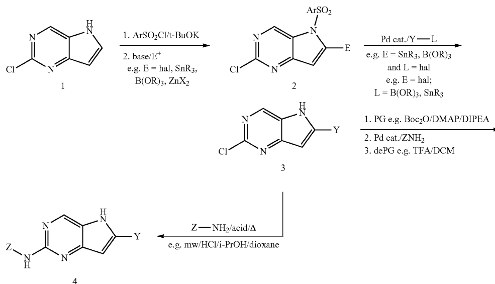
Scheme 1. Deprotonation-electrophilic activation for C-N coupling reactions
