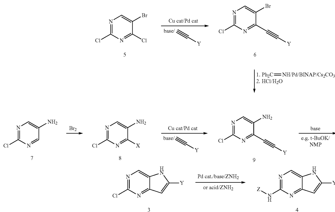
Scheme 2. Sonogashira Coupling and C-N coupling reactions.
