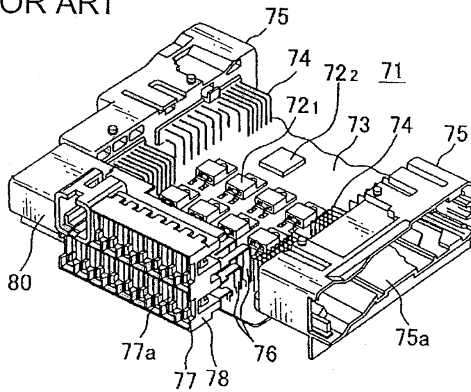
FIG. 8 PRIOR ART
