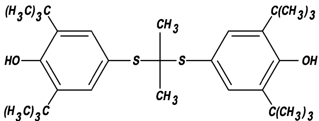
Probucol
