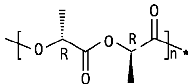
poly (D-lactide)
