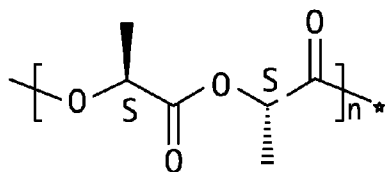
poly (L-lactide)
