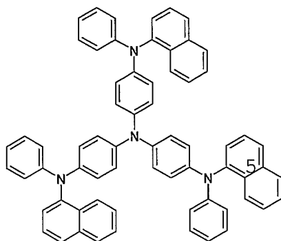
Chemical Formula 4
