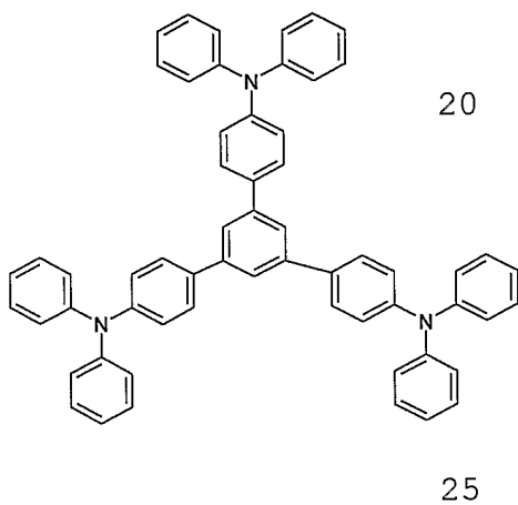
Chemical Formula 7
