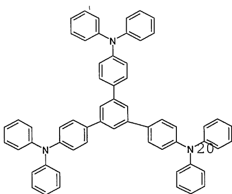
Chemical Formula 6
