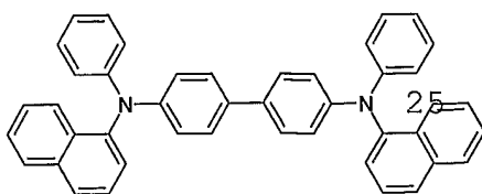
Chemical Formula 3
