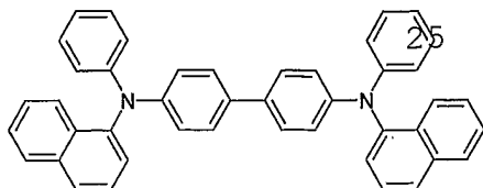
Chemical Formula 3
