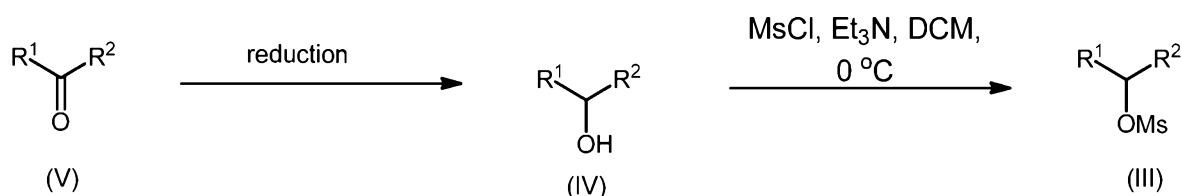
Reaction Scheme 4
