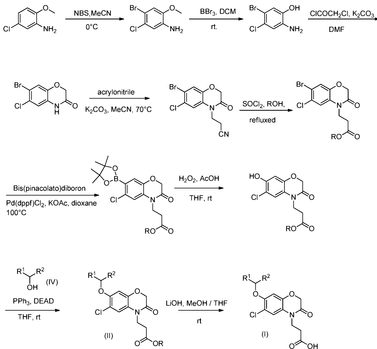
Reaction Scheme 1
