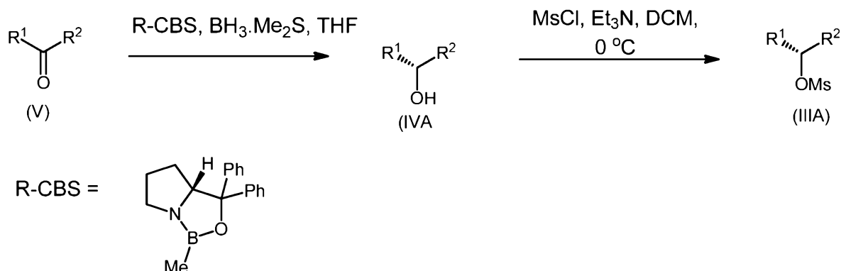
Reaction Scheme 5
