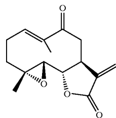
4. Parthenolid-9-one
