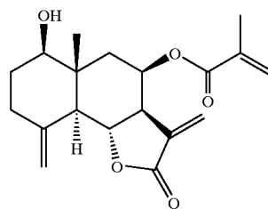
32. Arturin
