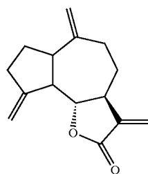
20. Dehydrocostus lactone
