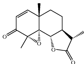
42. Epoxy(4,5α)-4,5-dihydrosantonin
