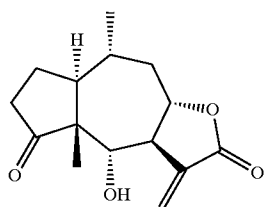
29. 6 \alpha -Hydroxy-2,3-dihydroaromaticin
