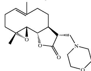
compound 49
