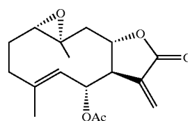
10. Pyrethrosine
