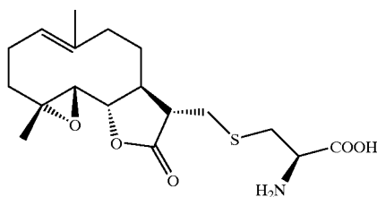
compound 53
