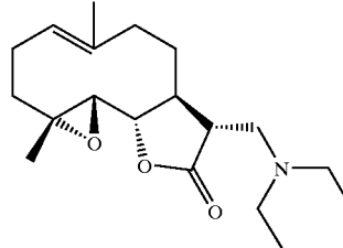
compound 45
