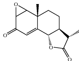
43. 4(5)α-epoxy-4,5-dihydrosantonin
