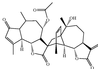
22. Arteminolide
