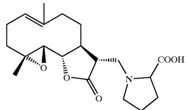
compound 50
