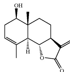
36. Santamarine
