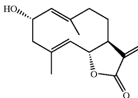
13. Tamaulipin A
