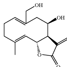
9. Deacetylovatifolin
