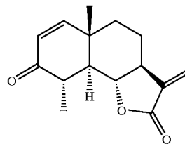
33. Tuberiferine
