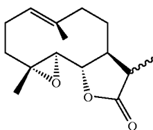
41. Dihydroparthenolide
