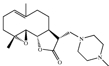
compound 52
