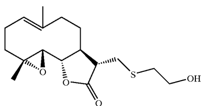
compound 51
