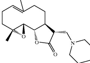
compound 47
