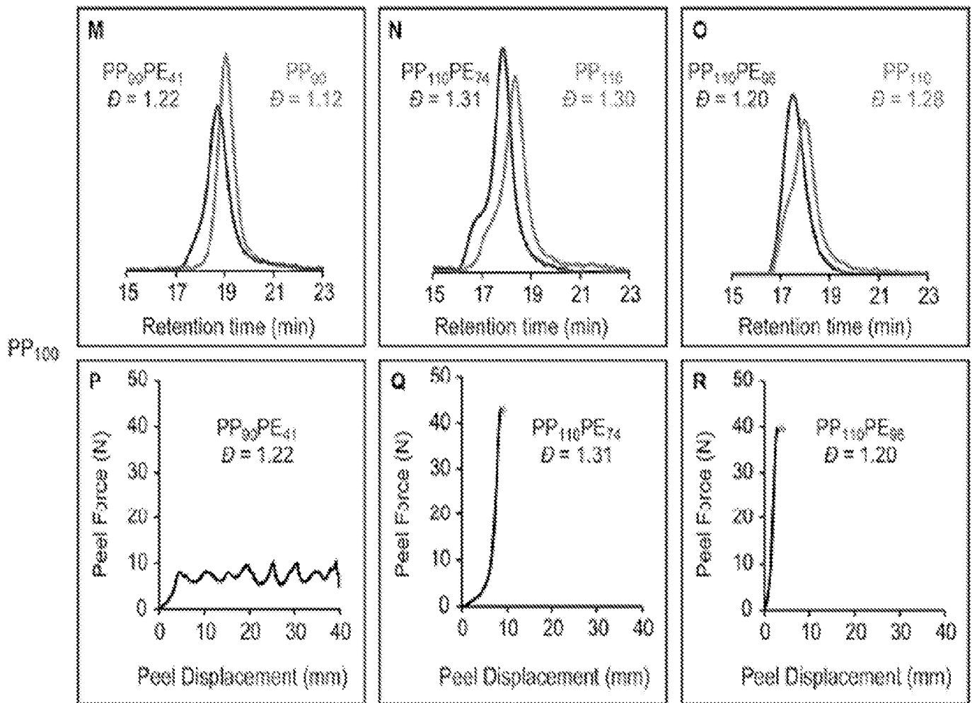
FIGS. 11M-R
