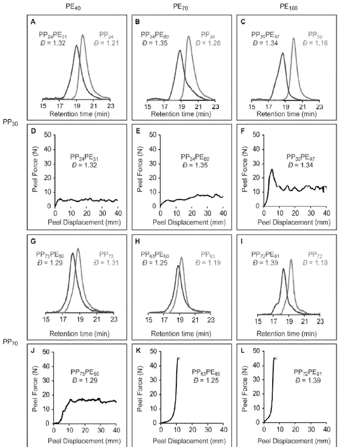
FIGS. 11A-L
