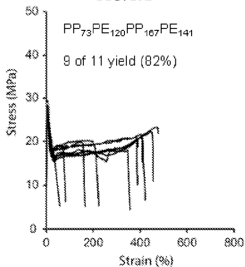
FIG. 23D
