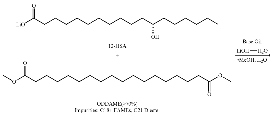
FIG. 2. Reaction of ODDAME with 12-HSA as complexing agent.
