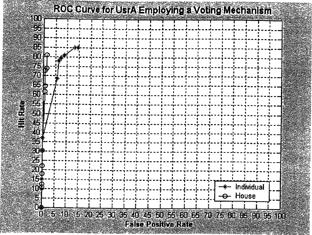
ROC Curve for 'usrA' using a voting scheme
