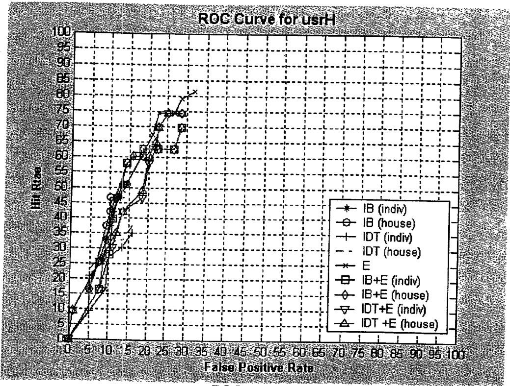
ROC curves for 'usrH'
