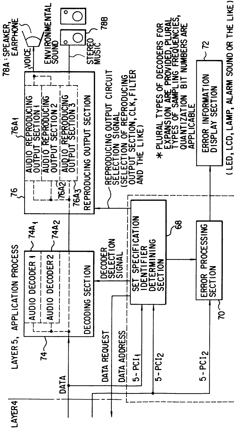
66: MICROCOMPUTER, CONTROLLER FIG. 16
