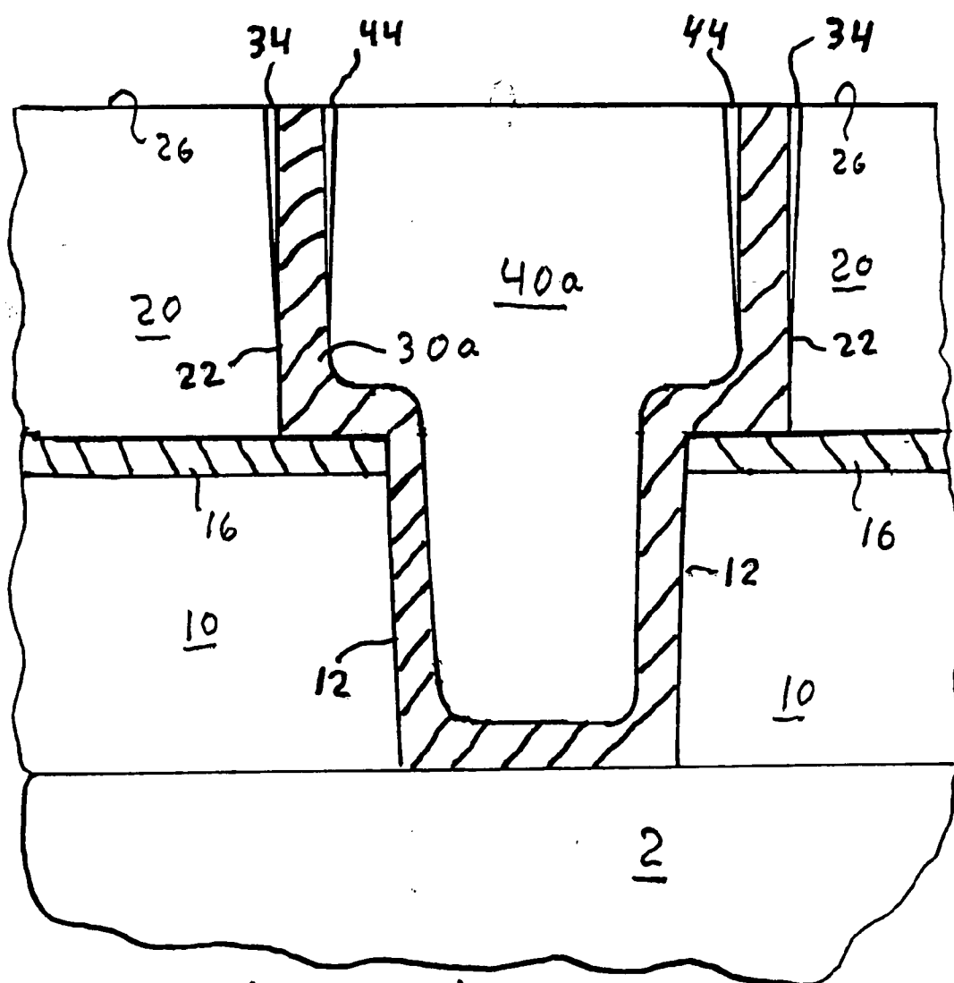
Fig. 6 (prior Art)
