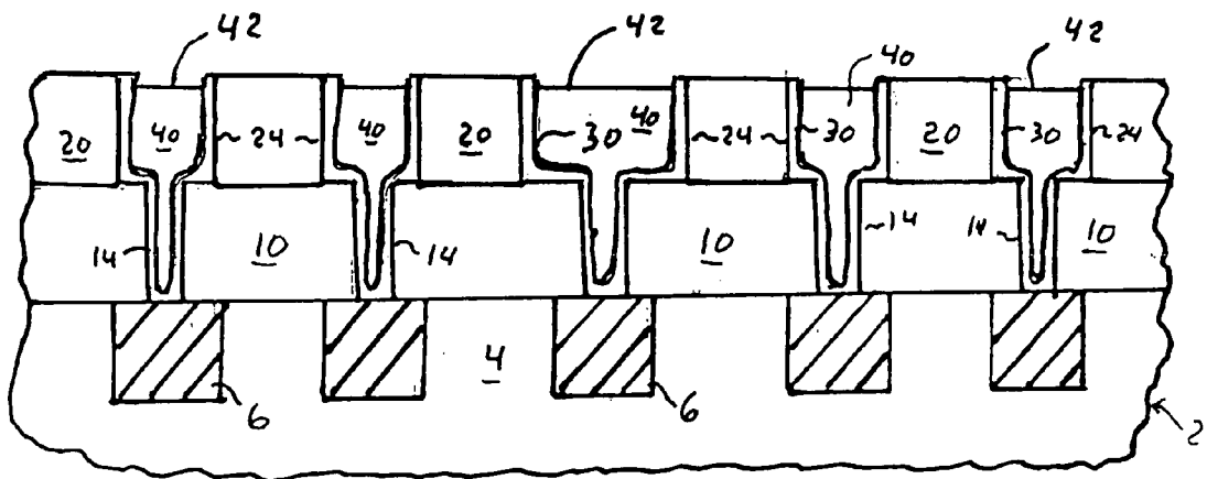
Fig. 3 (Prior Art)
