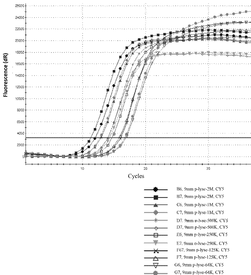
FIGURE 14 Amplification Plots
