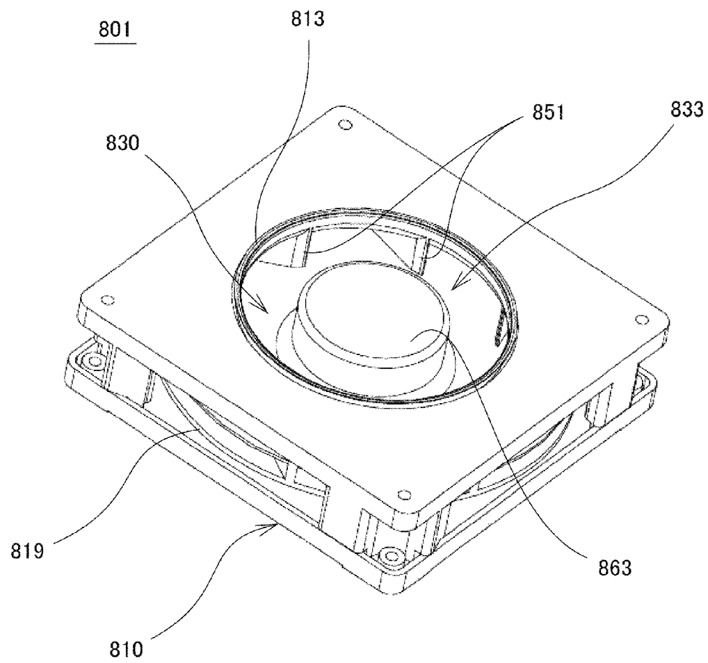
FIG. 15 RELATED ART
