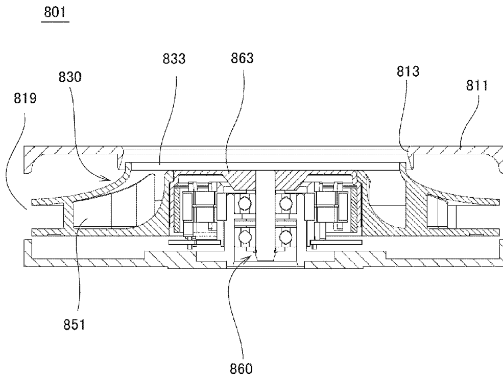
FIG. 16 RELATED ART
