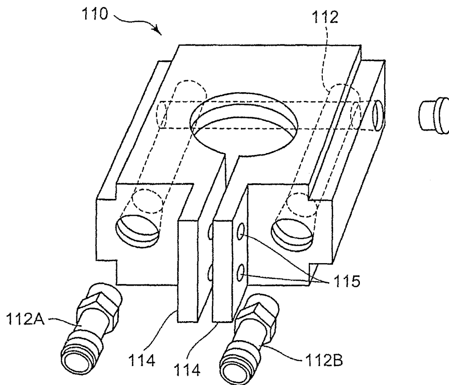
Fig. 10 PRIOR ART
