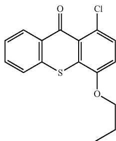
CPTX, photosensitizer 1-chloro-4-propoxy-9-H-thioxanthene-9-one CAS 142770-42-1
