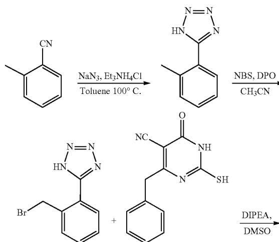
General Scheme K, 4-Benzyl-6-oxo-2-[2-(1H-tetrazol-5-yl)-benzylsulfanyl]-1,6-dihydro-pyrimidine-5-carbonitrile
