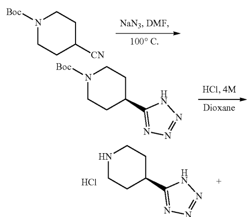
General Scheme I, 6-Oxo-2-[4-(1H-tetrazol-5-yl)-piperidin-1-yl]-4-thiophen-2-yl-1,6-dihydro-pyrimidine-5-carbonitrile
