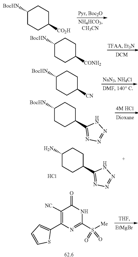
General Scheme H, 6-Oxo-2-[4-(1H-tetrazol-5-yl)-cyclohexylamino]-4-thiophen-2-yl-1,6-dihydro-pyrimidine-5-carbonitrile
