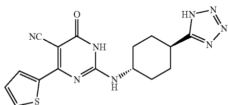
General Scheme I, 6-Oxo-2-[4-(1H-tetrazol-5-yl)-piperidin-1-yl]-4-thiophen-2-yl-1,6-dihydro-pyrimidine-5-carbonitrile
