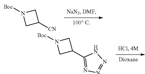
General Scheme J, 6-Oxo-2-[3-(1H-tetrazol-5-yl)-azetidin-1-yl]-4-thiophen-2-yl-1,6-dihydro-pyrimidine-5-carbonitrile
