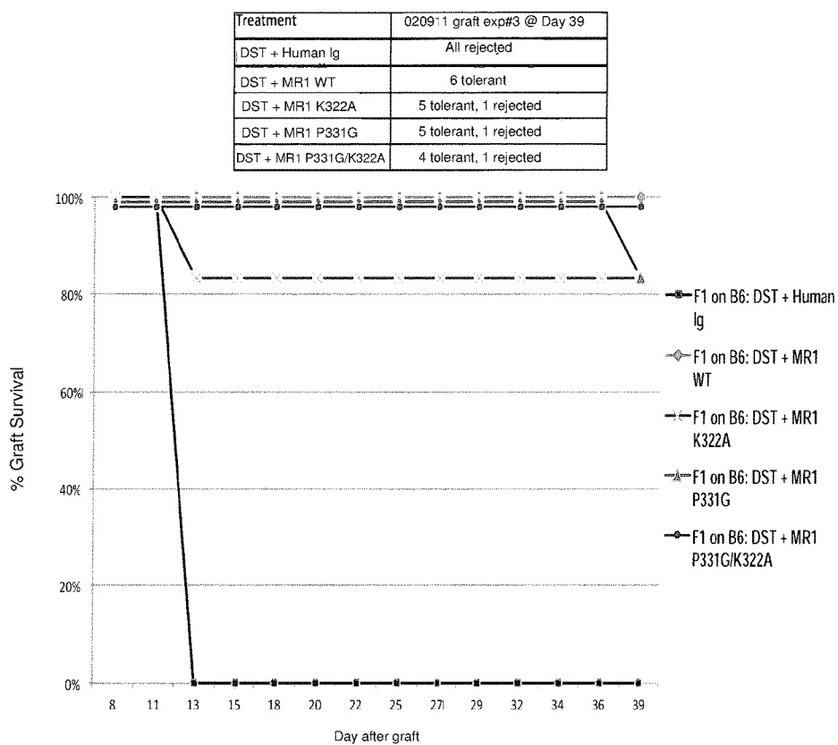
Figure 5. Loss of complement activation does not reduce the ability of anti-CD40L to induce tolerance.
