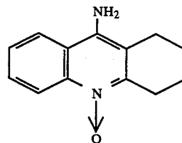
N-oxy-1,2,3,4-tetrahydro-5-aminoacridine
