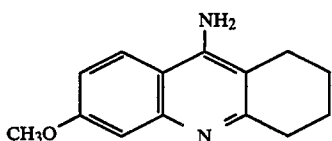
8-methoxy-1,2,3,4-tetrahydro-5-aminoacridine
