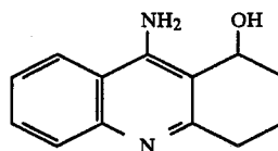
4-hydroxy-1,2,3,4-tetrahydro-5-aminoacridine
