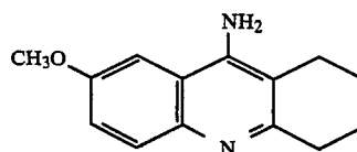
7-methoxy-1,2,3,4-tetrahydro-5-aminoacridine
