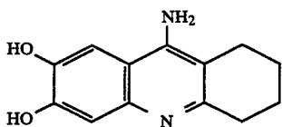
7,8-dihydroxy-1,2,3,4-tetrahydro-5-aminoacridine
