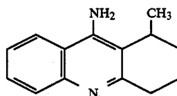
4-methyl-1,2,3,4-tetrahydro-5-aminoacridine
