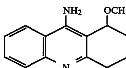
4-methoxy-1,2,3,4-tetrahydro-5-aminoacridine
