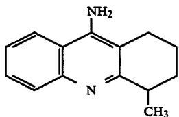
1-methyl-1,2,3,4-tetrahydro-5-aminoacridine
