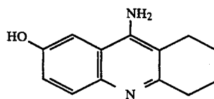
7-hydroxy-1,2,3,4-tetrahydro-5-aminoacridine
