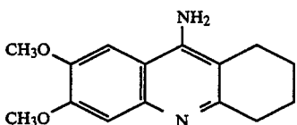
7,8-dimethoxy-1,2,3,4-tetrahydro-5-aminoacridine
