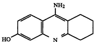
8-hydroxy-1,2,3,4-tetrahydro-5-aminoacridine
