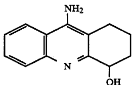
1-hydroxy-1,2,3,4-tetrahydro-5-aminoacridine
