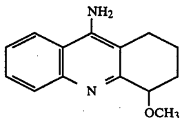
1-methoxy-1,2,3,4-tetrahydro-5-aminoacridine
