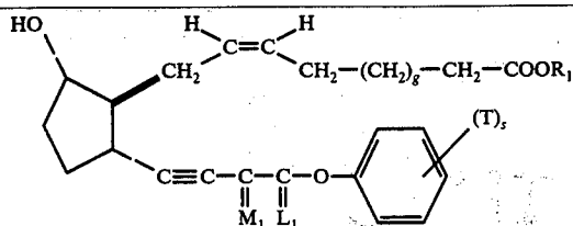
13,14-didehydro-11-deoxy-8 \beta ,12 \alpha -PGF 2 \alpha -type compounds
