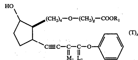
3-oxa-13,14-didehydro-11-deoxy-8 \beta ,12 \alpha -PGF 1 \alpha -type compounds
