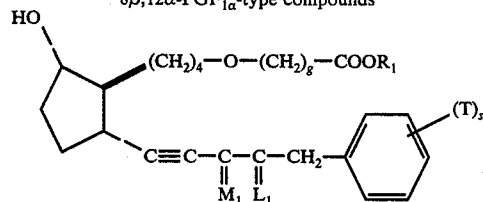
3-oxa-13,14-didehydro-18,19,20-trinor-11-deoxy-8 \beta ,12 \alpha -PGF 1 \alpha -type compounds
