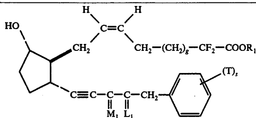
2,2-difluoro-13,14-didehydro-18,19,20-trinor-11-deoxy-8 \beta ,12 \alpha -PGF 2 \alpha -type compounds
