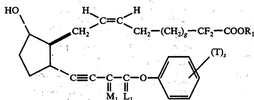
2,2-difluoro-13,14-didehydro-11-deoxy-8 \beta ,12 \alpha -PGF 2 \alpha -type compounds
