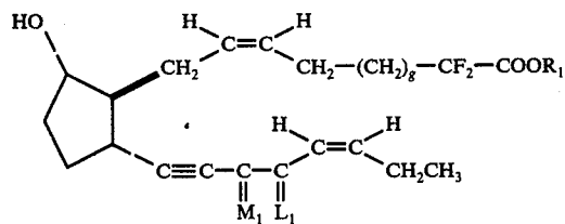
2,2-difluoro-13,14-didehydro-11-deoxy- 8 \beta ,12 \alpha -PGF _{3\alpha} -type compounds
