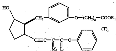
3,7-inter-m-phenylene-4,5,6-trinor-3-oxa-13,14-didehydro-11-deoxy-8 \beta ,12 \alpha -PGF 1 \alpha -type compounds
