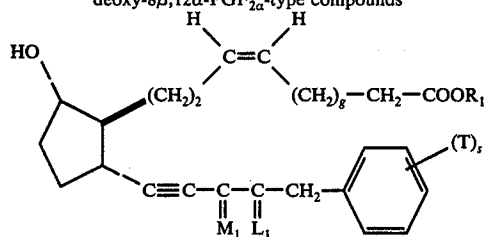
cis-4,5-didehydro-13,14-didehydro-18,19,20-trinor-11-deoxy-8 \beta ,12 \alpha -PGF 1 \alpha -type compounds
