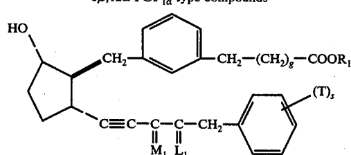
3,7-inter-m-phenylene-4,5,6,18,19,20-hexanor-13,14-didehydro-11-deoxy-8 \beta ,12 \alpha -PGF 1 \alpha -type compounds
