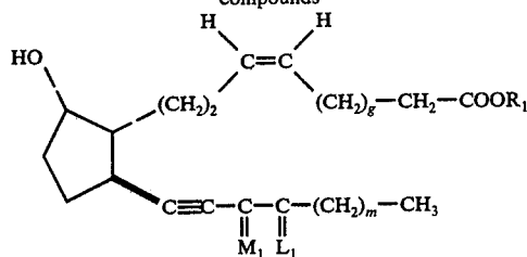
cis-4,5-didehydro-13,14-didehydro-11-deoxy-PGF 1α -type compounds
