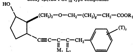
5-oxa-13,14-didehydro-18,19,20-trinor-11-deoxy-8 \beta ,12 \alpha -PGF 1 \alpha -type compounds
