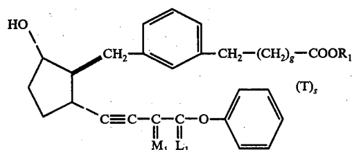
3,7-inter-m-phenylene-4,5,6-trinor-13,14-didehydro-11-deoxy-8 \beta ,12 \alpha -PGF 1 \alpha -type compounds
