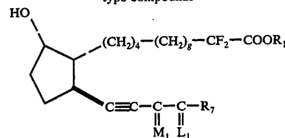
2,2-difluoro-13,14-didehydro-11-deoxy-PGF 1α -type compounds
