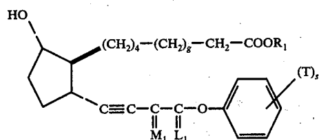
13,14-didehydro-11-deoxy-8 \beta ,12 \alpha -PGF 1 \alpha -type compounds
