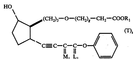
4-oxa-13,14-didehydro-11-deoxy-8 \beta ,12 \alpha -PGF 1 \alpha -type compounds
