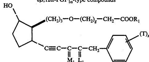
4-oxa-13,14-didehydro-18,19,20-trinor-11-deoxy-8 \beta ,12 \alpha -PGF 1 \alpha -type compounds
