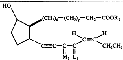
13,14-didehydro-cis-17,18-didehydro-11-deoxy- 8 \beta ,12 \alpha -PGF _{1\alpha} -type compounds
