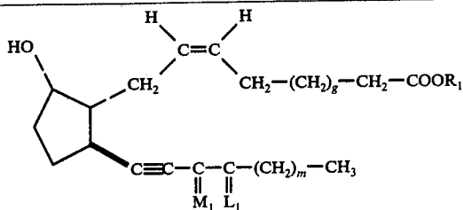
13,14-didehydro-11-deoxy-PGF 2α -type compounds
