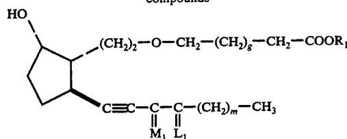
5-oxa-13,14-didehydro-11-deoxy-PGF 1α -type compounds
