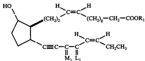
cis-4,5,17,18-tetradecahydro-13,14-didehydro-11- deoxy-8 \beta ,12 \alpha -PGF _{1\alpha} -type compounds
