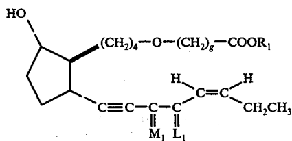
3-oxa-13,14-didehydro-cis-17,18-didehydro-11- deoxy-8 \beta ,12 \alpha -PGF _{1\alpha} -type compounds
