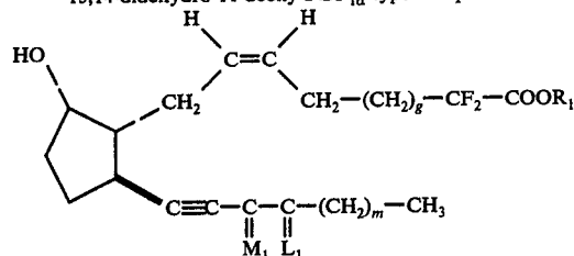
2,2-difluoro-13,14-didehydro-11-deoxy-PGF 2α -type compounds
