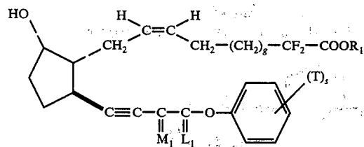
2,2-difluoro-13,14-didehydro-11-deoxy-PGF 2α -type compounds
