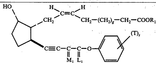
13,14-didehydro-11-deoxy-PGF 2α -type compounds
