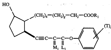
13,14-didehydro-11-deoxy-PGF 1α -type compounds
