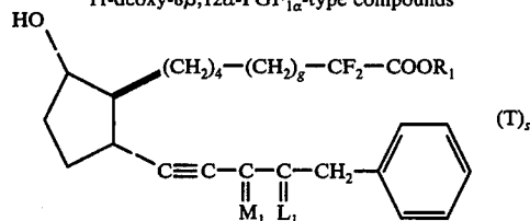
2,2-difluoro-13,14-didehydro-18,19,20-trinor-11-deoxy-8 \beta ,12 \alpha -PGF 1 \alpha -type compounds
