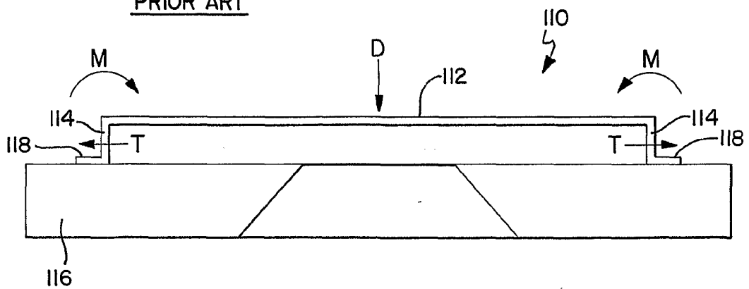
FIG. 12 PRIOR ART
