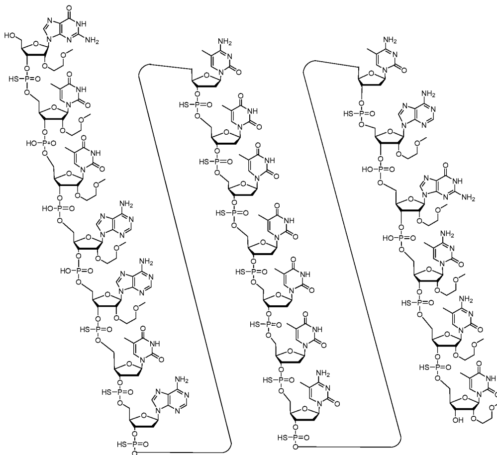
Structure 5. Compound No. 1102130
