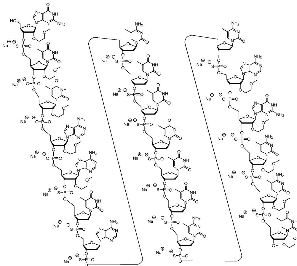
Structure 6. The sodium salt of Compound No. 1102130
