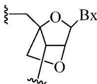
LNA ( \beta\text{-D} -configuration) bridge = 4'- \text{CH}_2\text{-O-2'}
