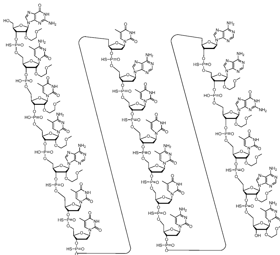
Structure 1. Compound No. 1100673
