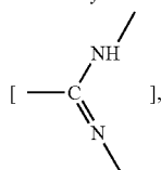
nitrilomethylenethios
