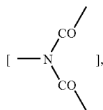
nitrilomethyleneoxys
