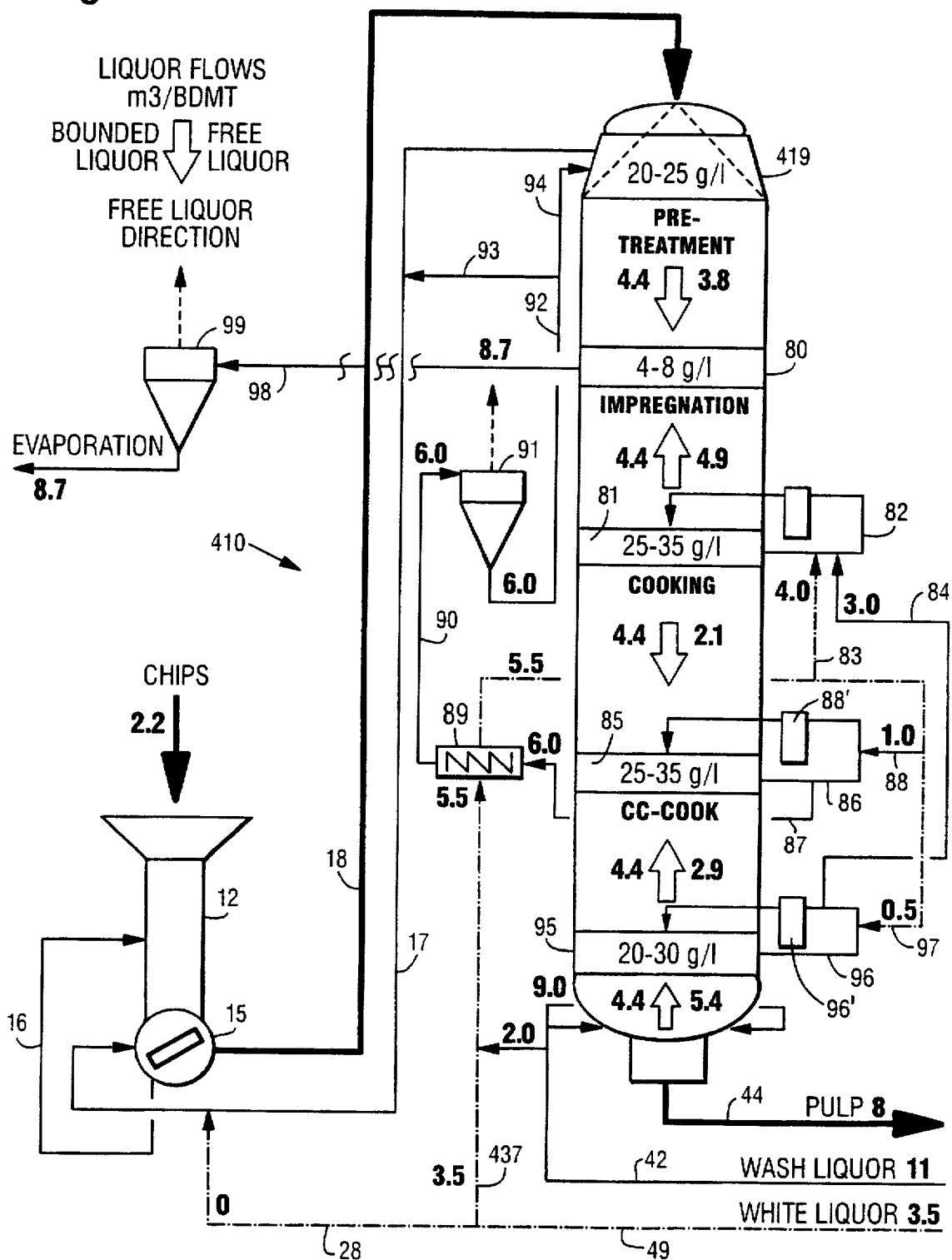
Fig. 10 LO-SOLIDS + COOKING LIQUOR RE-CIRCULATION
