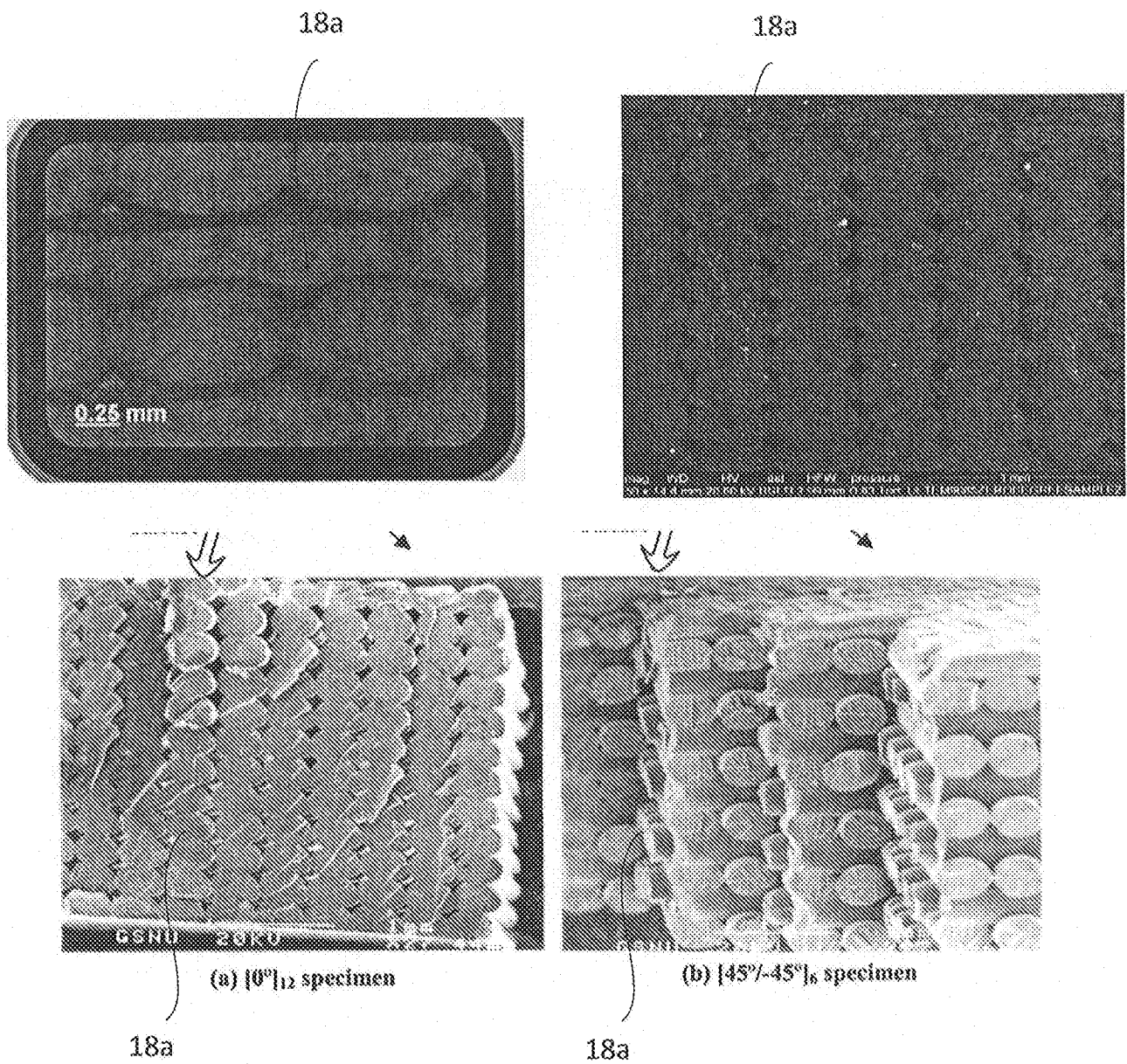
FIG. 1D FFF CROSS SECTIONS
