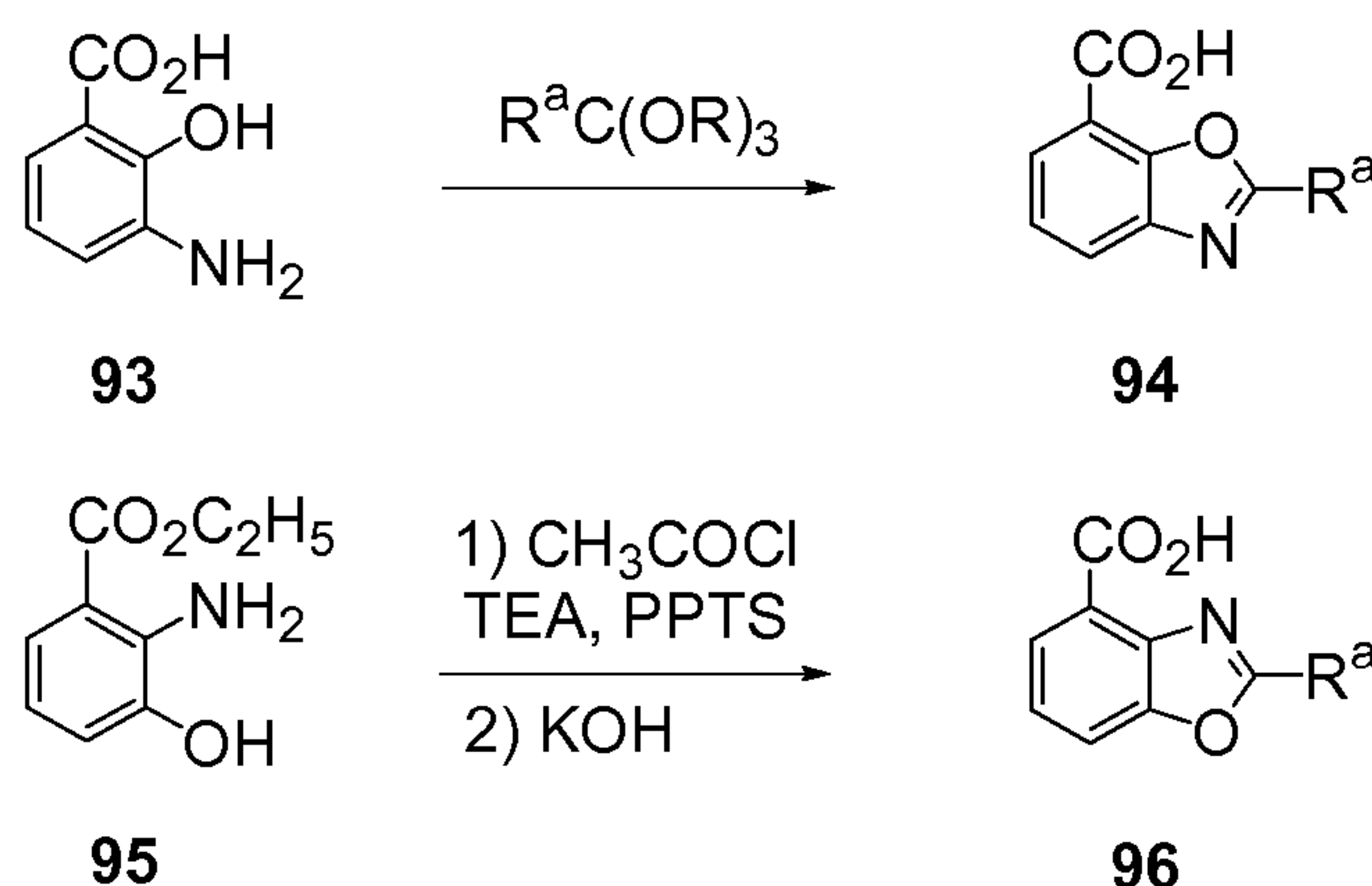
Scheme 13: Synthesis of benzoxazole-carboxylic acid derivatives wherein R is methyl or ethyl and R^a is hydrogen or methyl
