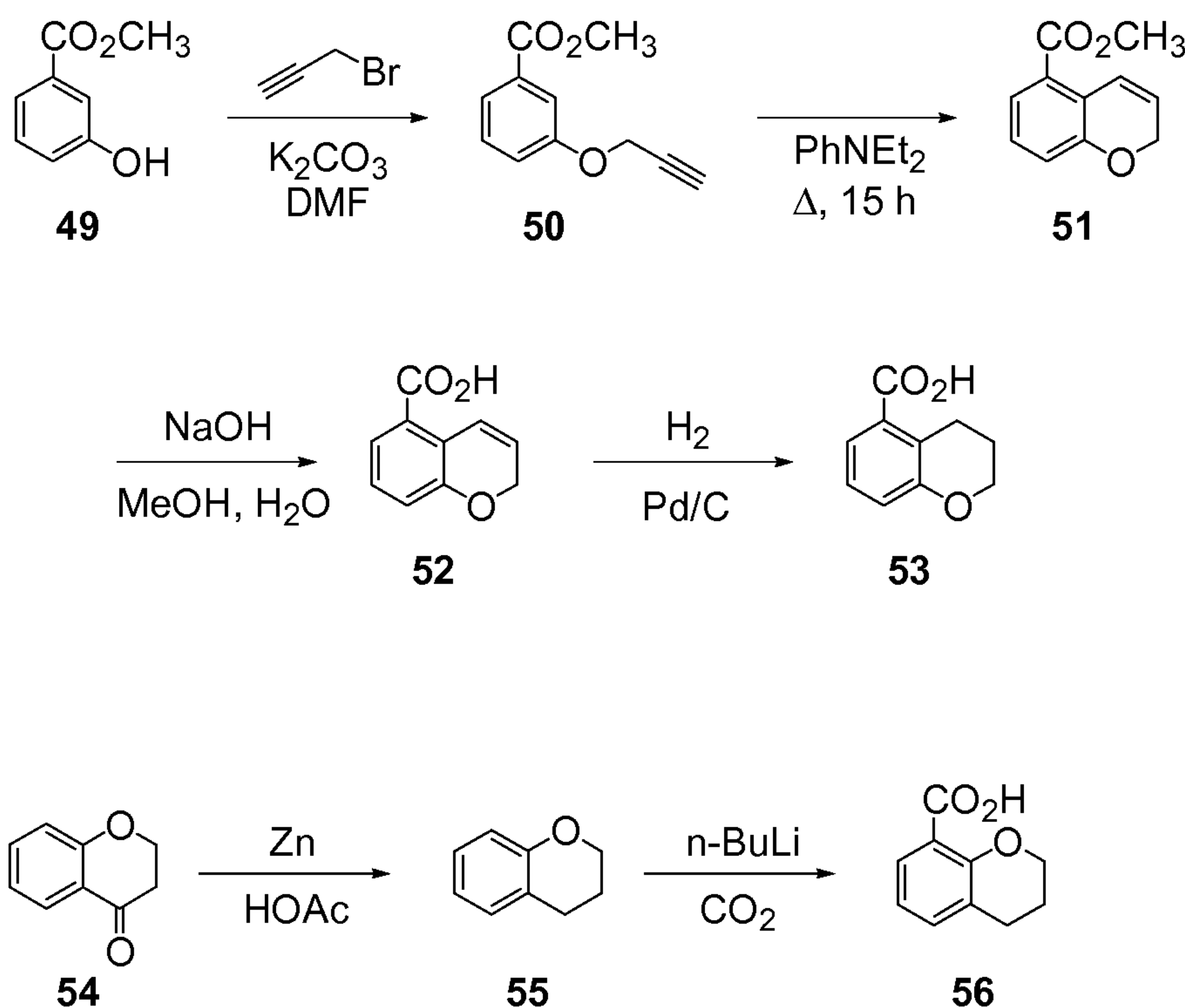
Scheme 9: Synthesis of chroman-carboxylic acid derivatives
