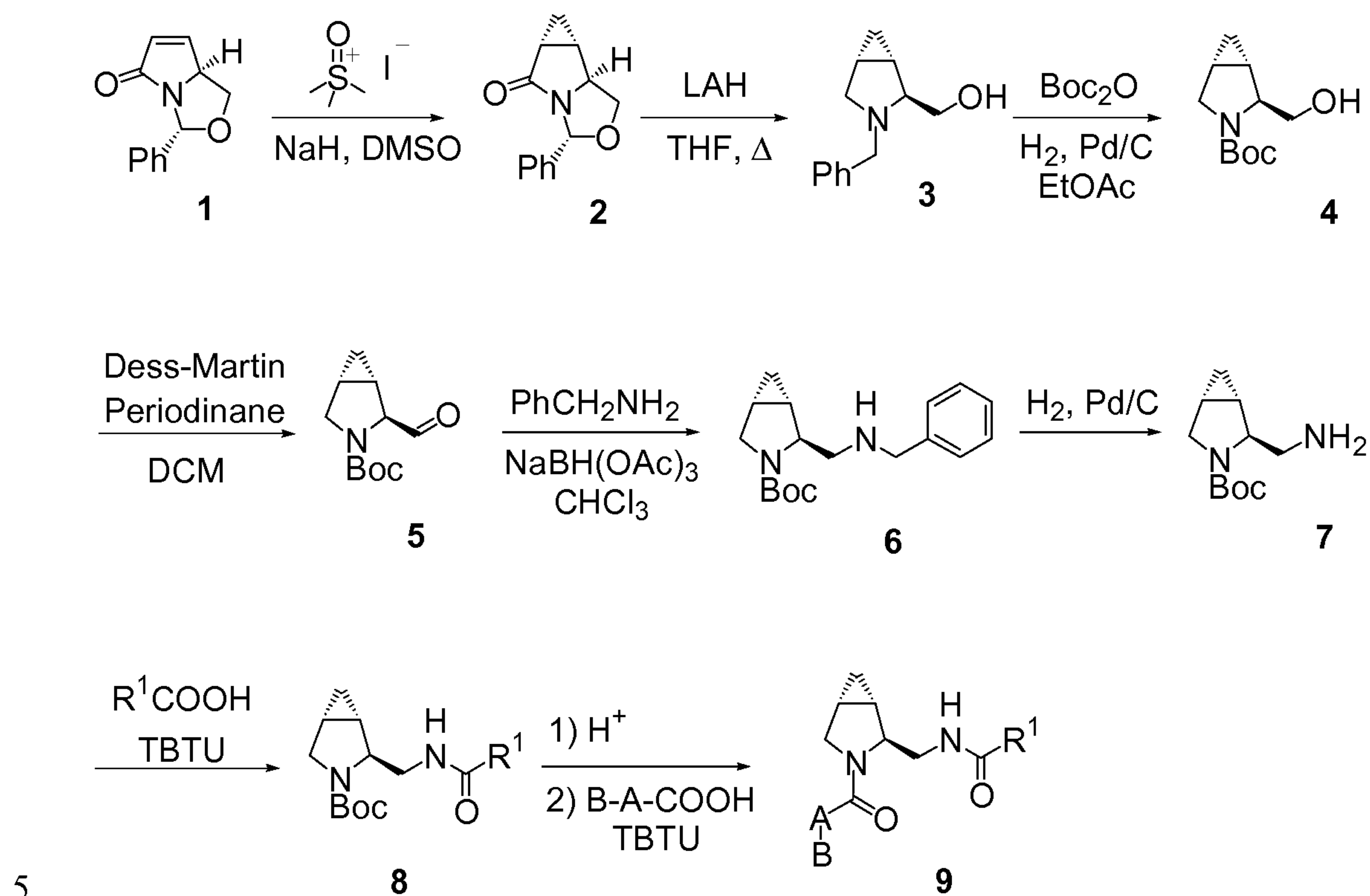
Scheme 1: Synthesis of compounds of formula (I), wherein n represents 1
