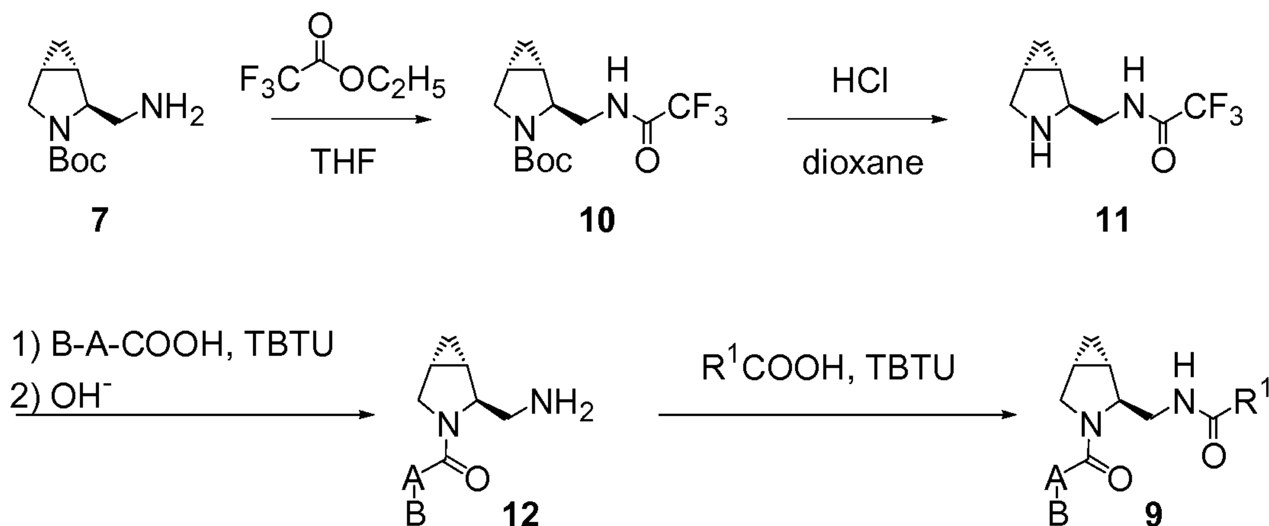
Scheme 2: Alternative synthesis of compounds of formula (I), wherein n represents 1
