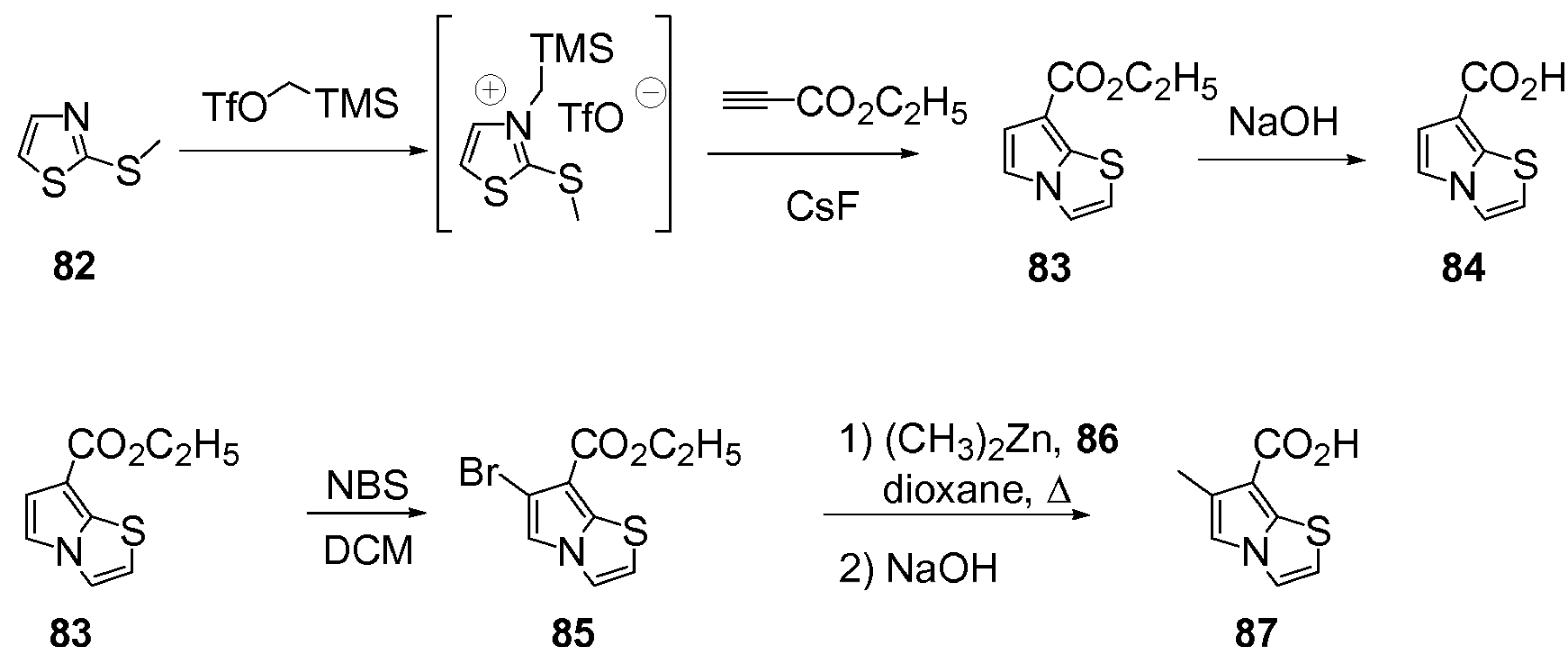
Scheme 11 : Synthesis of pyrrolo[2,1-b]thiazole-carboxylic acid derivatives
