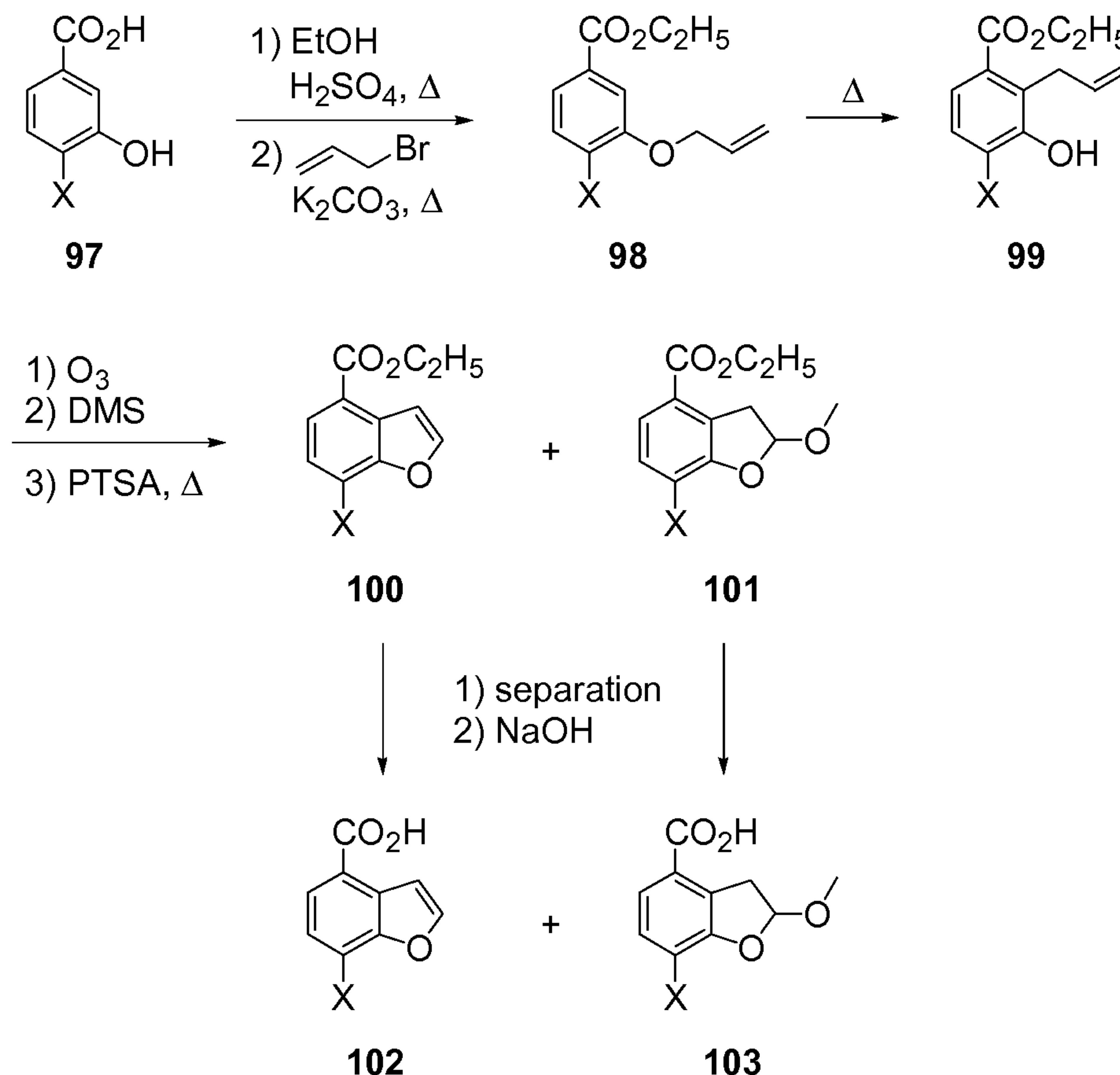
Scheme 14 : Synthesis of benzofuran-carboxylic acid derivatives wherein X is fluorine or chlorine
