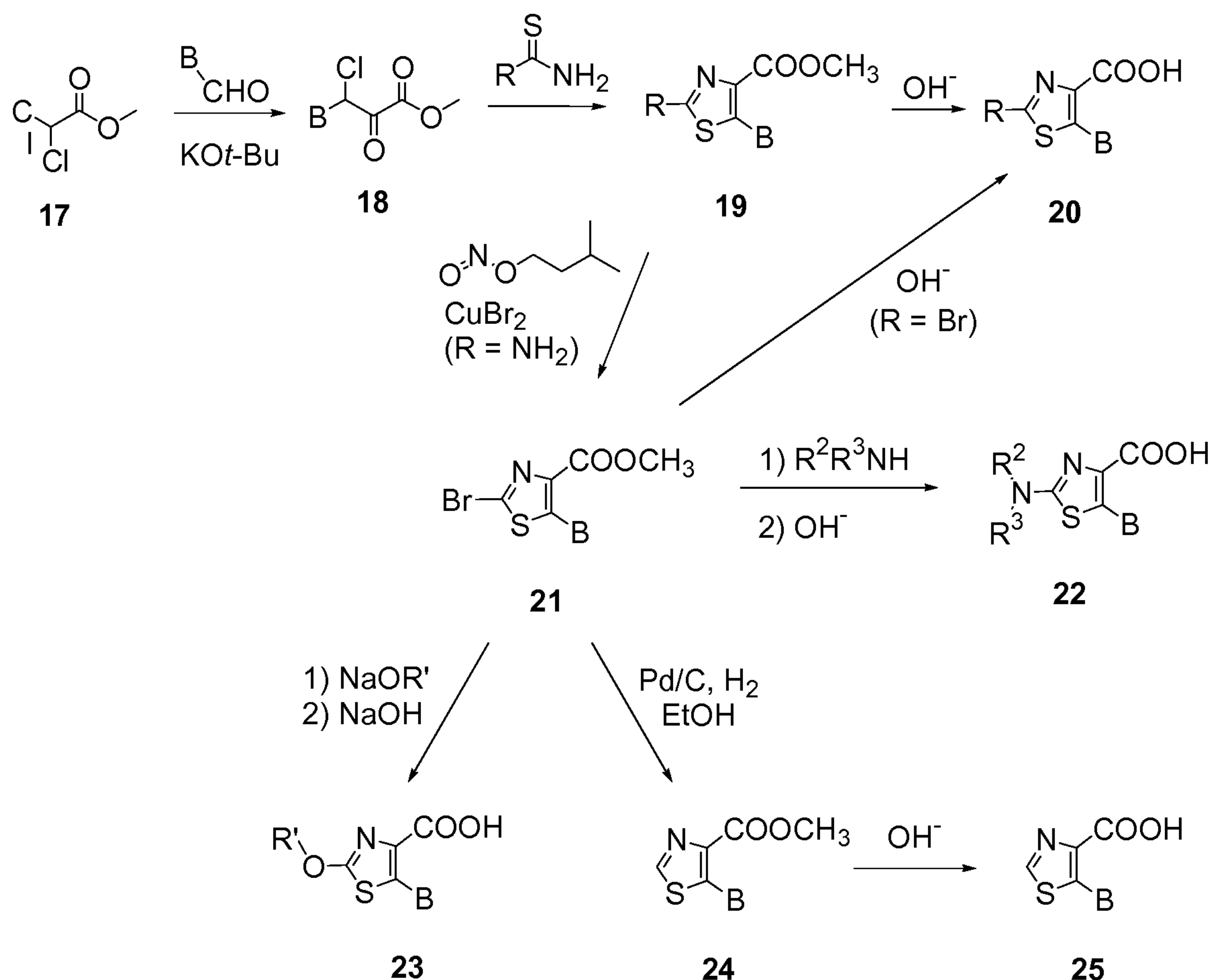
Scheme 5: Synthesis of thiazole-4-carboxylic acid derivatives, wherein
