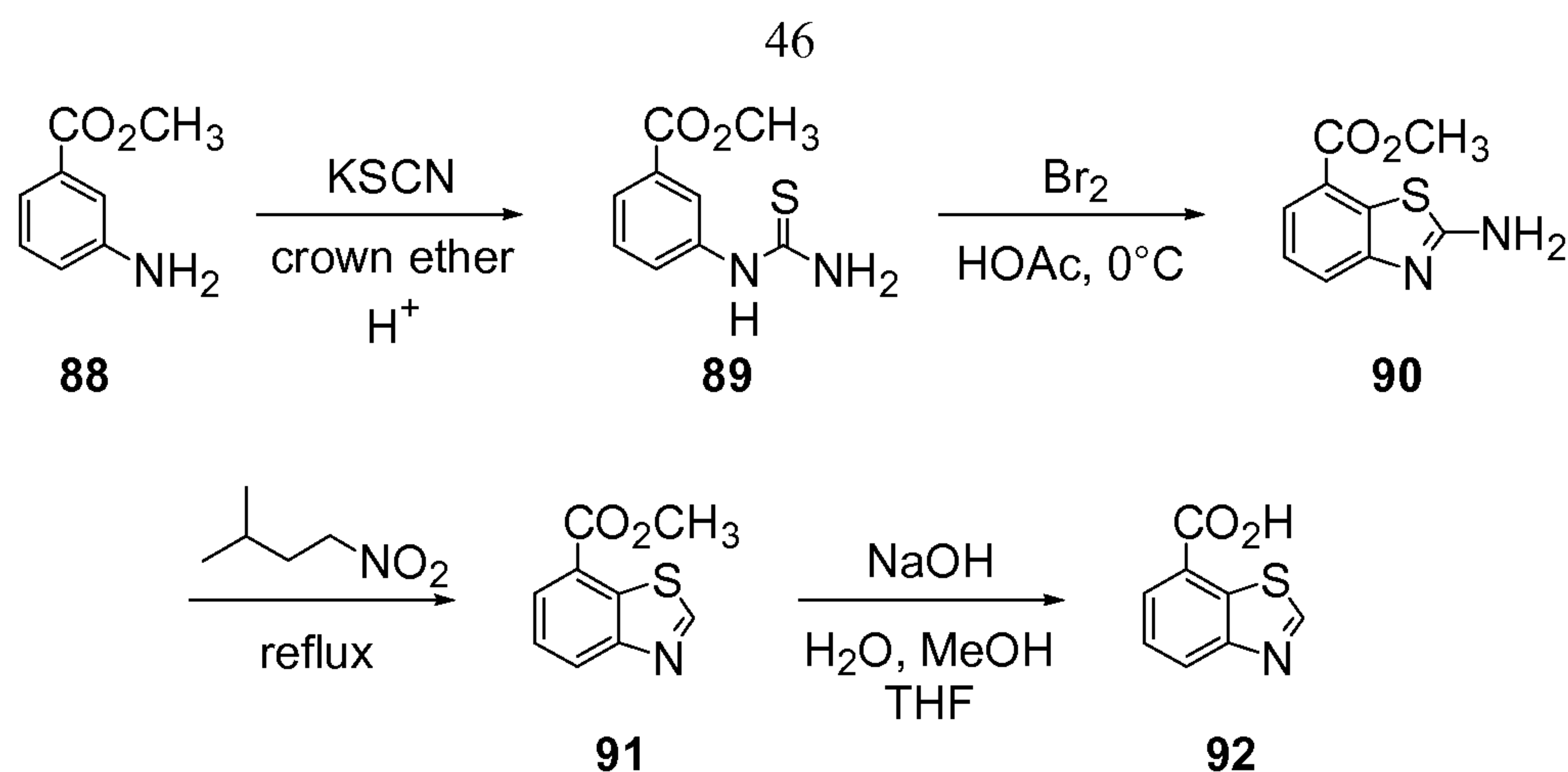
Scheme 12: Synthesis of benzothiazole-carboxylic acid derivatives
