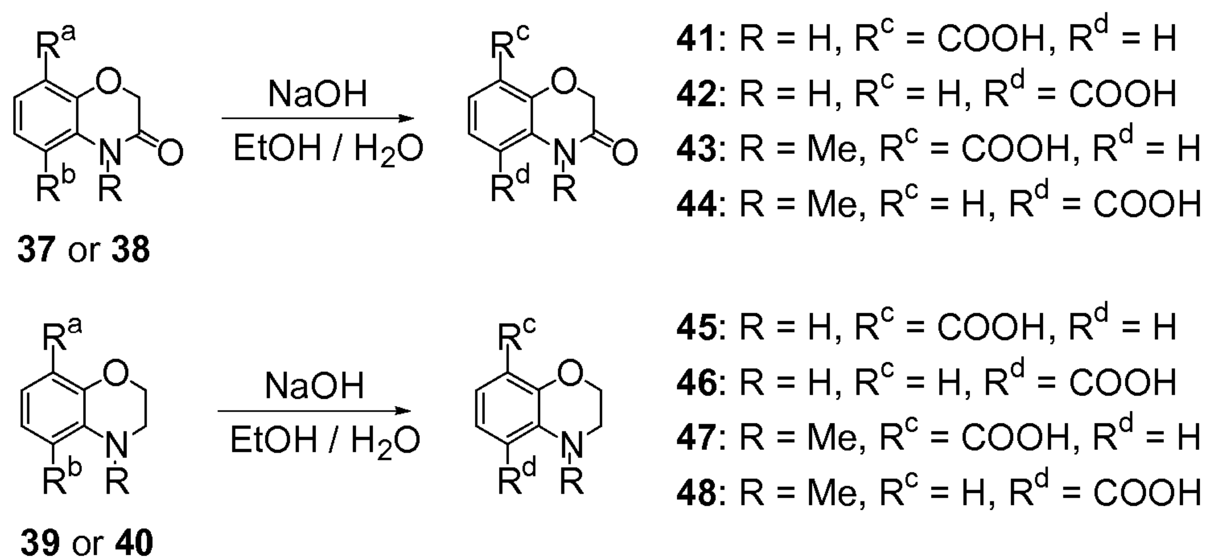
Scheme 8 : Synthesis of benzo[1,4]oxazine-carboxylic acid derivatives
