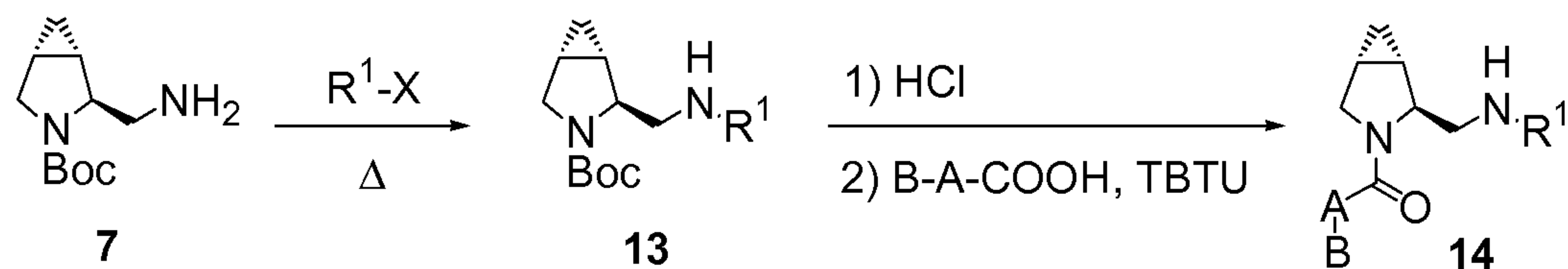
Scheme 3: Alternative synthesis of compounds of formula (I), wherein n represents 0; X represents Cl, Br, or OTf.
