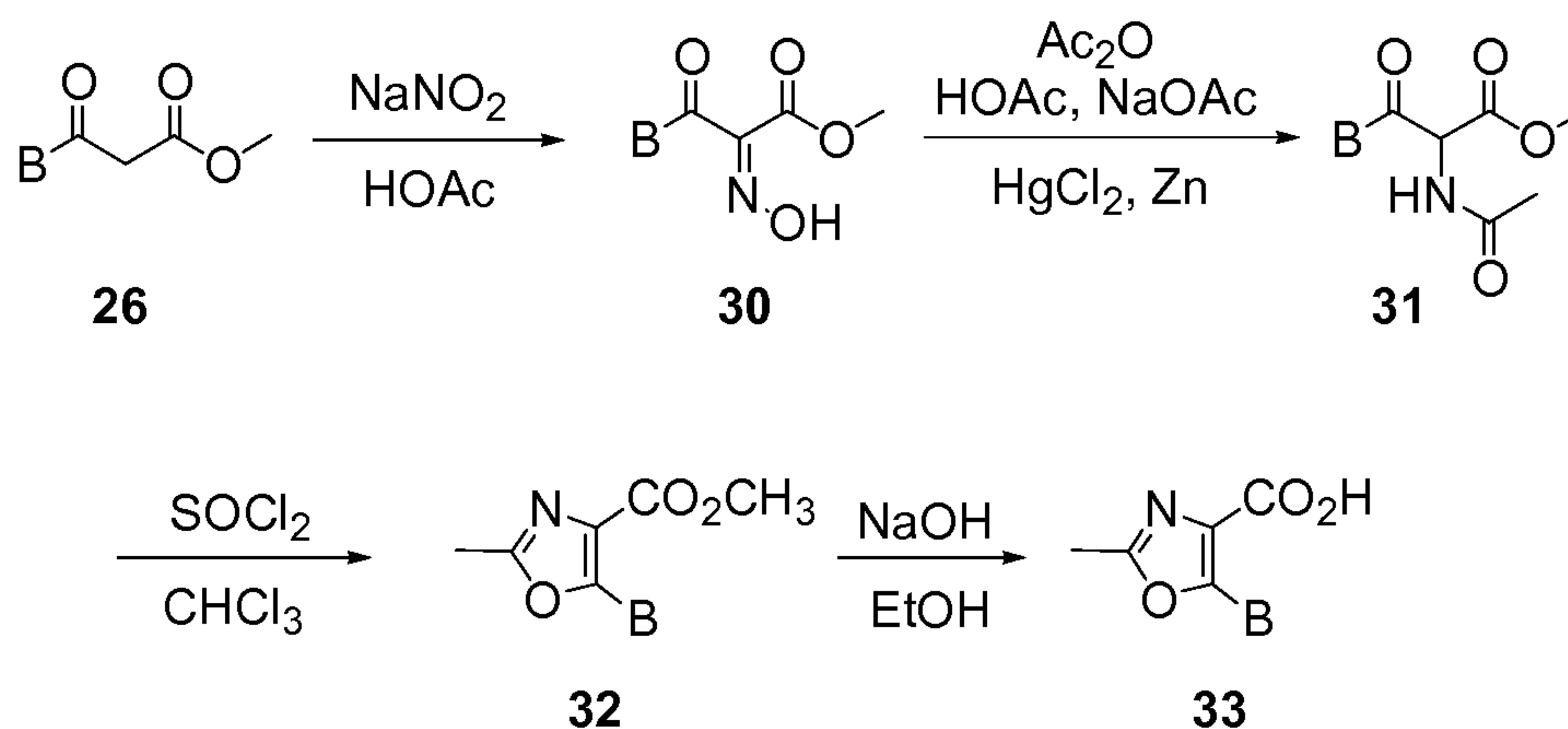
Scheme 7: Synthesis of oxazole-4-carboxylic acid derivatives
