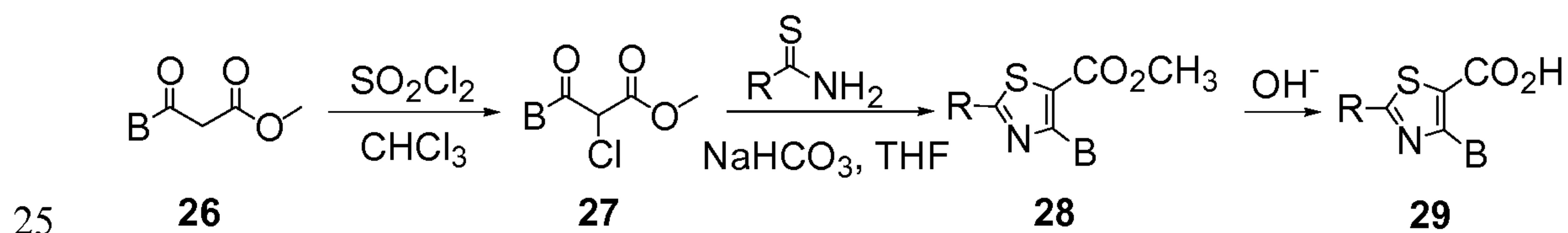
Scheme 6 : Synthesis of thiazole-5-carboxylic acid derivatives, wherein R is (C 1-4 )alkyl or (C 3-6 )cycloalkyl
