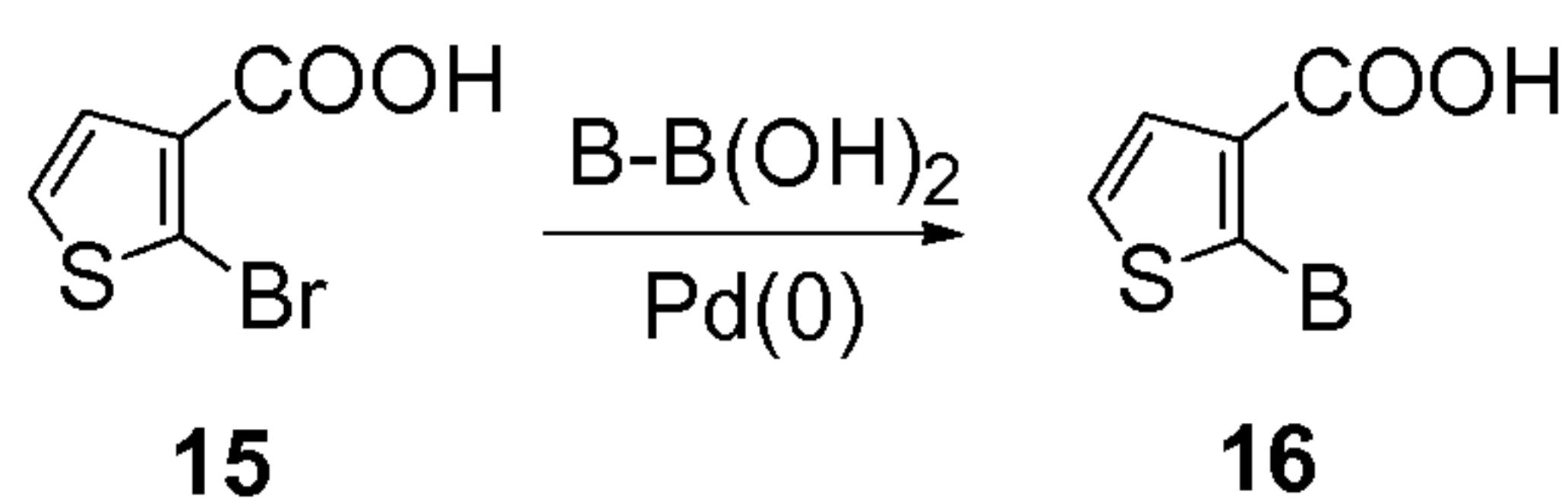
Scheme 4: Synthesis of thiophene-3-carboxylic acid derivatives
