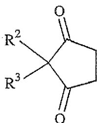
Formula VI
