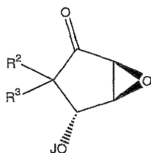
Formula IX
