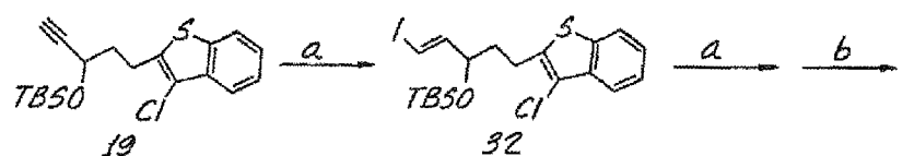
Fig. 7 (SCHEME 7)
