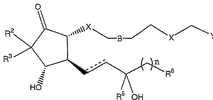
Formula V
