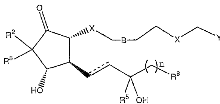
Formula V
