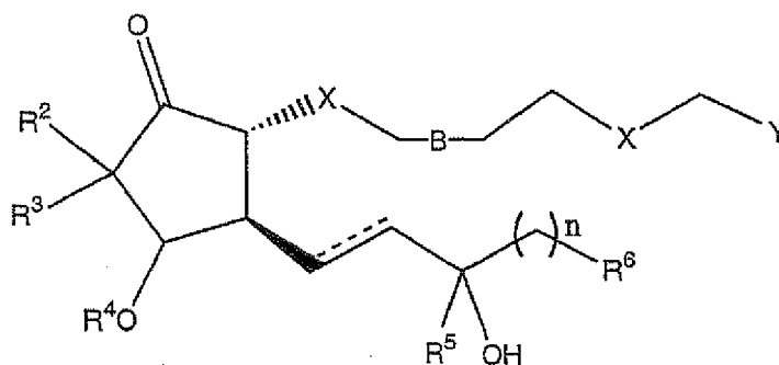
Formula I
