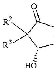
Formula VII
