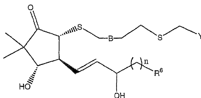
Formula III
