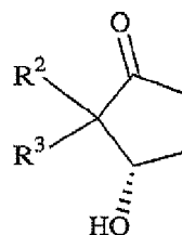
Formula VII
