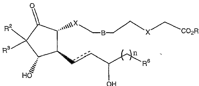
Formula VIII
