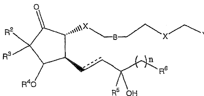
Formula I
