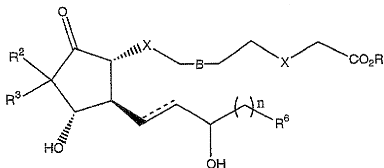
Formula VIII
