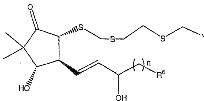
Formula III
