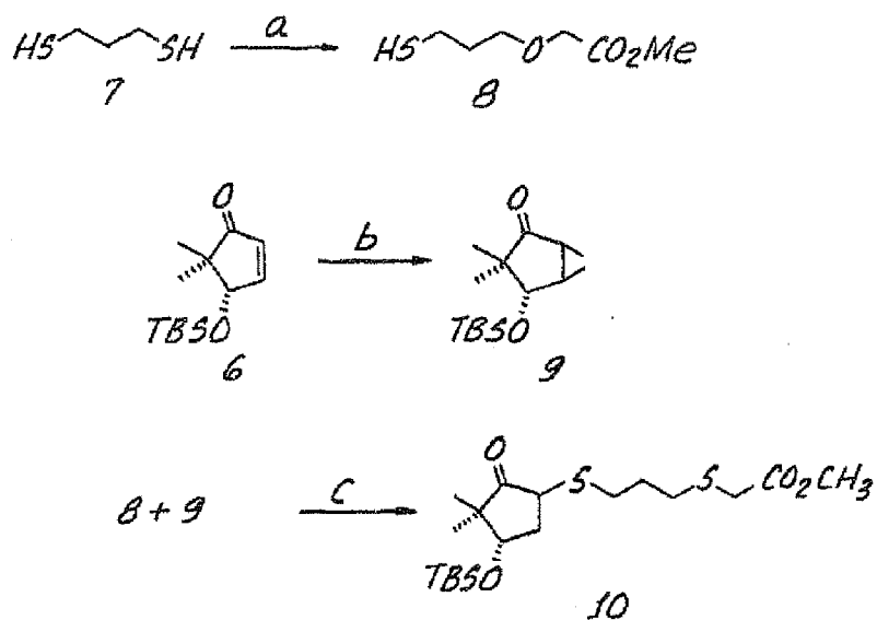
Fig. 3. (SCHEME 3)
