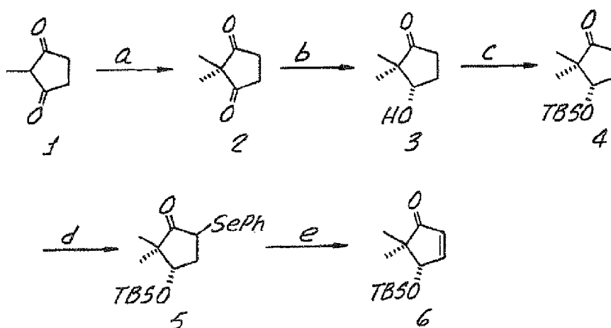
FIG. 2. (SCHEME 2)
