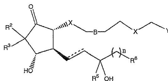
Formula V
