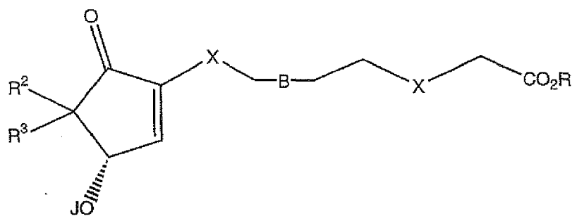
Formula XI
