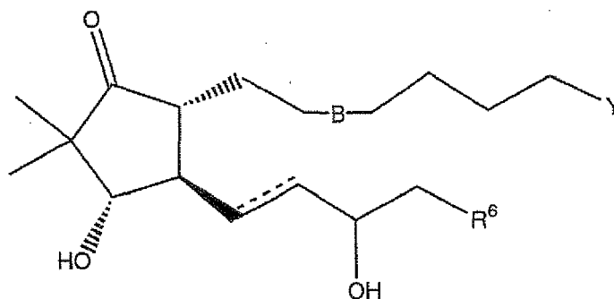
Formula XIII
