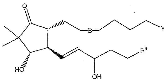
Formula IV
