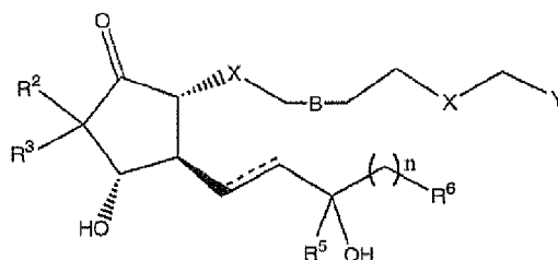
Formula V
