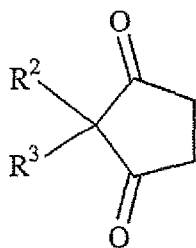
Formula VI
