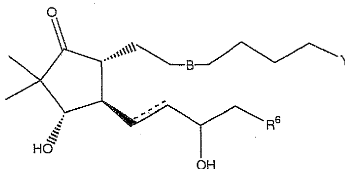
Formula XIII
