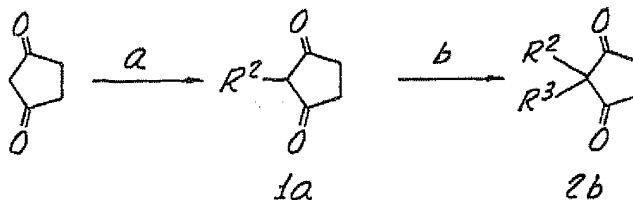
EQUATION 2
