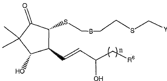
Formula III
