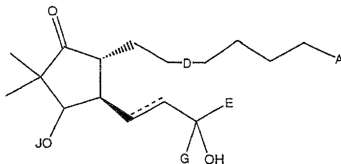
Formula II
