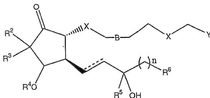
Formula I
