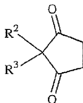
Formula VI
