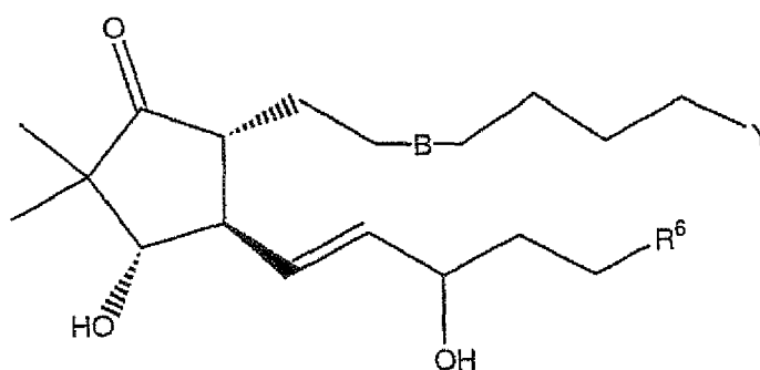
Formula IV
