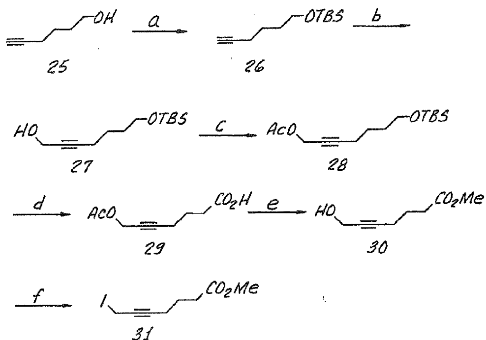
Fig. 6. (SCHEME 6)
