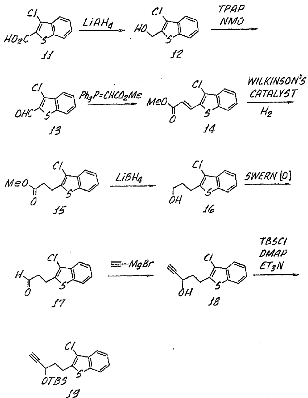
Fig. 4. (SCHEME 4)
