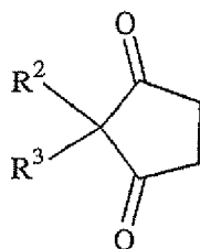
Formula VI
