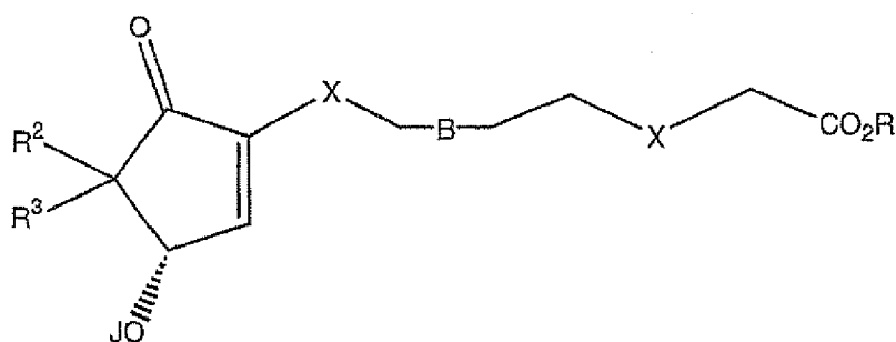
Formula XI
