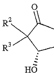
Formula VII
