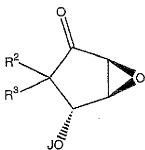
Formula IX
