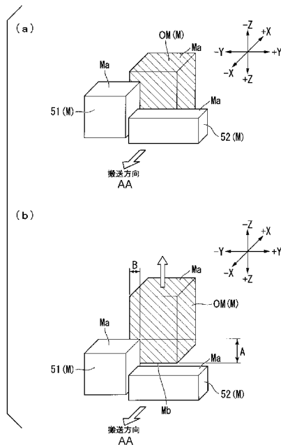
FIG. 9: AA Conveyance direction
