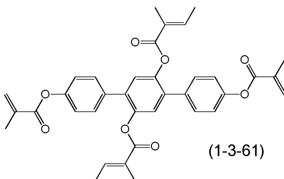
Compound (1-3-61)
