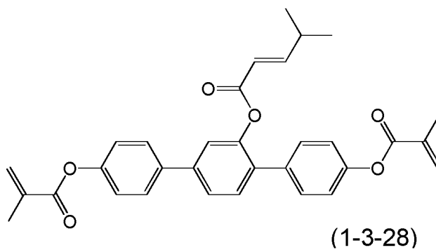
Compound (1-3-28)
