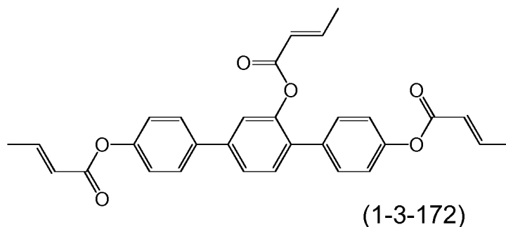
Compound (1-3-172)
