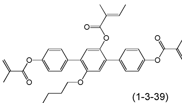
Compound (1-3-39)
