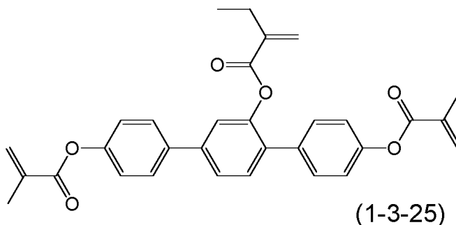
Compound (1-3-25)
