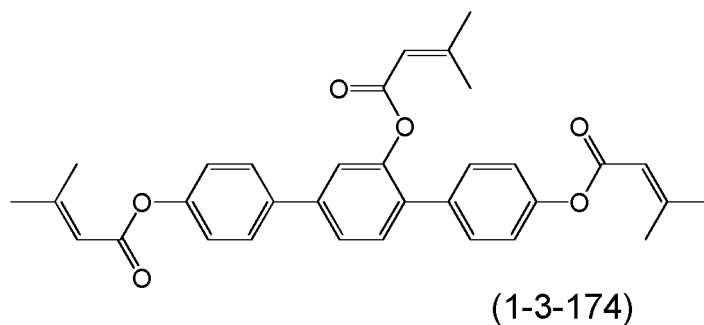
Compound (1-3-174)
