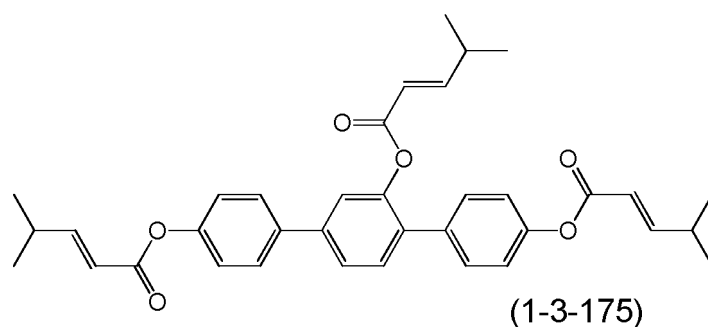
Compound (1-3-175)
