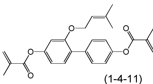
Compound (1-4-11)
