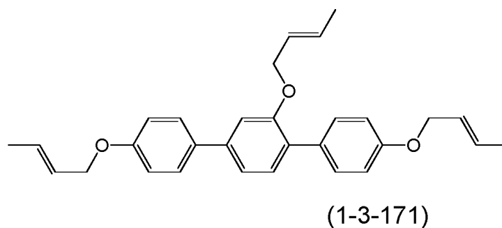
Compound (1-3-171)
