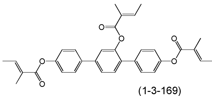
Compound (1-3-169)
