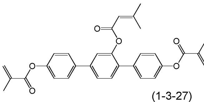
Compound (1-3-27)
