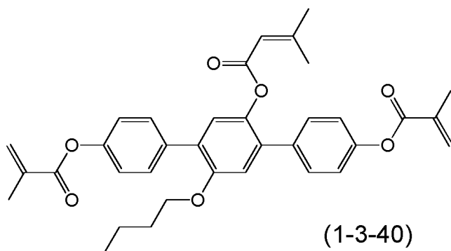
Compound (1-3-40)
