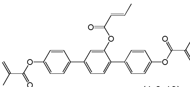
(1-3-19)
