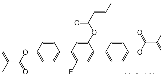
(1-3-18)
