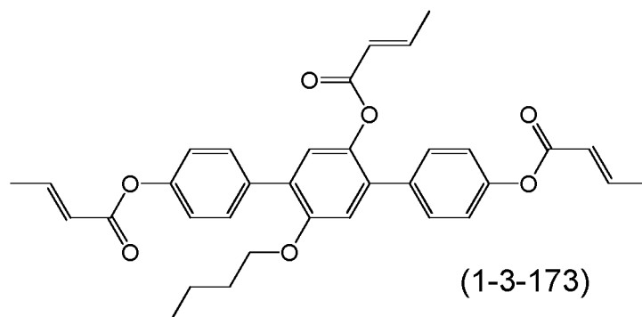
Compound (1-3-173)
