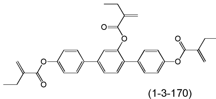
Compound (1-3-170)
