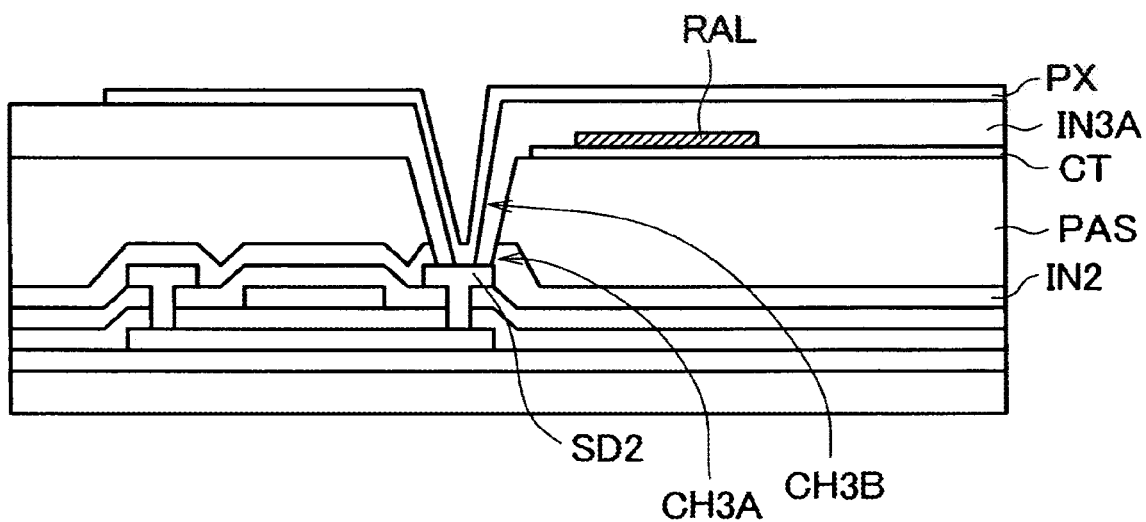
FIG. 7 RELATED ART
