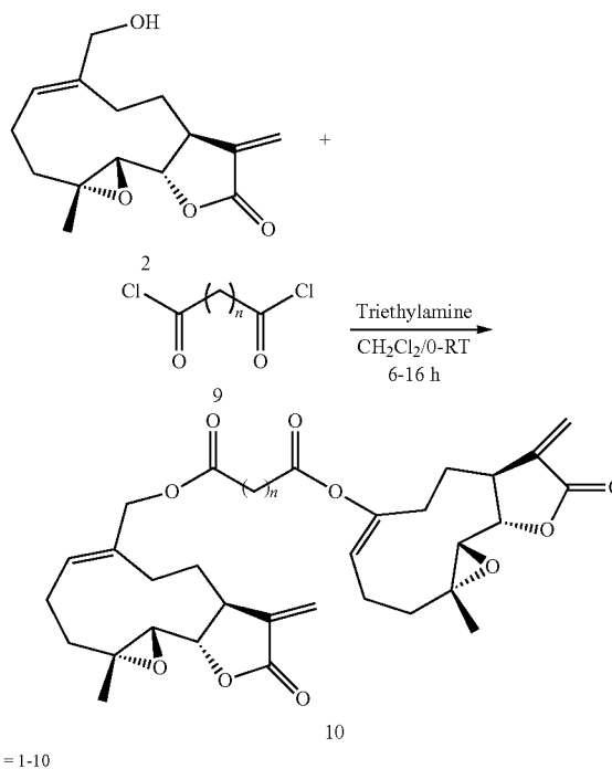
Scheme 3: Synthesis of ester dimers of MMB
