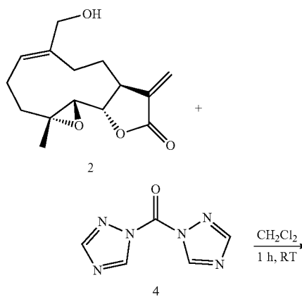
Scheme 1: Synthesis of carbamate and carbonate dimers of MMB
