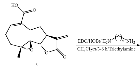
Scheme 5: synthesis of carboxamide dimers of melampomagnolic acid
