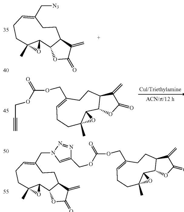
Scheme 6. Synthesis of triazole carbonate dimer of MMB
