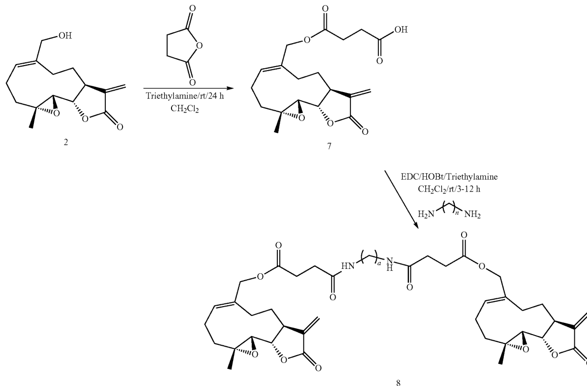
Scheme 2: Synthesis of succinic amide dimers of MMB
