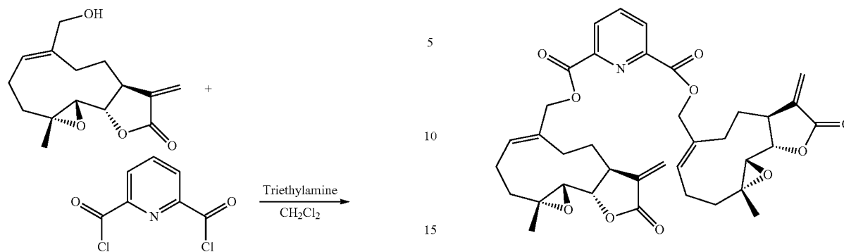
Scheme 7. Synthesis of pyridine 2, 6 diester dimer of MMB
