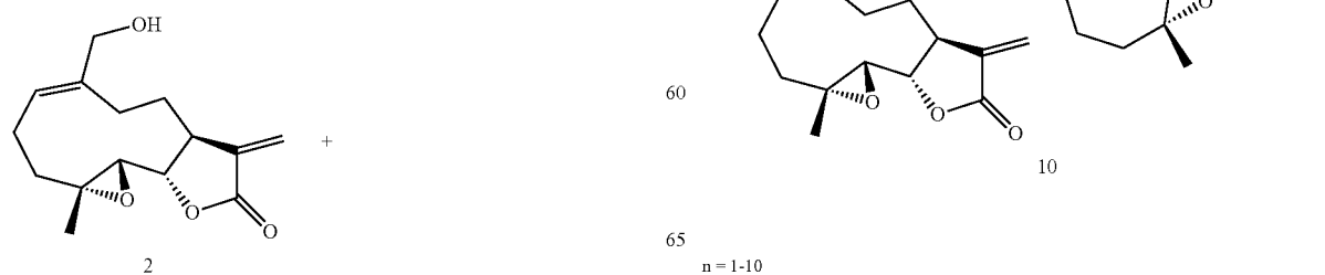
Scheme 3. Synthesis of ester derivatives of MMB
