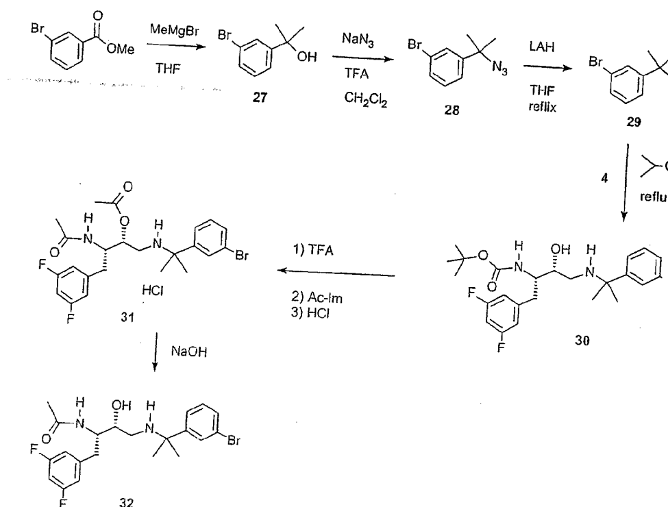
Scheme 8
