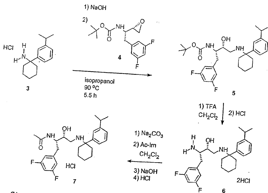
Scheme 2
