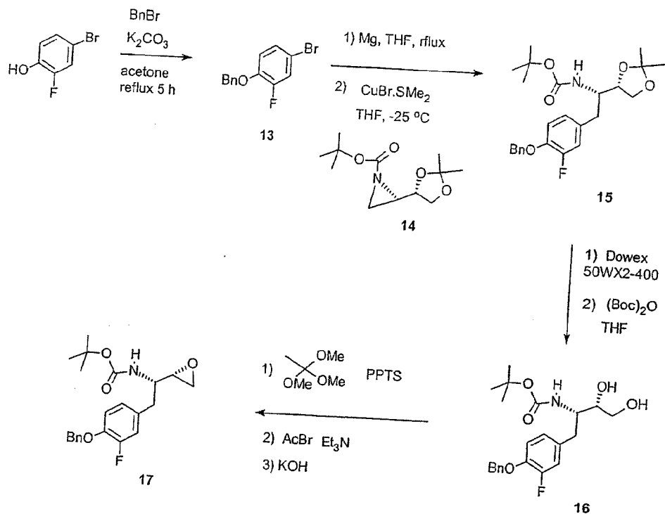
Scheme 4
