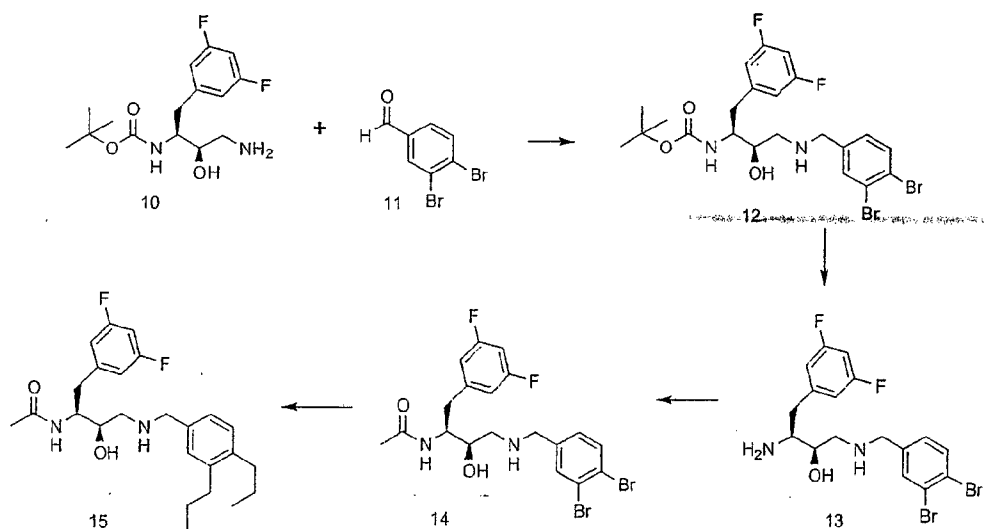
Scheme 118
