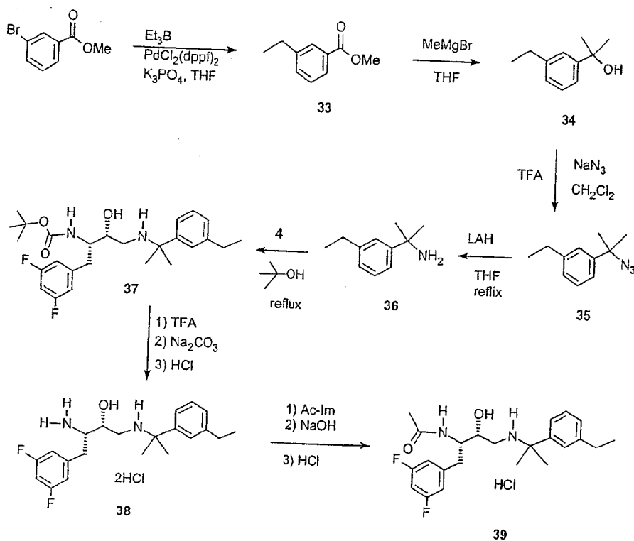
Scheme 9
