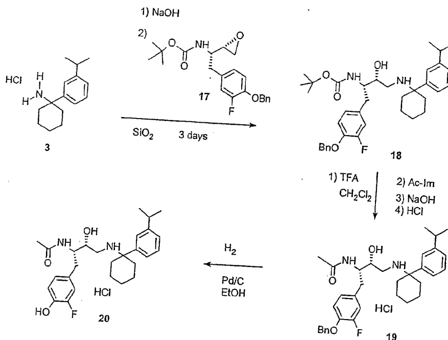
Scheme 5
