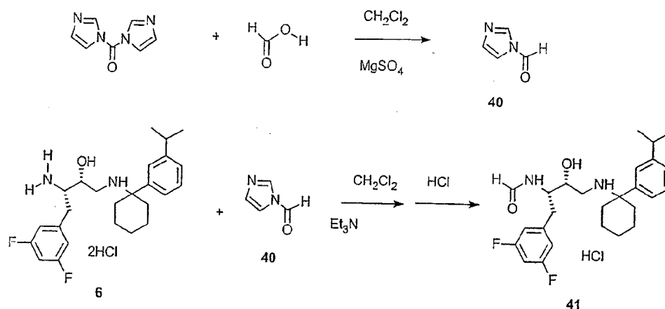
Scheme 10
