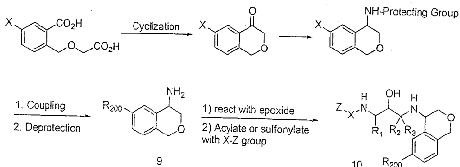
Scheme VIII
