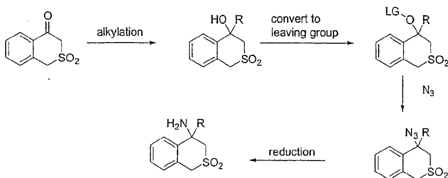
Scheme III
