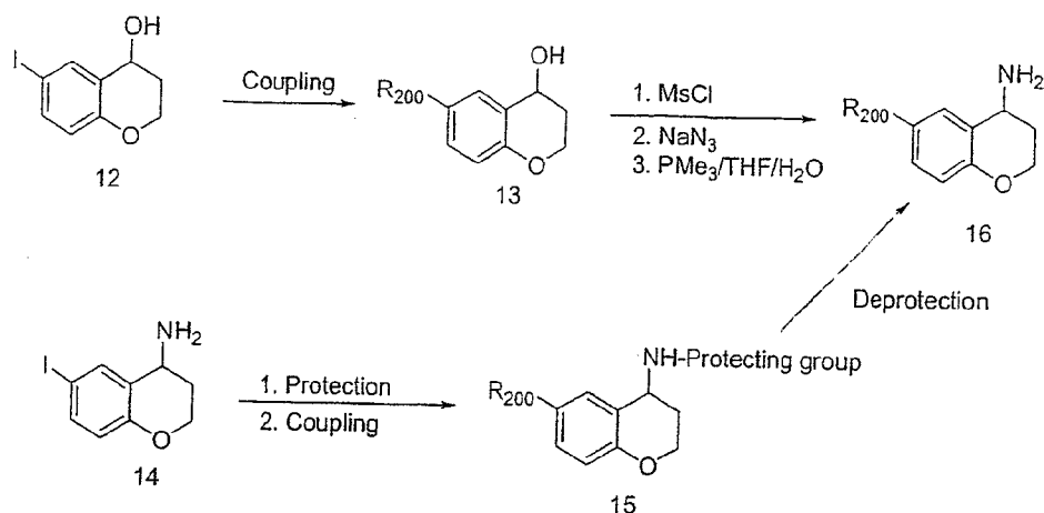
Scheme VII
