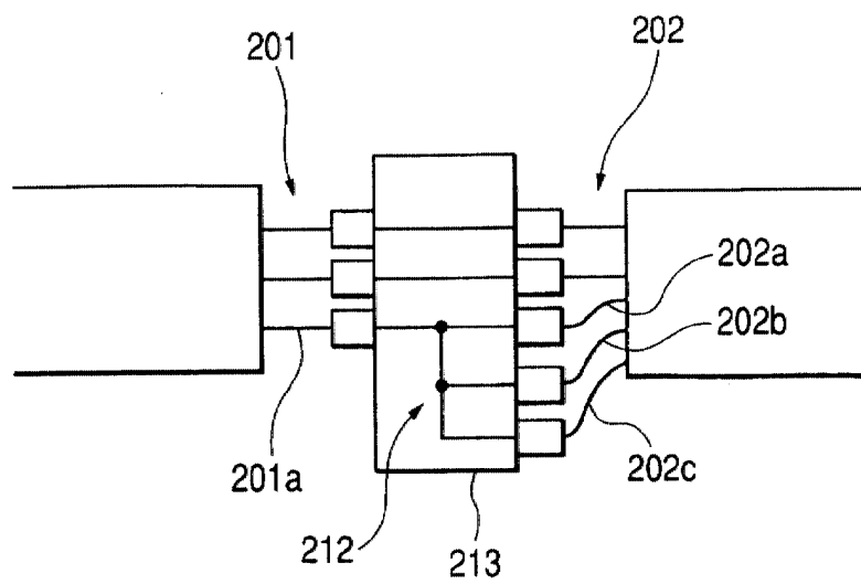
FIG. 27 PRIOR ART
