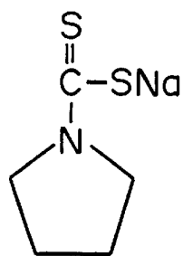
Sodium pyrrolidine- N - carbodithioate
