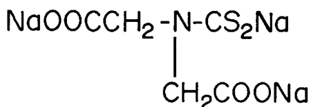
Trisodium N , N -di(carboxymethyl)- N - carbodithioate (or Iminodiacetic acid dithiocarbamate, trisodium)
