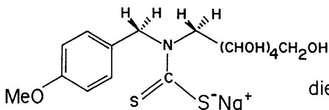
Sodium N -(4-methoxybenzyl) -D-glucamine- N - carbodithioate
