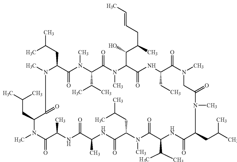
Formula I
