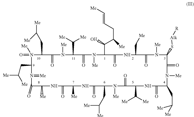
Formula III
