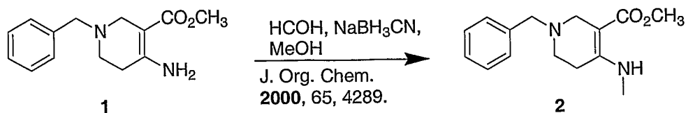
Scheme 3.
