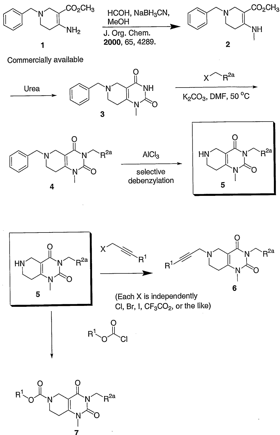
Scheme 2.
