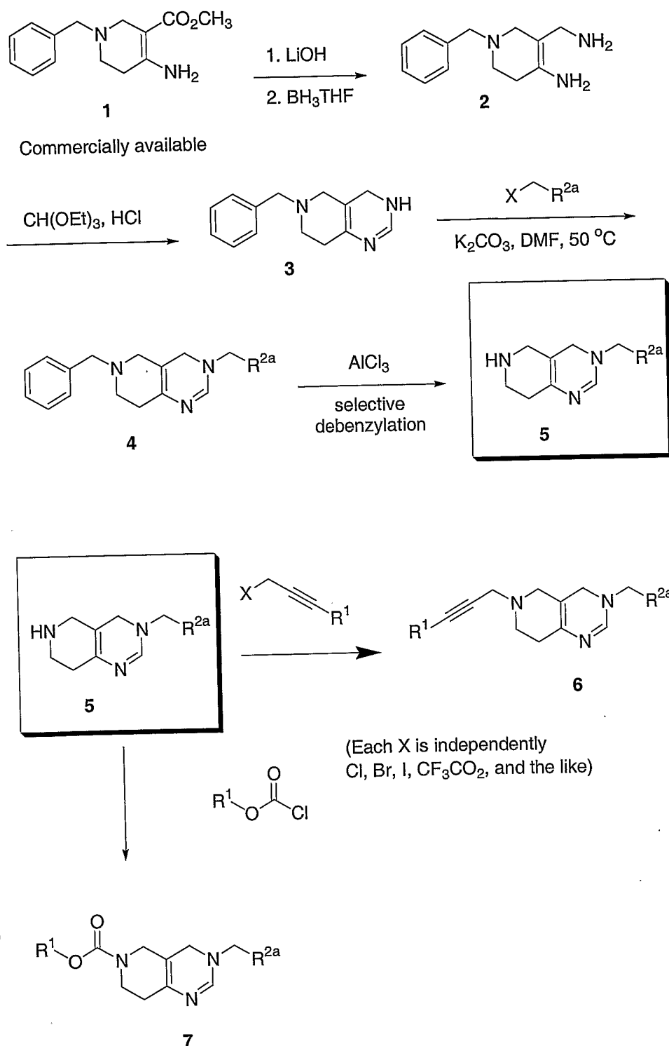
Scheme 4.
